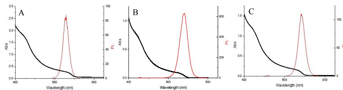
Figure 2S: CsPbI 3 absorption and PL at (A) 1 seconds growth duration, (B) 20 seconds growth duration and (C) 40 seconds growth duration.
