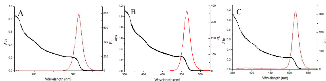
Figure 1S: CsPbBr 3 absorption and PL at (A) 1 seconds growth duration, (B) 20 seconds growth duration and (C) 40 seconds growth duration.
