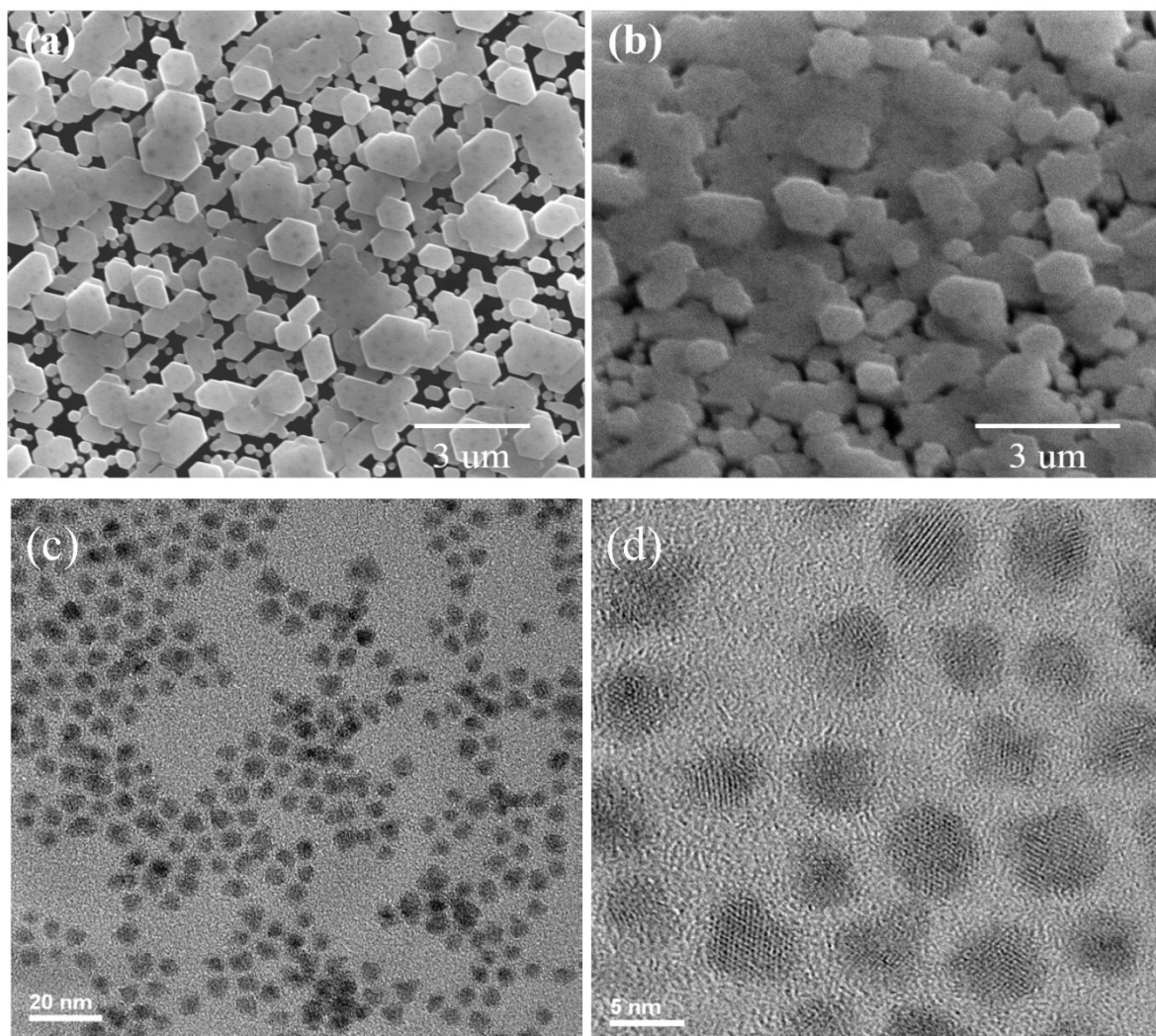
Figure S1. Top view SEM images of anneal ZnO Nanorods (a) before QDs coating and (b) after QDs coating. (c) TEM images of CdSe quantum dots (d) magnified view of image (c).
