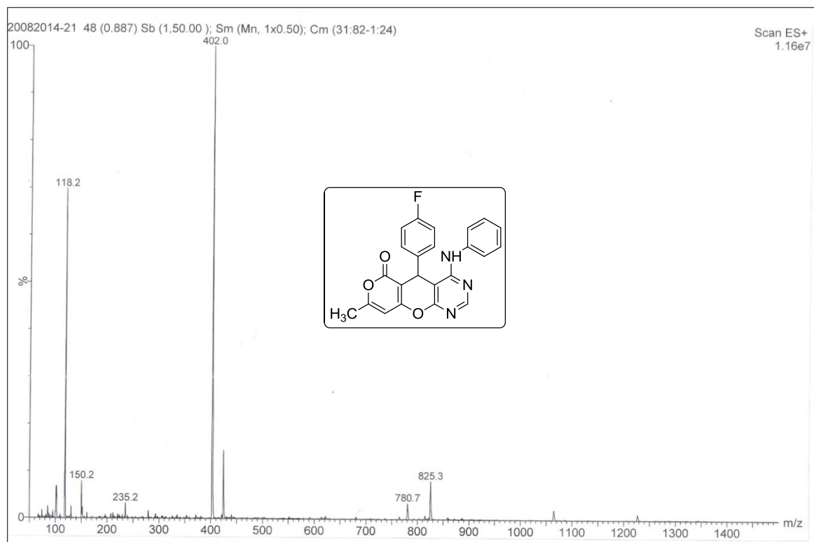
Mass Spectrum of compound 4e
