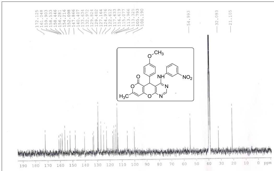
13 C NMR Spectrum of compound 4k
