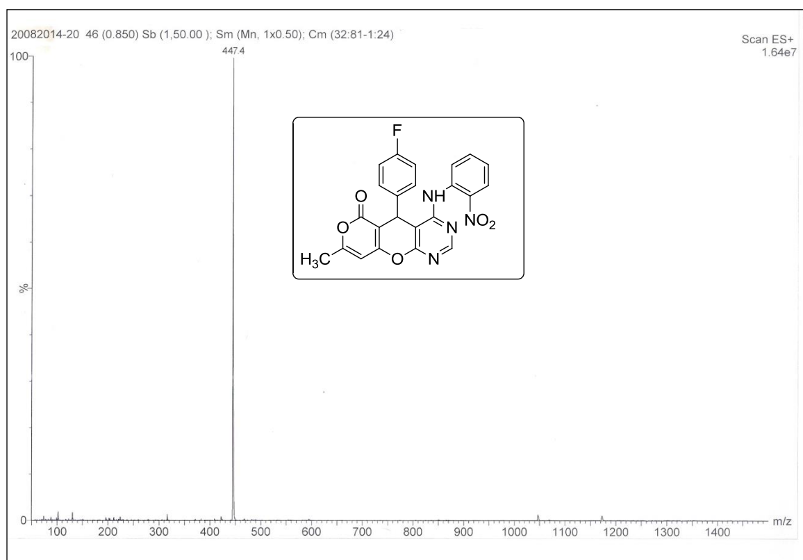
Mass Spectrum of compound 4g
