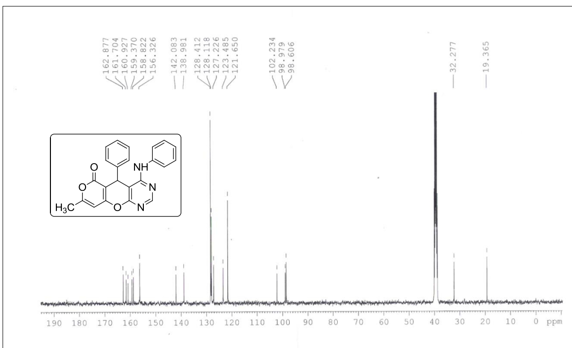
13 C NMR Spectrum of compound 4a
