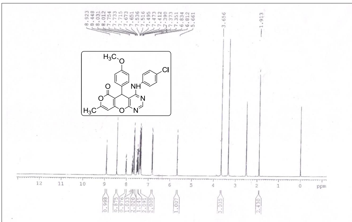
1 H NMR Spectrum of compound 4j
