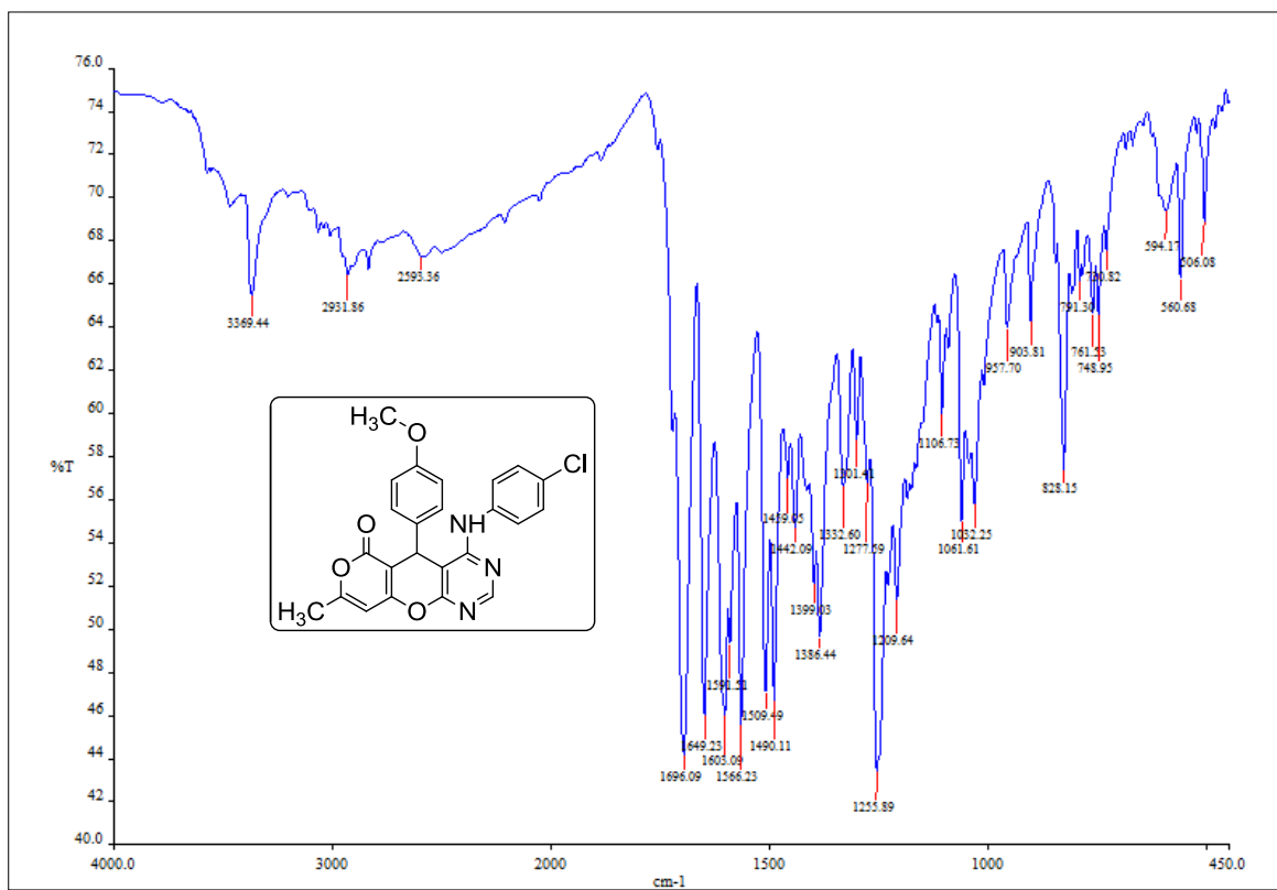
IR Spectrum of compound 4j
