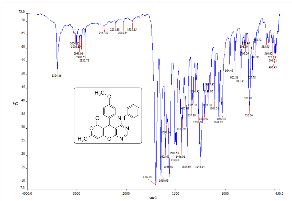
IR Spectrum of compound 4i
