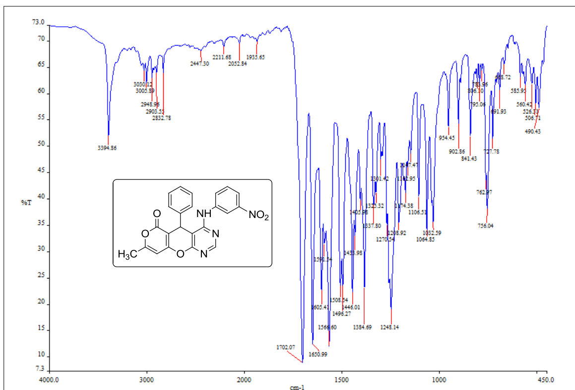
IR Spectrum of compound 4c
