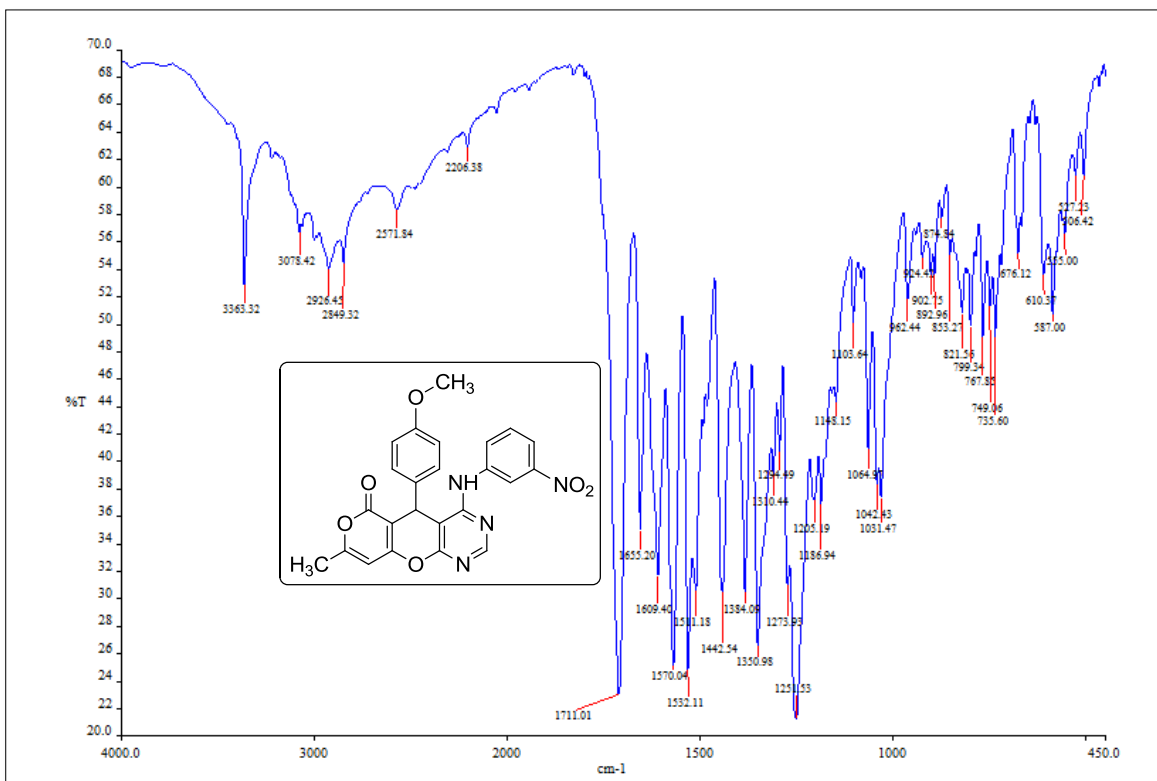
IR Spectrum of compound 4k
