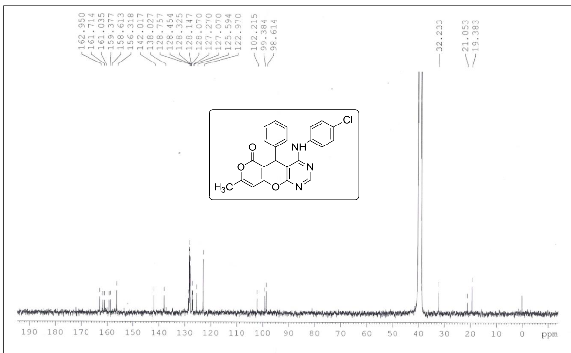
13 C NMR Spectrum of compound 4b
