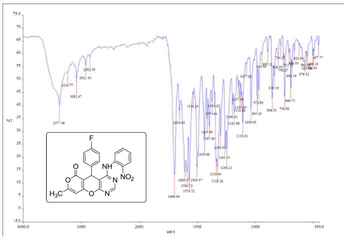
IR Spectrum of compound 4g
