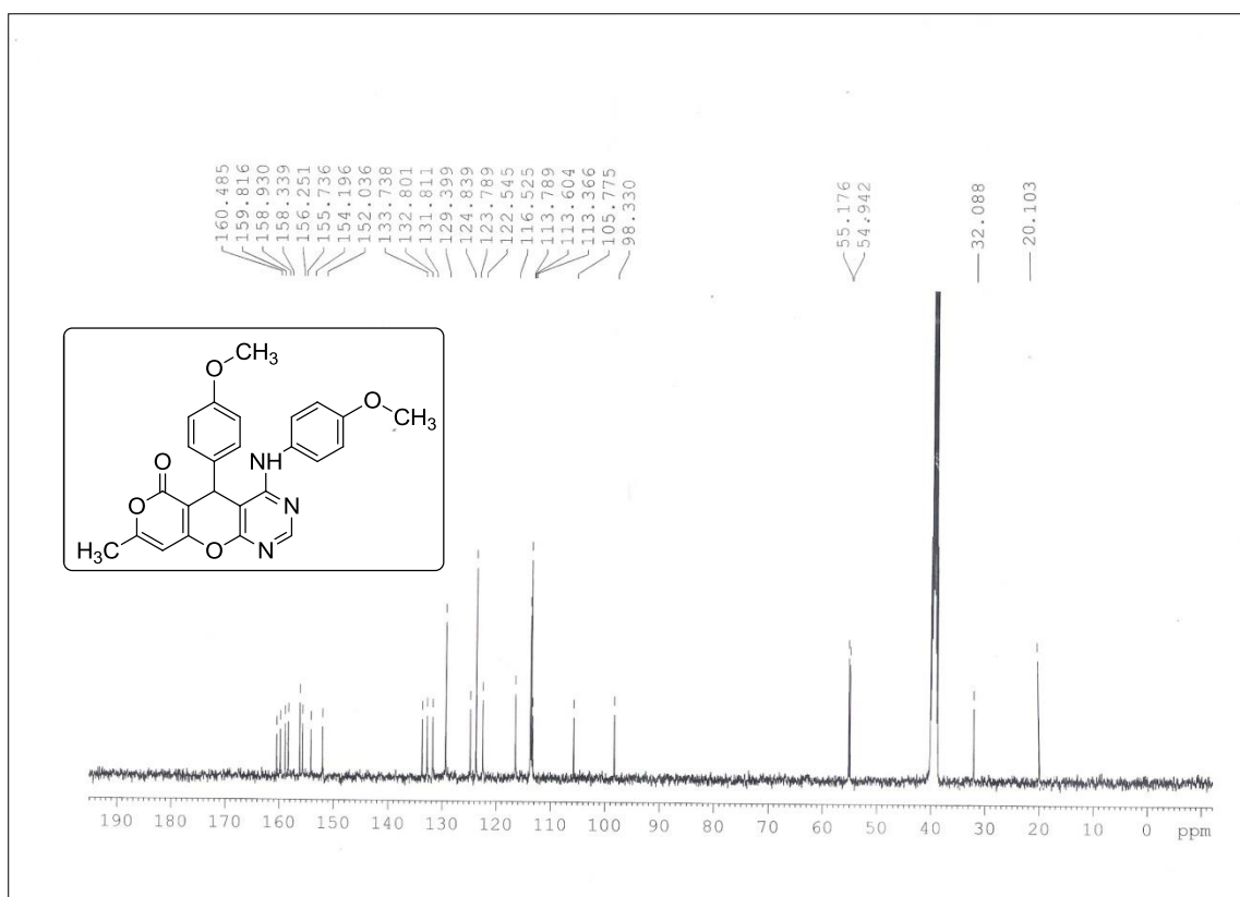
^{13}\text{C} NMR Spectrum of compound 41
