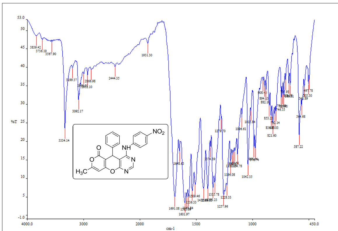
IR Spectrum of compound 4h
