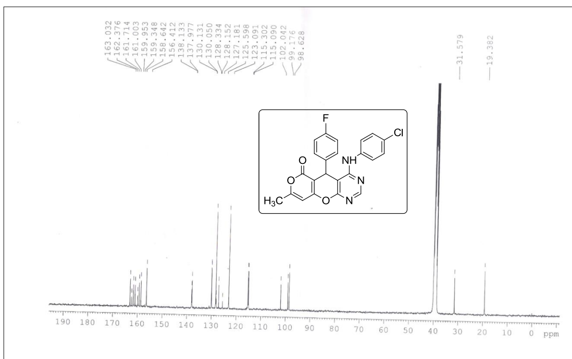
13 C NMR Spectrum of compound 4f
