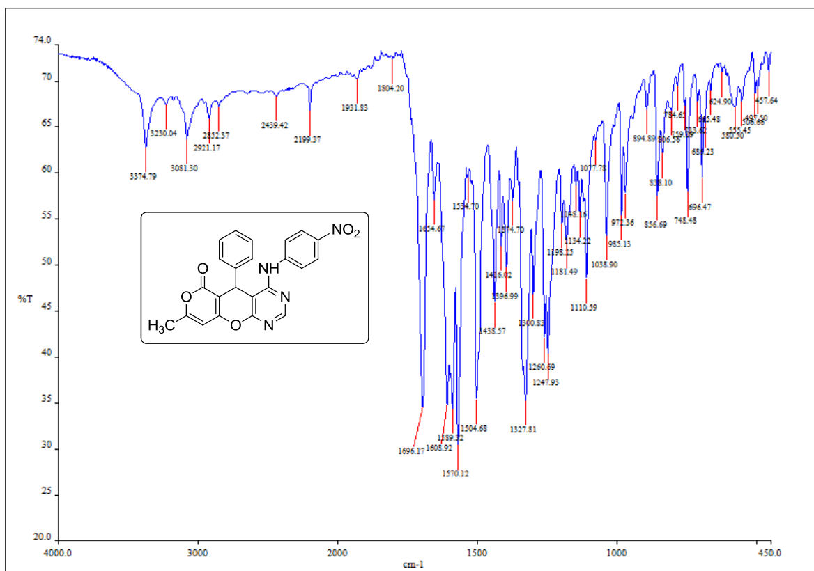
IR Spectrum of compound 4d
