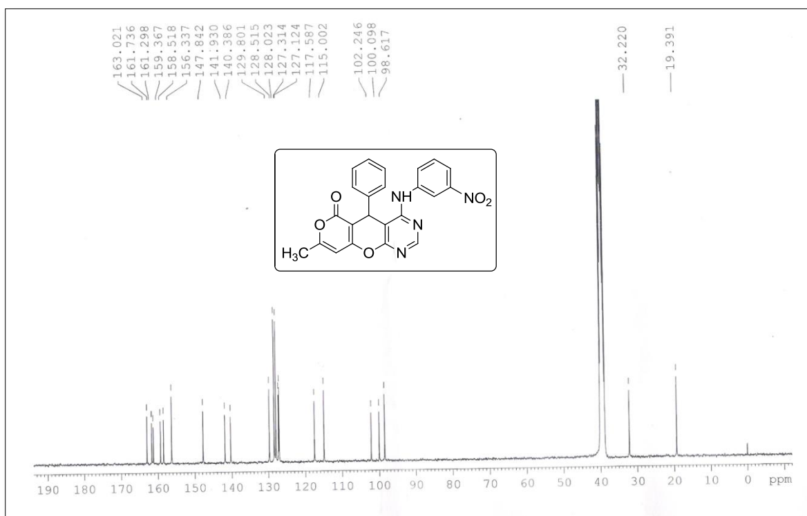
13 C NMR Spectrum of compound 4c
