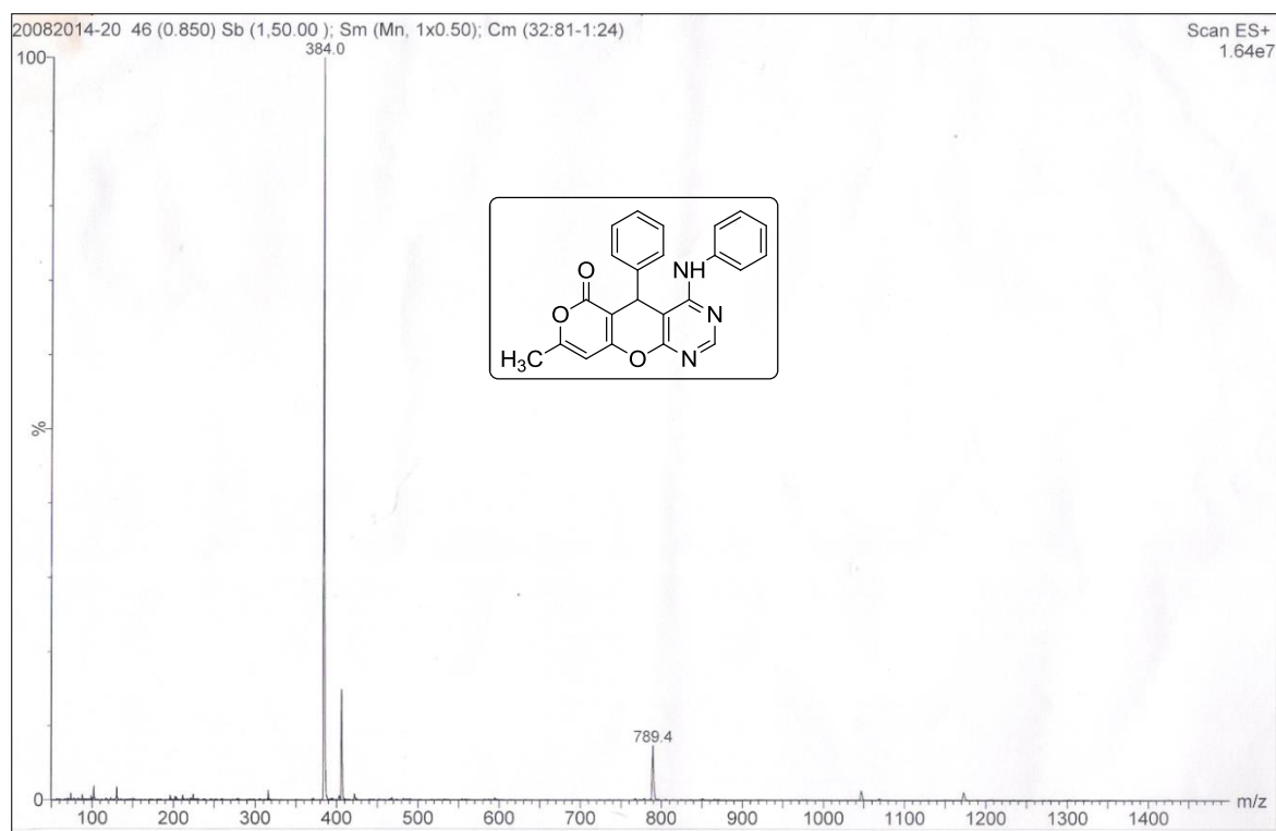
Mass Spectrum of compound 4a
