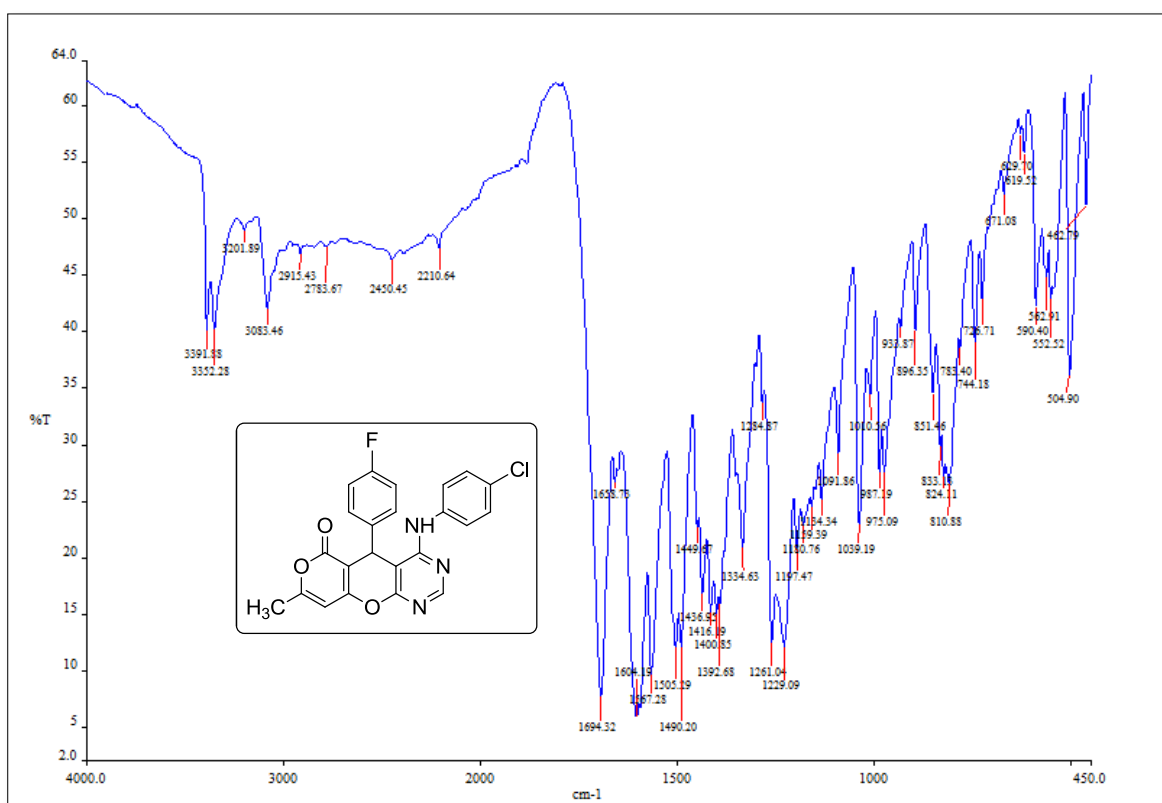
IR Spectrum of compound 4f
