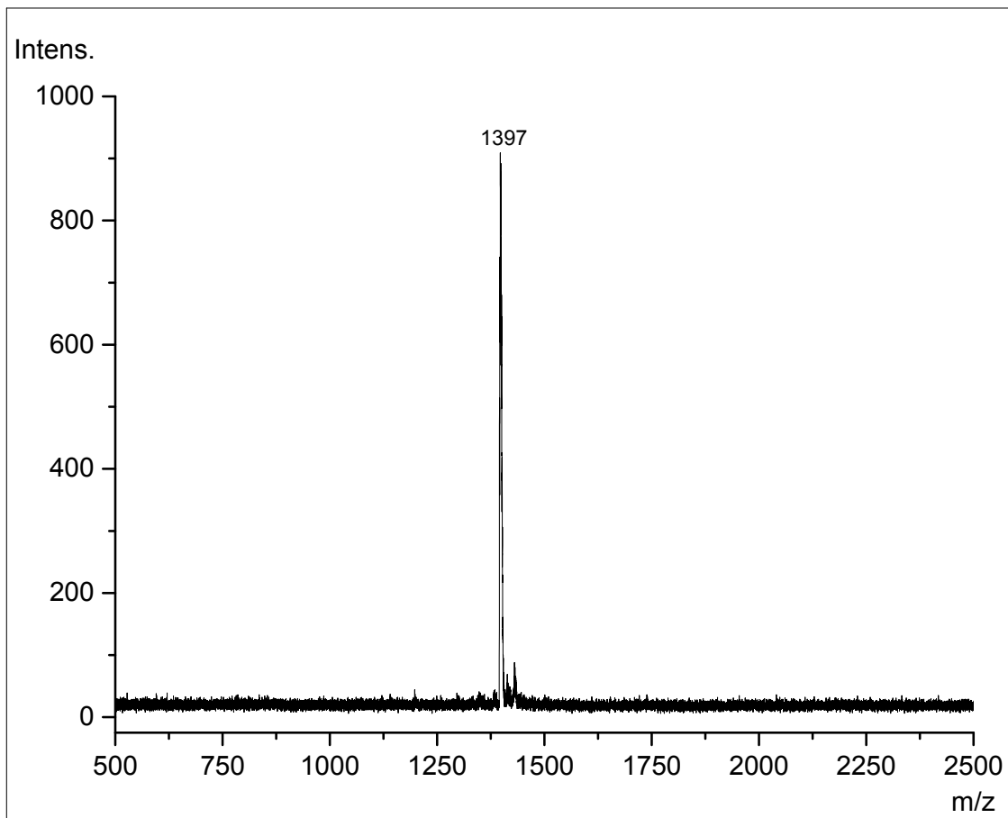
Fig. S27. MALDI TOF spectrum of Ph 4 TAQP-Zn (positive mode).
