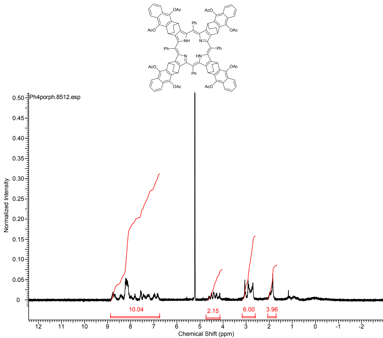
Fig. S21. 1 H NMR spectrum of compound 12.
