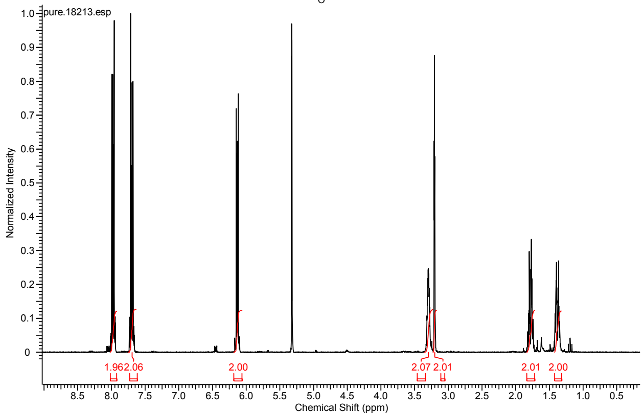
Fig. S11. ^1\text{H} NMR spectrum of compound 7.
