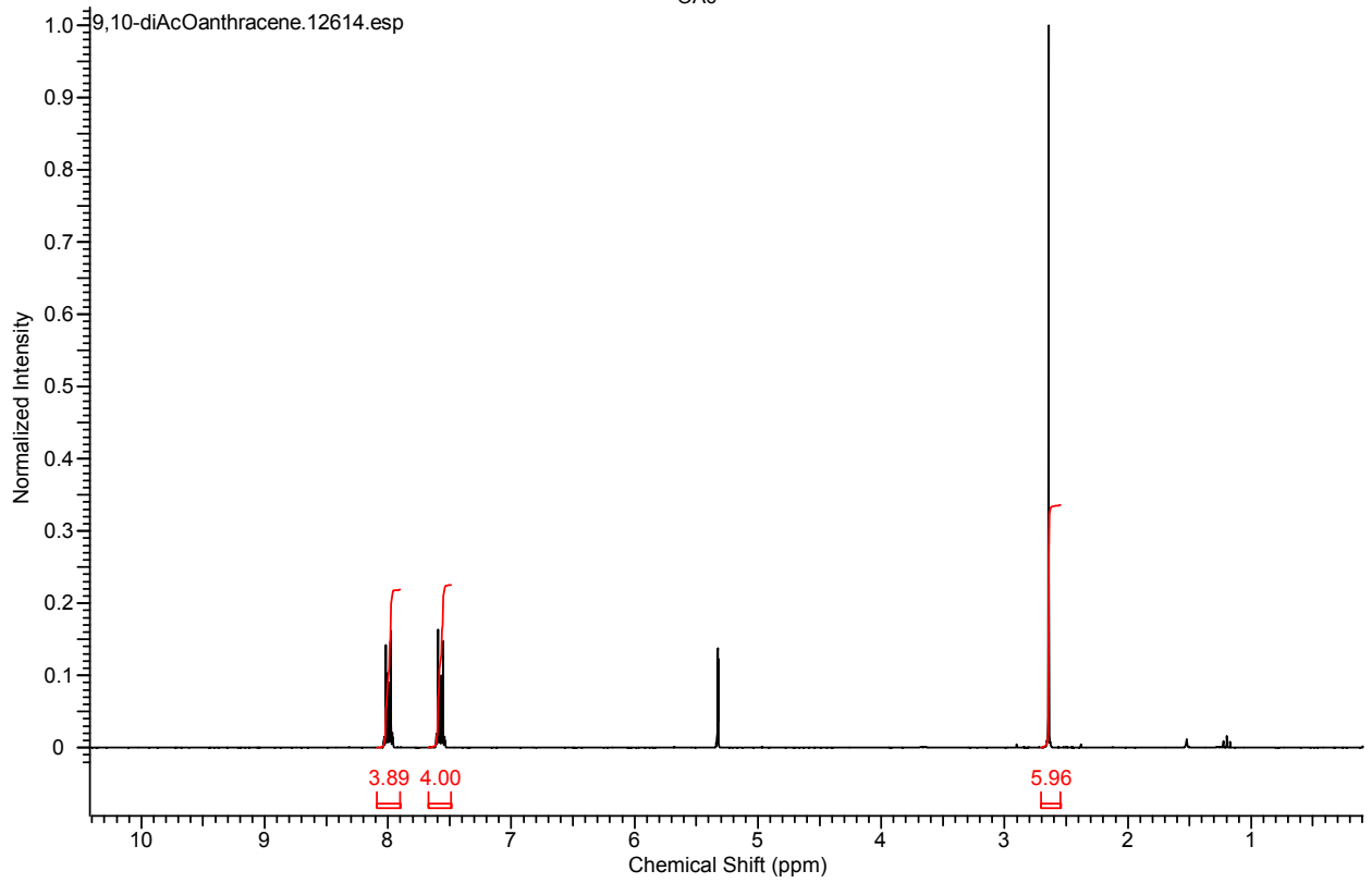
Fig. S9. ^1\text{H} NMR spectrum of compound 6 .
