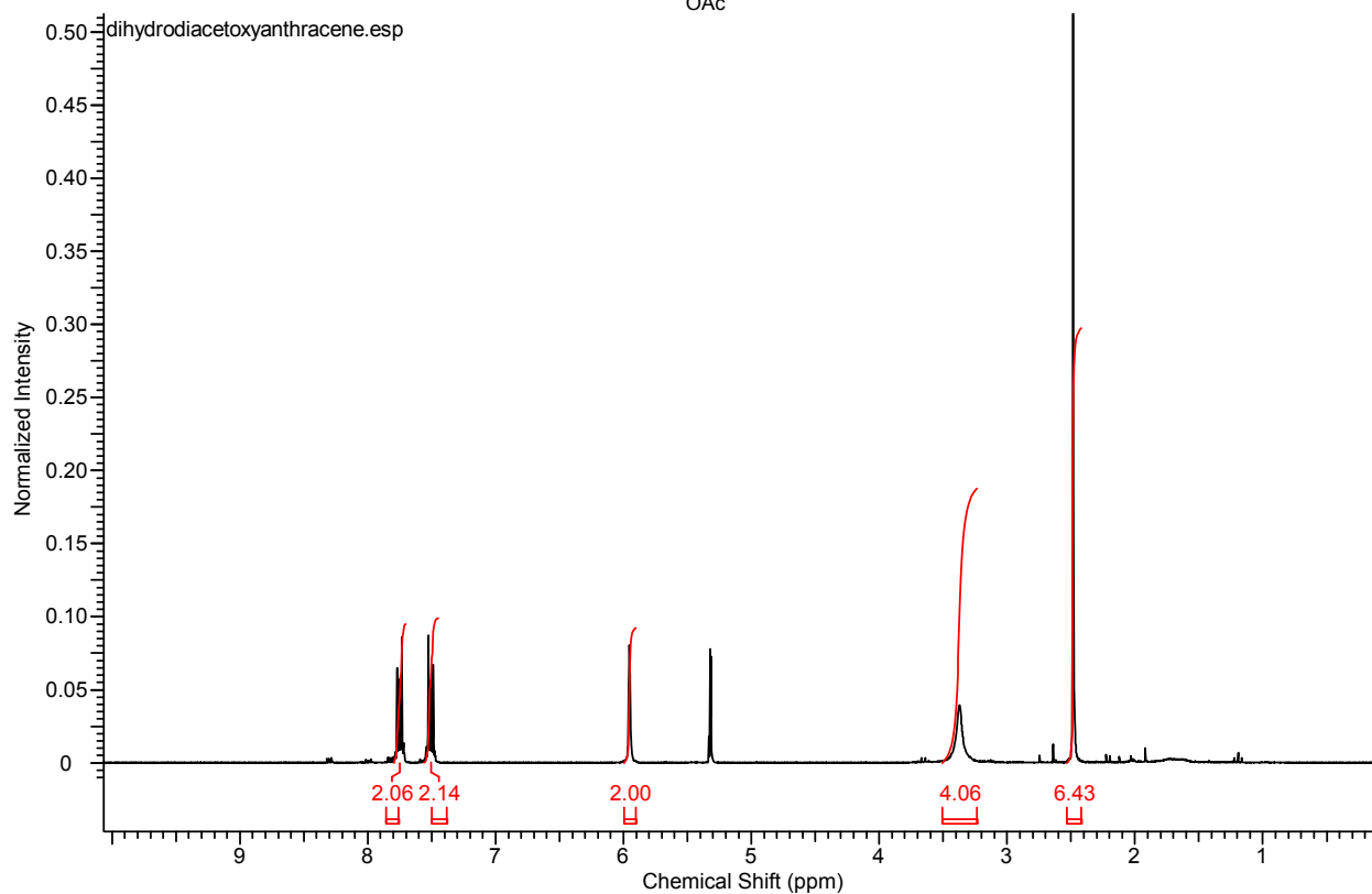
Fig. S5. ^1\text{H} NMR spectrum of compound 4.
