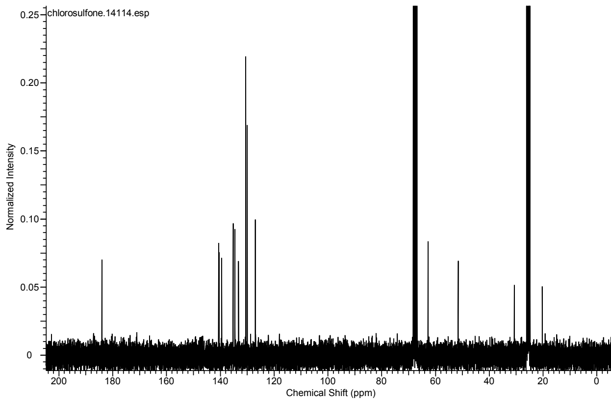
Fig. S2. ^{13}\text{C} NMR spectrum of compound 2 .
