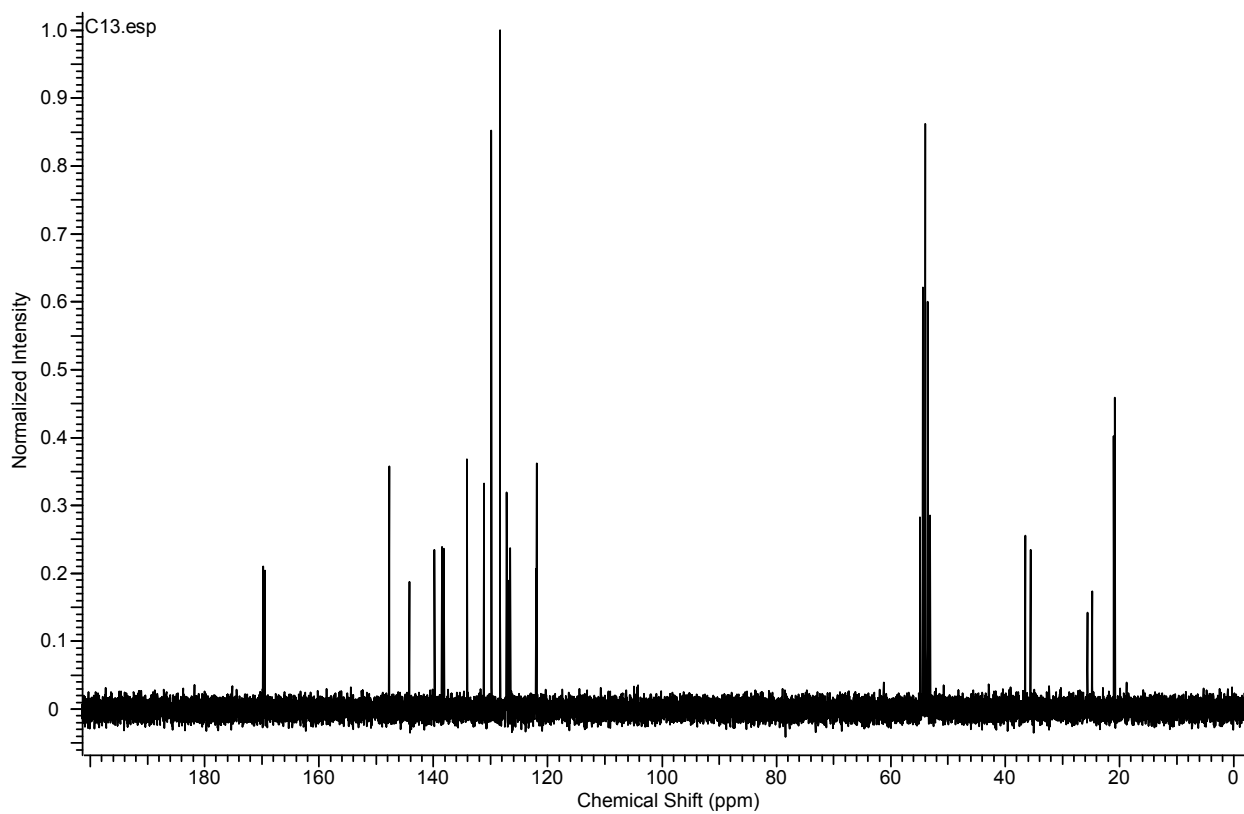
Fig. S16. ^{13}\text{C} NMR spectrum of compound 9 .
