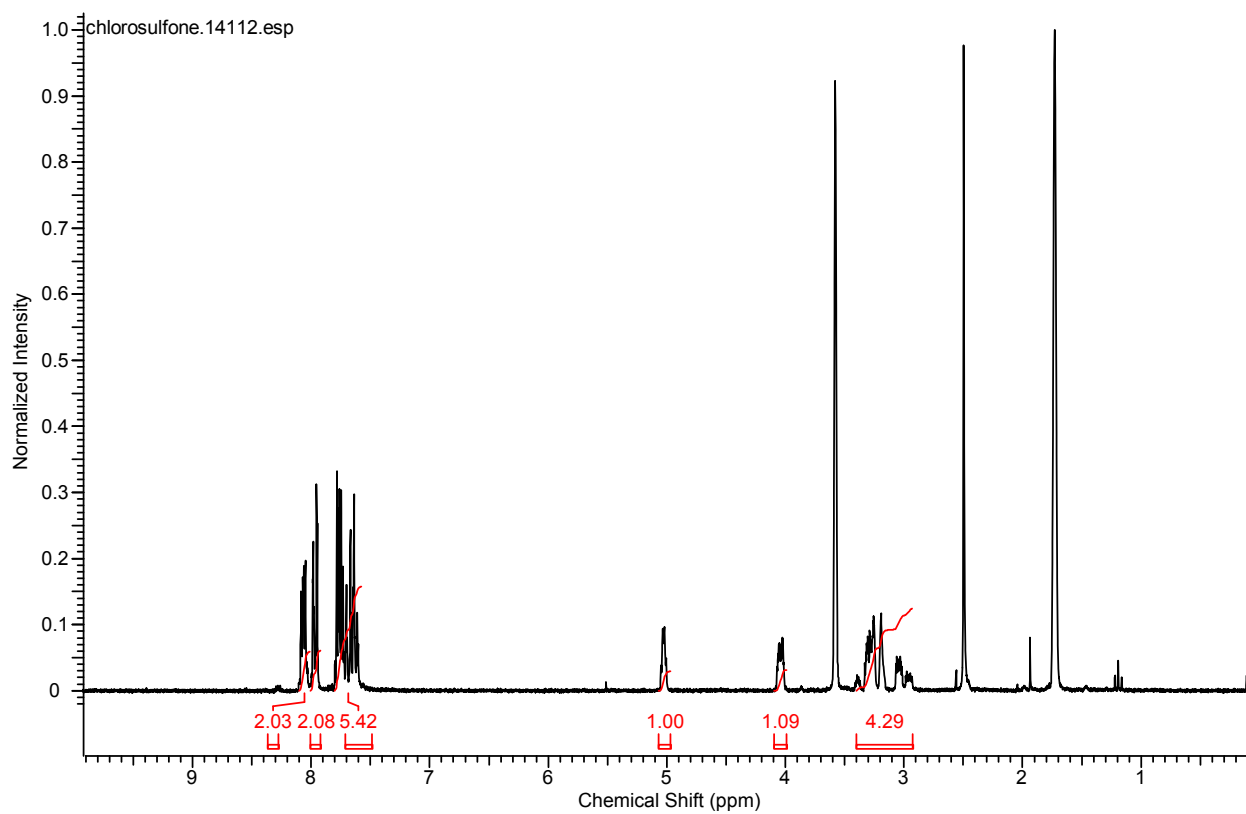
Fig. S1. ^1\text{H} NMR spectrum of compound 2 .
