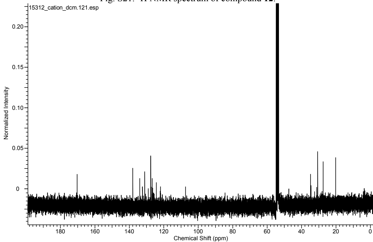
Fig. S22. 13 C NMR of compound 12.
