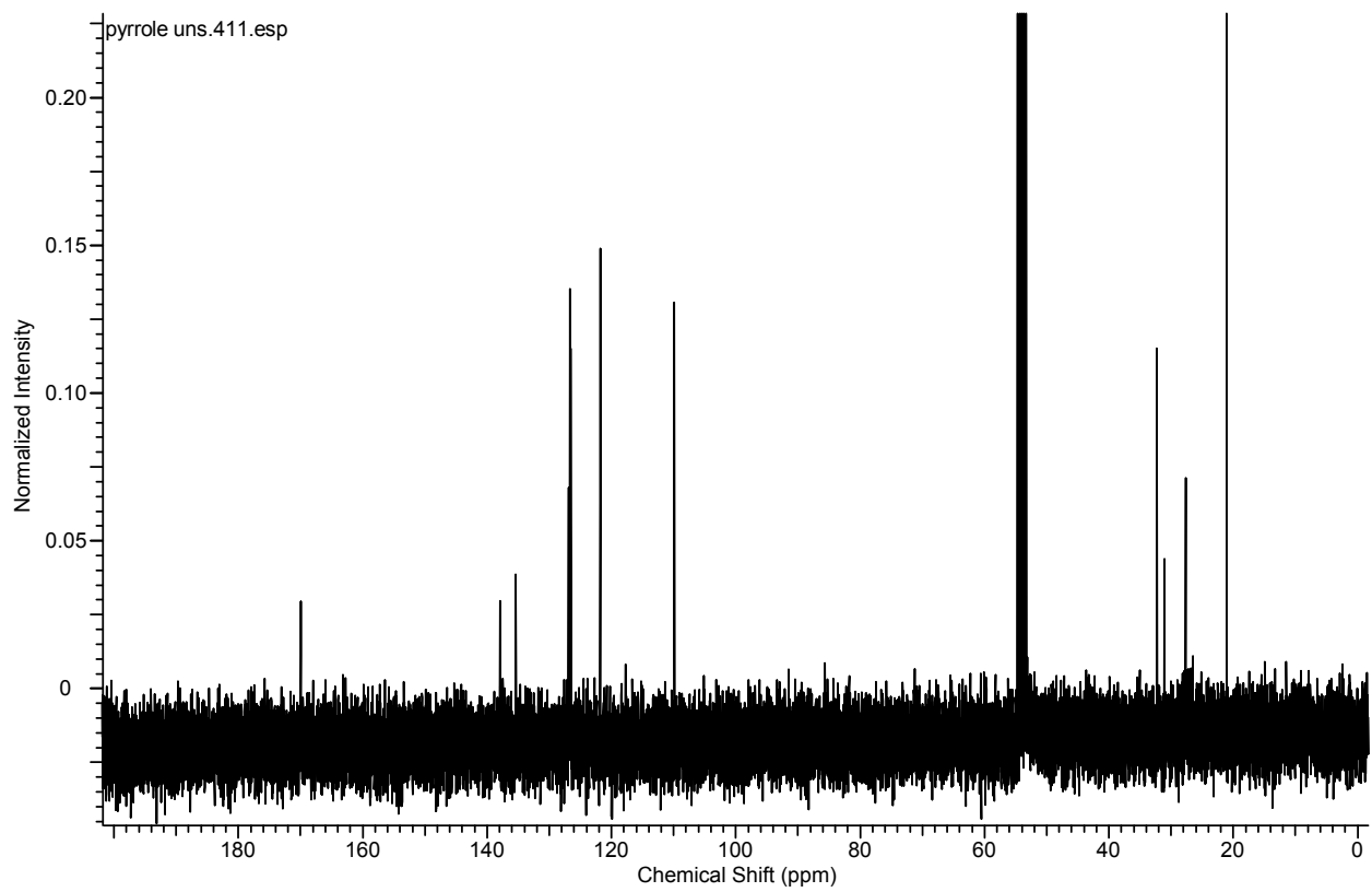
Fig. S20. ^{13}\text{C} NMR spectrum of compound 11.
