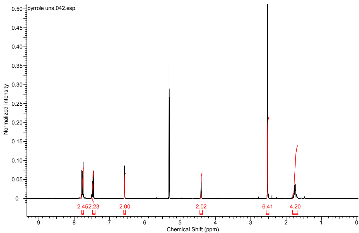
Fig. S19. ^1\text{H} NMR spectrum of compound 11.
