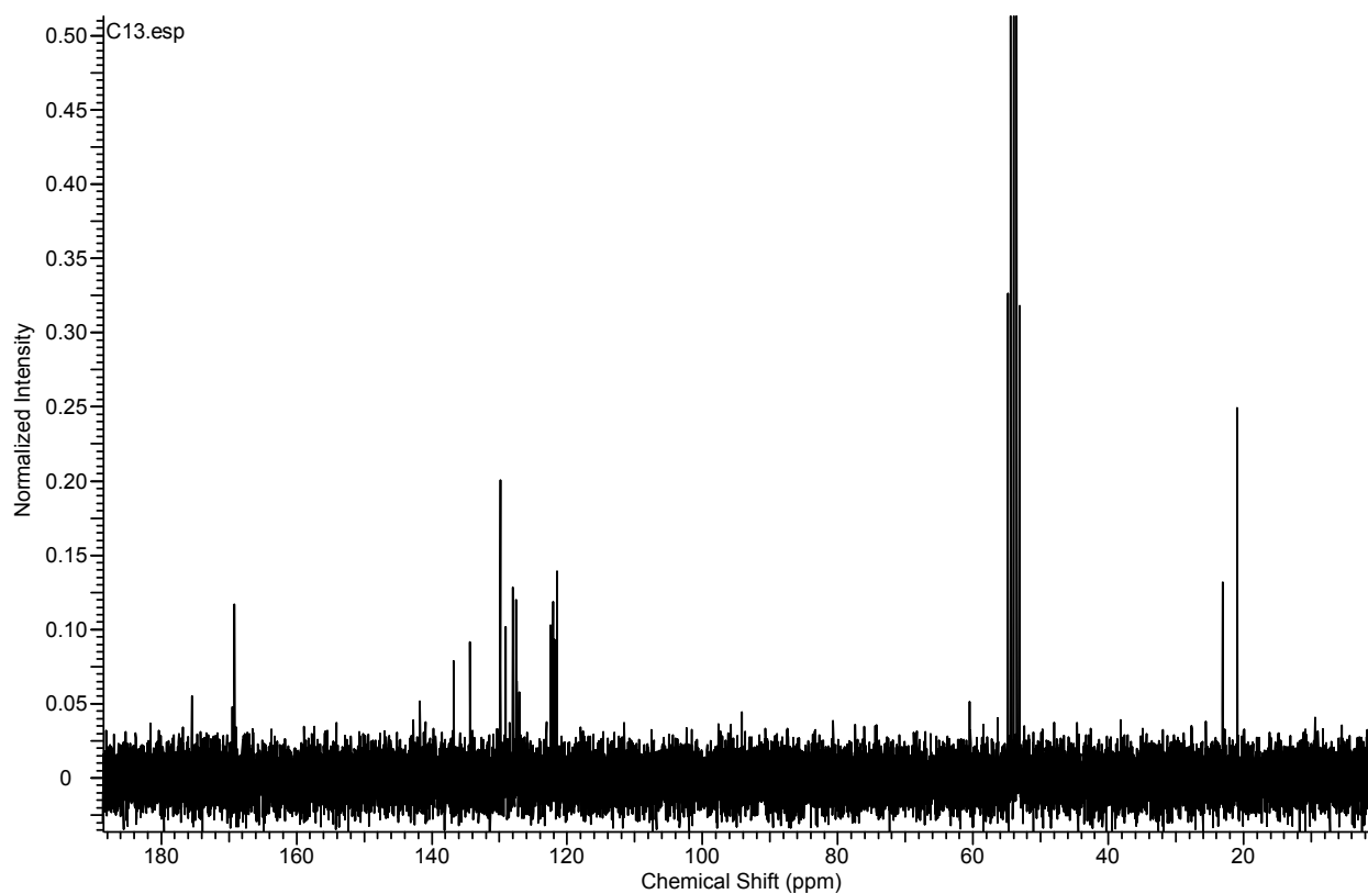
Fig. S8. ^{13}\text{C} NMR spectrum of compound 5 .
