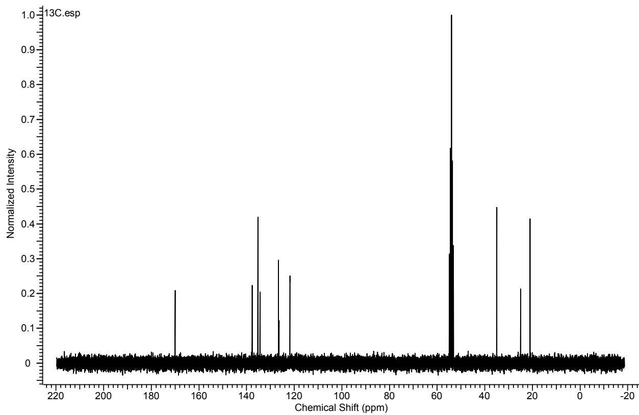
Fig. S14. 13 C NMR spectrum of compound 8 .
