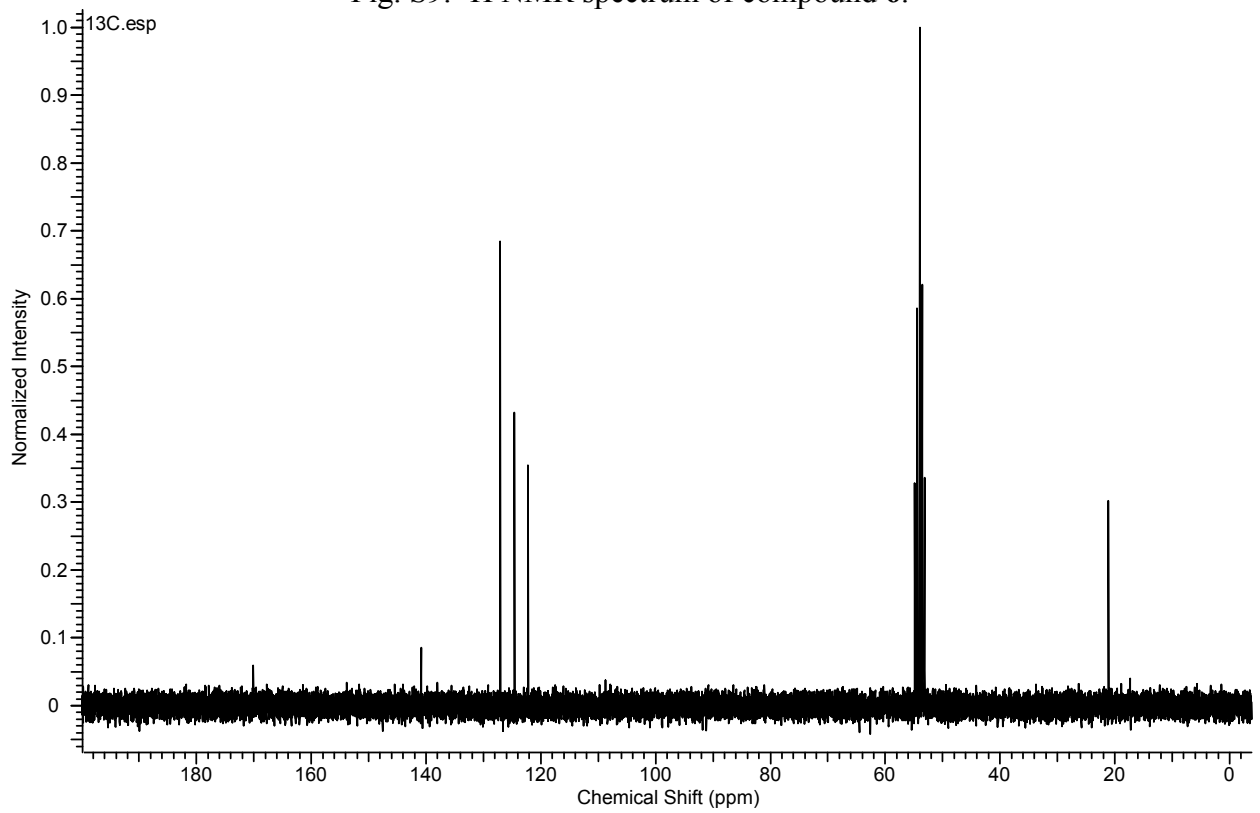
Fig. S10. ^{13}\text{C} NMR spectrum of compound 6 .
