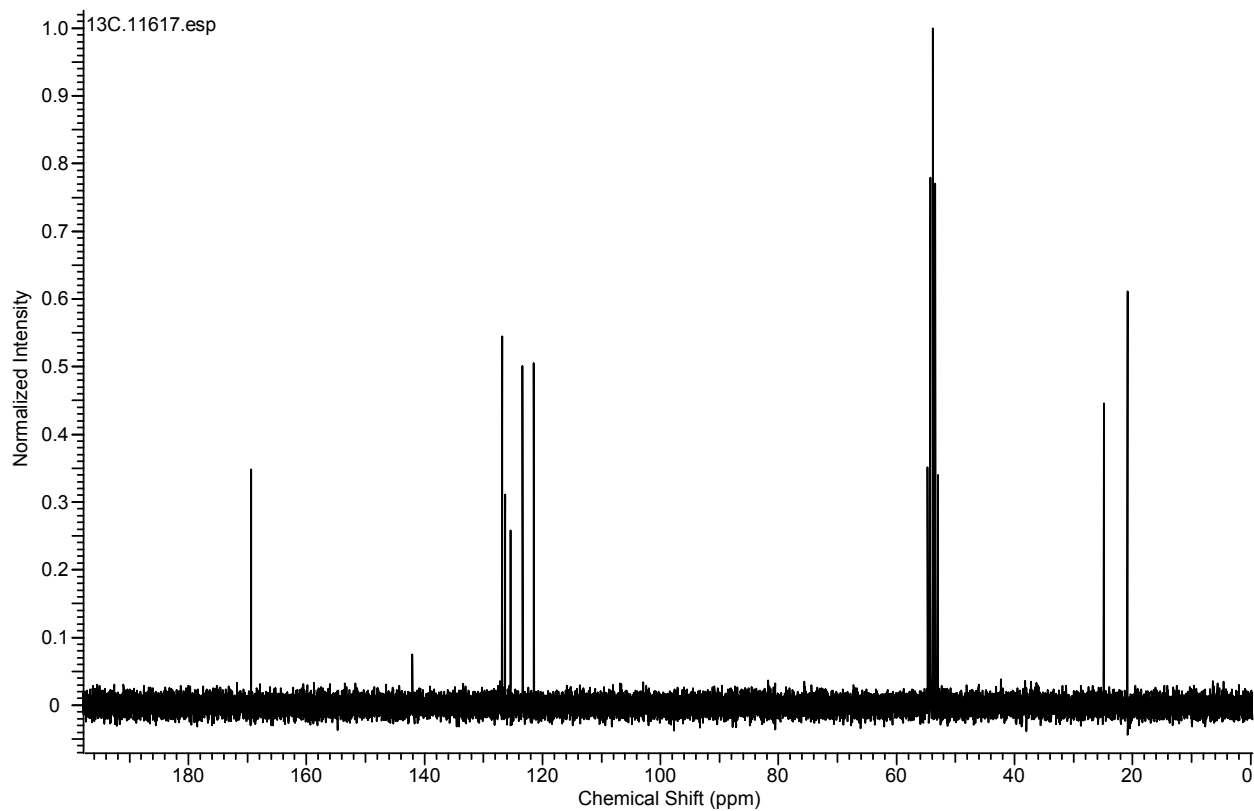
Fig. S6. ^{13}\text{C} NMR spectrum of compound 4.
