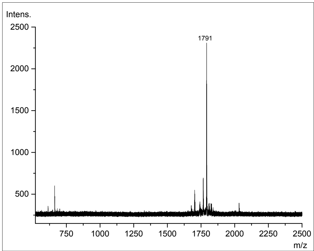
Fig. S23. MALDI TOF spectrum of 12 (positive mode).
