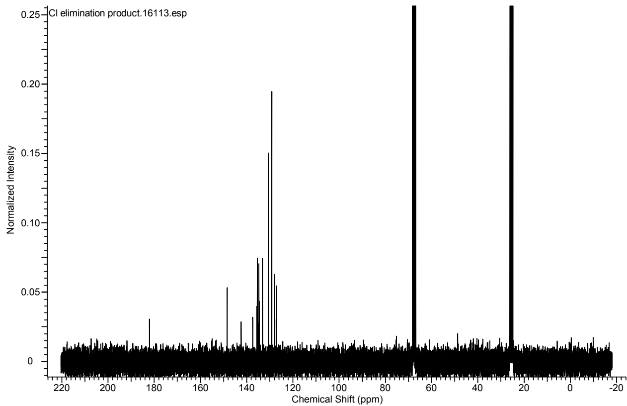
Fig. S4. ^{13}\text{C} NMR spectrum of compound 3 .
