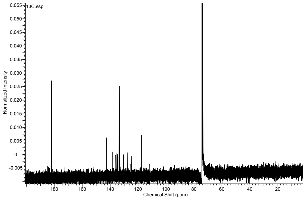
Fig. S25. ^{13}\text{C} NMR spectrum of compound Ph 4 TAQP .
