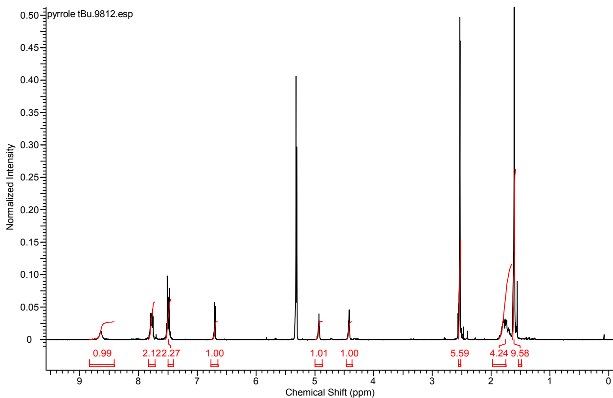
Fig. S17. ^1\text{H} NMR spectrum of compound 10 .
