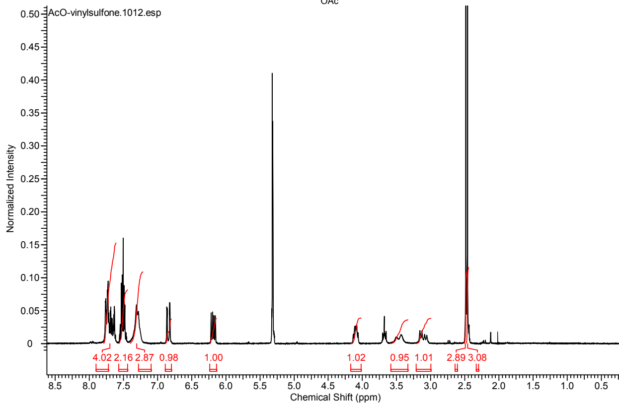
Fig. S7. ^1\text{H} NMR spectrum of compound 5 .
