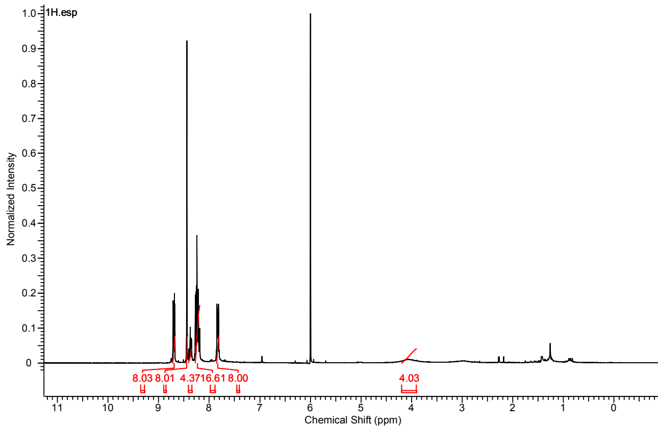
Fig. S24. ^1\text{H} NMR spectrum of compound \text{Ph}_4\text{TAQP} .
