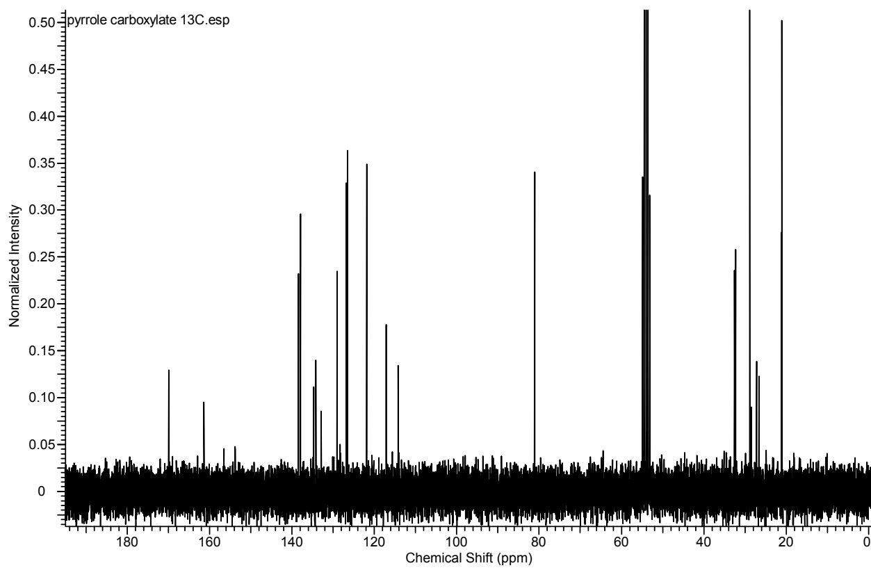
Fig. S18. ^{13}\text{C} NMR spectrum of compound 10 .
