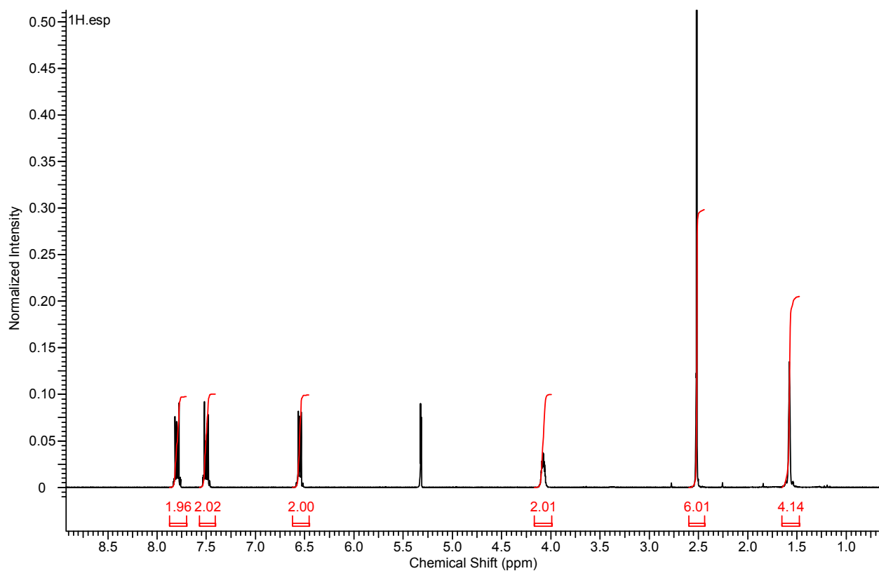
Fig. S13. 1 H NMR spectrum of compound 8 .
