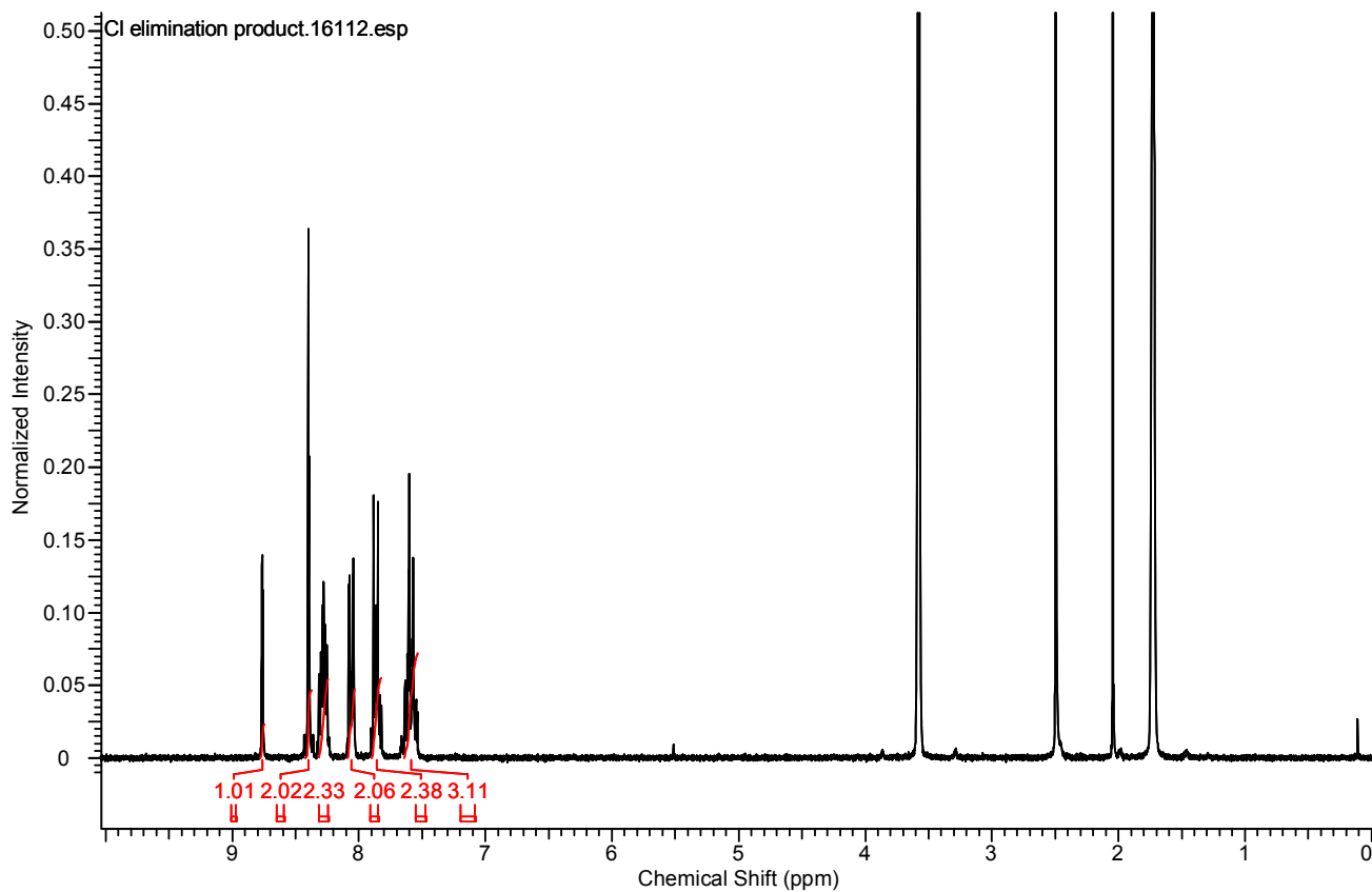
Fig. S3. 1 H NMR spectrum of compound 3.
