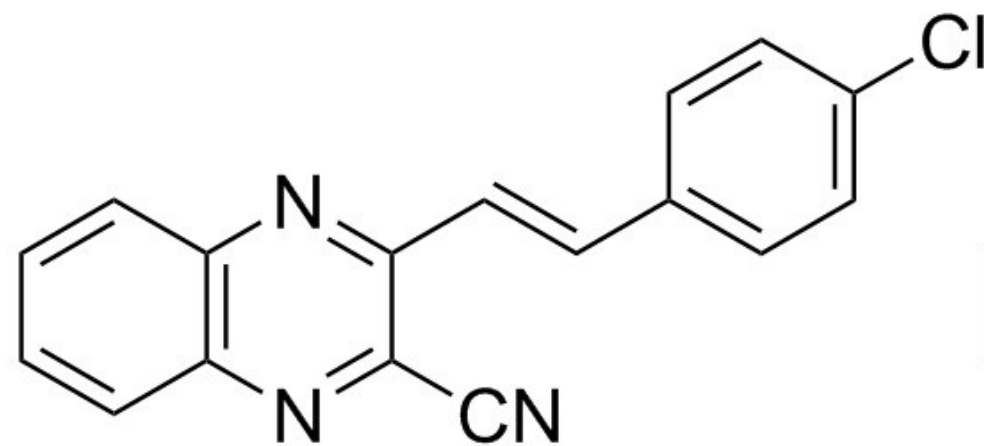
6a (92%, 10 min)
