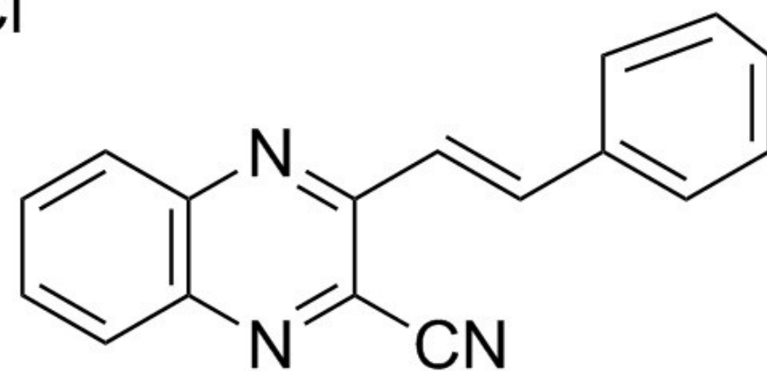
6f (91%, 15 min)
