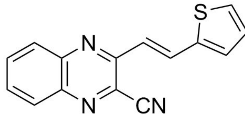
6h (95%, 20 min)
