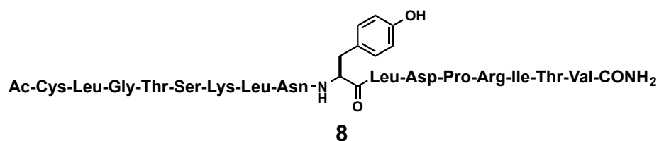
Figure S2. Unmodified peptide 8 .
