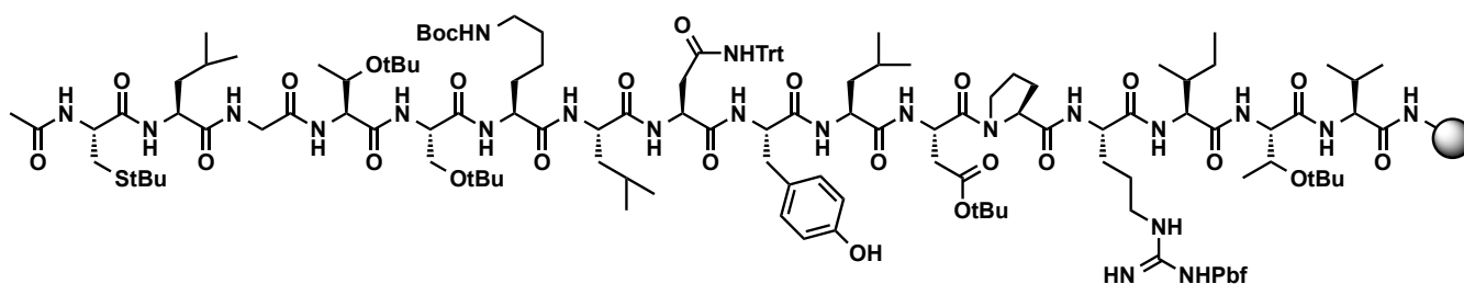
Figure S1. Resin bound peptide for direct conjugation.
