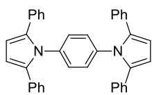
1,1'-p-phenylenebis[2,5-diphenylpyrrole] (5)
