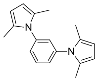
2,5-Dimethyl-1-(3-(2,5-dimethyl-1H-pyrrol-1-yl)phenyl)-1H-pyrrole (2)
