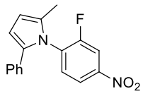
1-(2-Fluoro-4-nitrophenyl)-2-methyl-5-phenyl-1H-pyrrole ( 18 )
