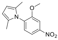
1-(2-Methoxy-4-nitrophenyl)-2,5-dimethyl-1H-pyrrole (10)
