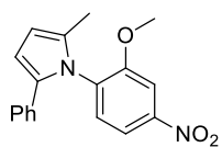
1-(2-Methoxy-4-nitrophenyl)-2-methyl-5-phenyl-1H-pyrrole (17)
