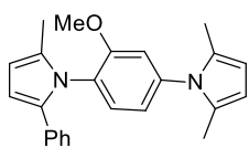
2,5-Dimethyl-1-[3-methoxy-4-(2-methyl-5-phenyl-1H-pyrrol-1-yl)phenyl]-1H-pyrrole ( 29 )
