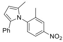
2-Methyl-1-(2-methyl-4-nitrophenyl)-5-phenyl-1H-pyrrole ( 15 )
