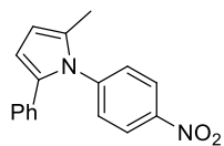
2-Methyl-1-(4-nitrophenyl)-5-phenyl-1H-pyrrole ( 13 )
