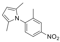
2,5-Dimethyl-1-(2-methyl-4-nitrophenyl)-1H-pyrrole ( 8 )
