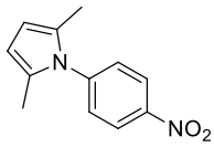
2,5-Dimethyl-1-(4-nitrophenyl)-1H-pyrrole (6)
