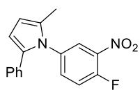
1-(4-Fluoro-3-nitrophenyl)-2-methyl-5-phenyl-1H-pyrrole ( 19 )
