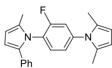
2,5-Dimethyl-1-[3-fluoro-4-(2-methyl-5-phenyl-1H-pyrrol-1-yl)phenyl]-1H-pyrrole ( 30 )
