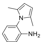
2-(2,5-dimethyl-1H-pyrrol-1-yl)benzeneamine (1')
