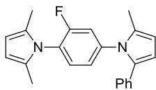
2,5-Dimethyl-1-[2-fluoro-4-(2-methyl-5-phenyl-1H-pyrrol-1-yl)phenyl]-1H-pyrrole ( 25 )
