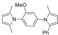
2,5-Dimethyl-1-[2-methoxy-4-(2-methyl-5-phenyl-1H-pyrrol-1-yl)phenyl]-1H-pyrrole ( 24 )
