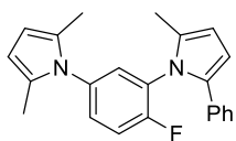
2,5-Dimethyl-1-[4-fluoro-3-(2-methyl-5-phenyl-1H-pyrrol-1-yl)phenyl]-1H-pyrrole ( 26 )
