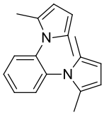
2,5-Dimethyl-1-(2-(2,5-dimethyl-1H-pyrrol-1-yl)phenyl)-1H-pyrrole (1)
