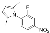
1-(2-Fluoro-4-nitrophenyl)-2,5-dimethyl-1H-pyrrole (11)
