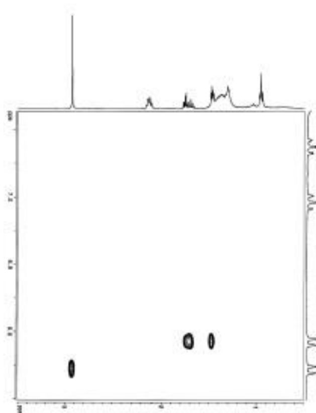
NOESY of compound 4s (400MHz, C 6 D 6 )
