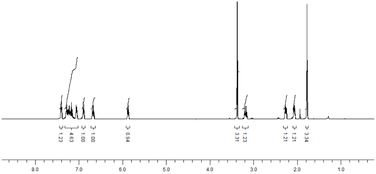
3i d.r. 92:8
