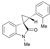
3i d.r. 92:8
