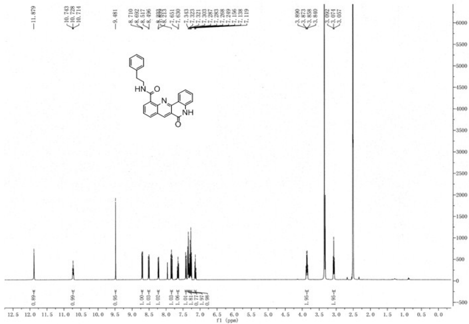
6-Oxo-N-phenethyl-5,6-dihydrodibenzo[b,h][1,6]naphthyridine-11-carboxamide ( 31 )
