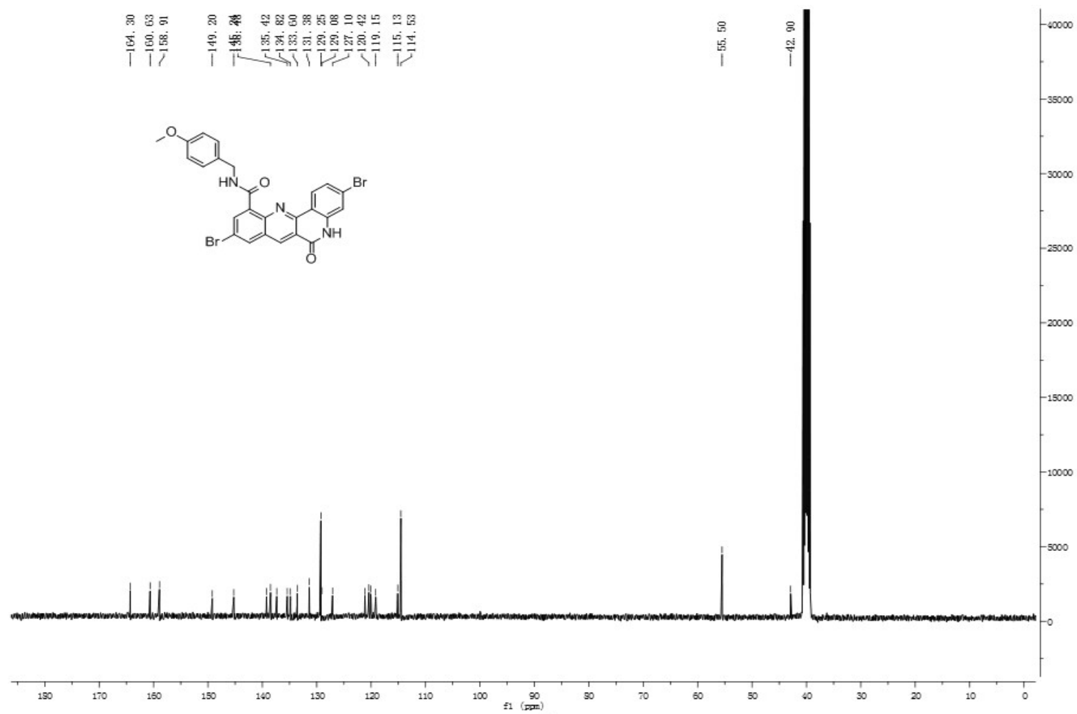
3,9-Dibromo-N-(4-methoxybenzyl)-6-oxo-5,6-dihydrodibenzo[b,h][1,6]naphthyridine-11-carboxamide ( 3r )
