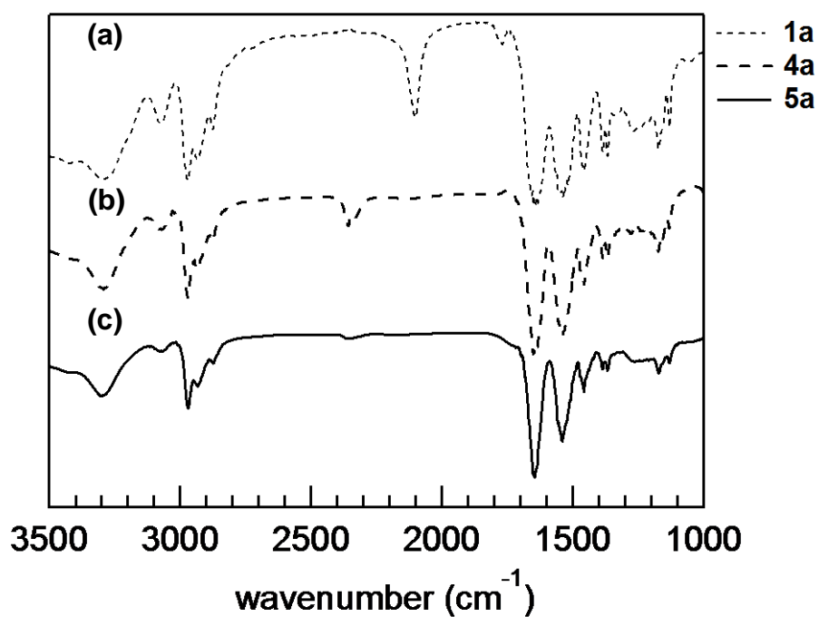
Figure S2. FT-IR spectra of (a) 1a , (b) 4a , and (c) 5a .
