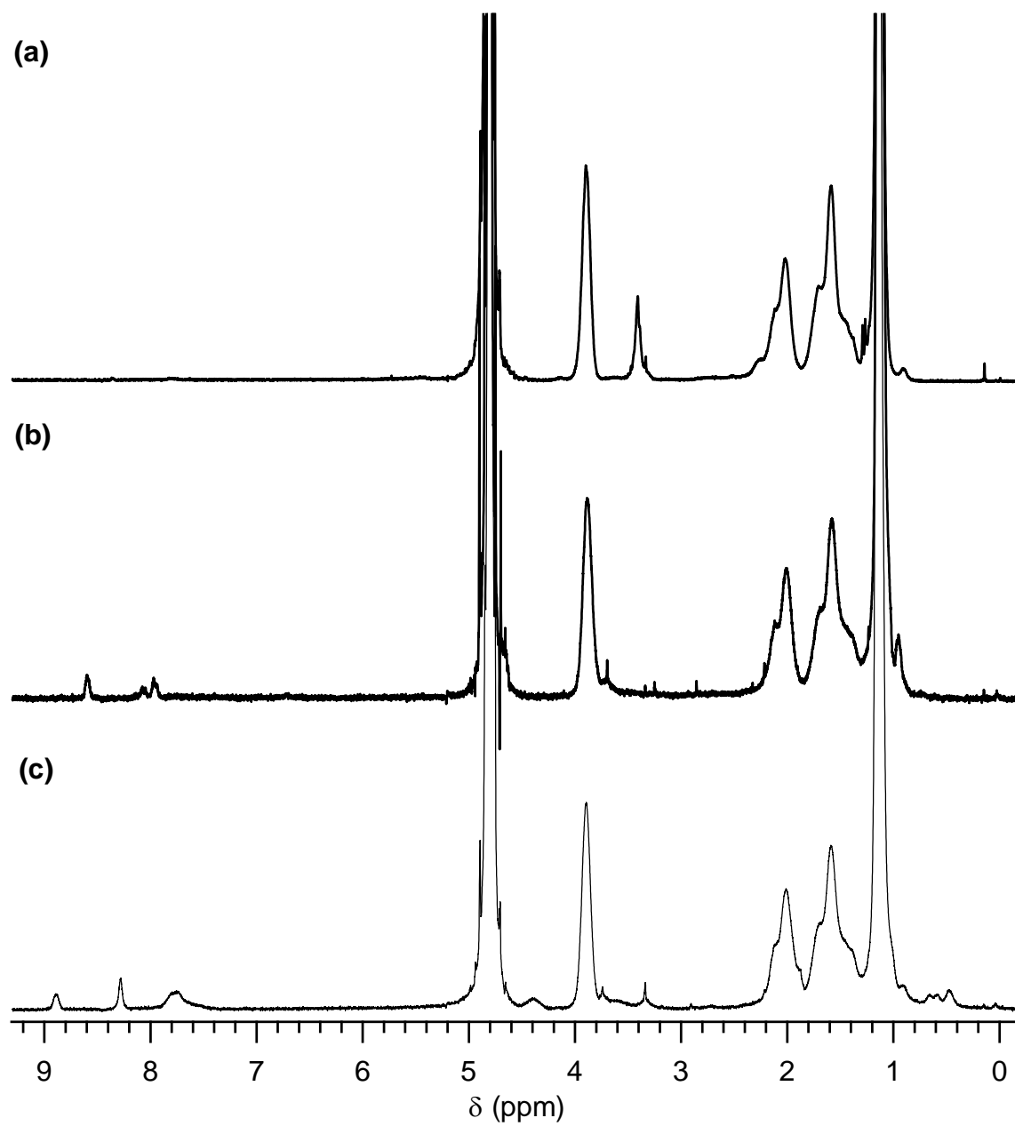
Figure S1. ^1\text{H} NMR spectra of (a) 1a , (b) 4a , and (c) 5a in \text{CDCl}_3 .
