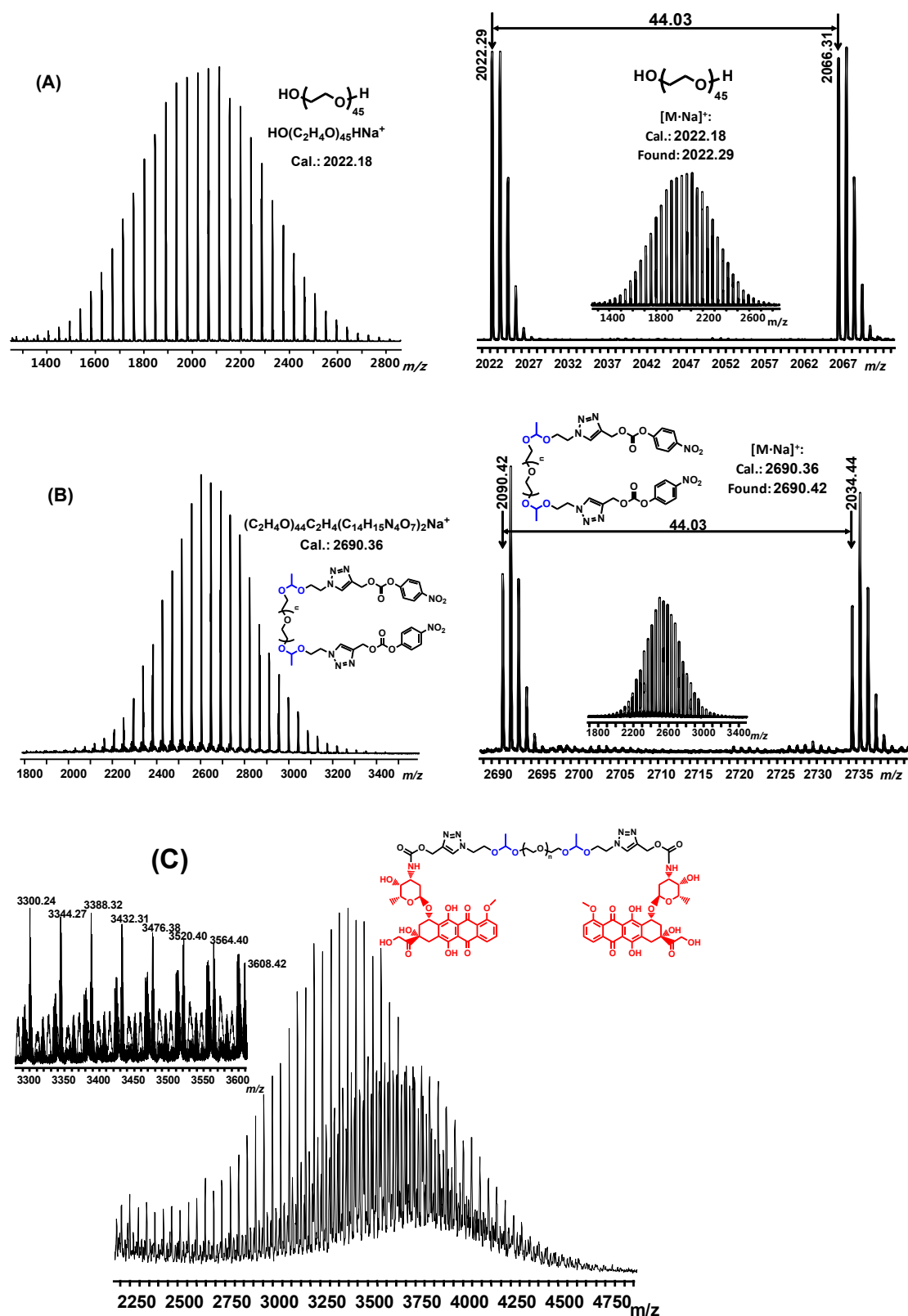
Fig. S1 MALDI-TOF mass spectra using Na salt as the cationization agent and a DCTB matrix. (A) HO-PEG 45 -OH, (B) NC- \alpha -PEG 45 - \alpha -NC and (C) P45.
