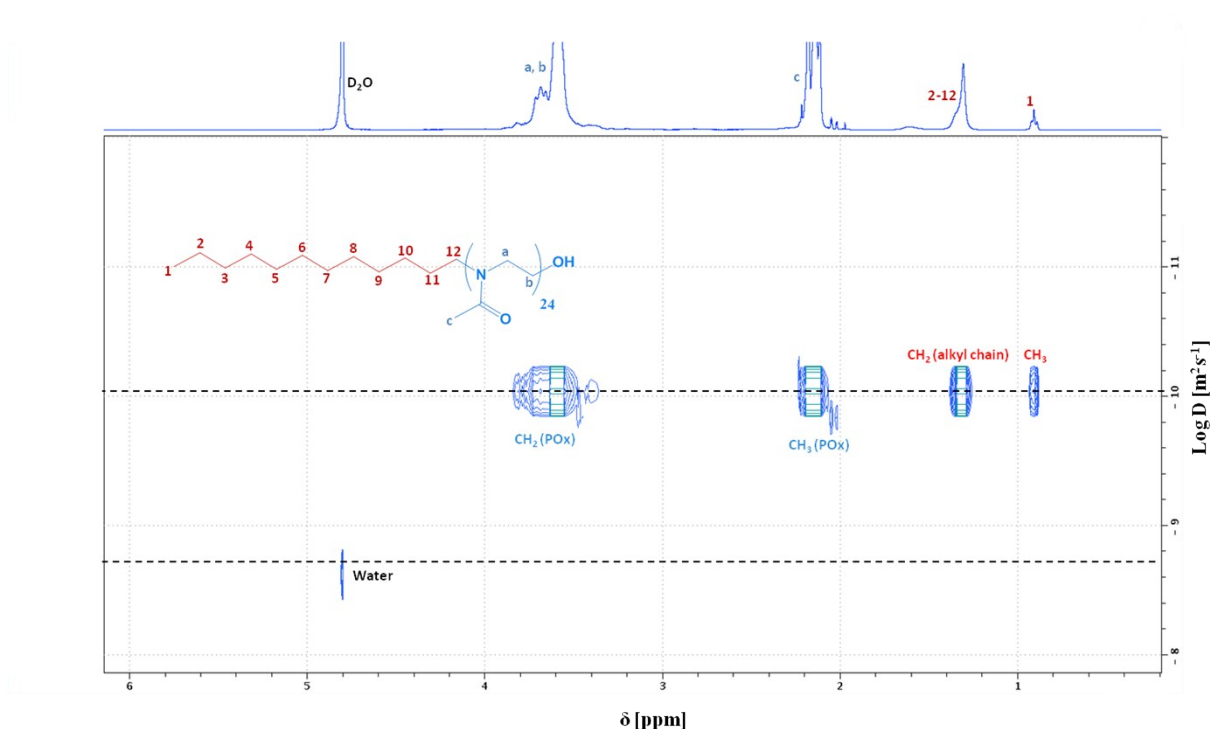
Figure X. 1 H DOSY NMR spectrum (600 MHz; D 2 O) of C 12 -POx 24 dissolved in water at 11.7 mg mL -1 .
