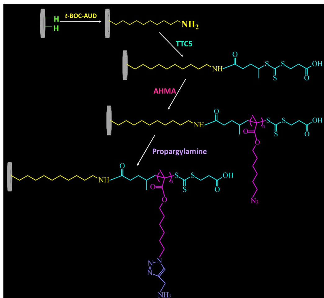
SCHEME S1 Synthetic routes of the amine functionalized poly(AHMA) brushes
