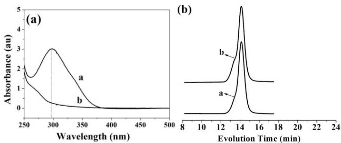
Fig. S3. (a) UV-vis spectra of POEGMA 42 - b -P( t BMA 200 -BiBOEMD 7 ) block copolymer prepared by two-step RAFT polymerization (spectrum a) and the block
