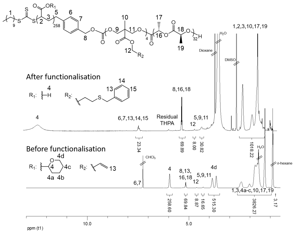
Figure S7. 1 H NMR spectrum (400 MHz) of benzyl mercaptan functionalized PLLA- b -PMAC- b -PAA triblock copolymer (top, d 6 -DMSO) and non-functionalized PLLA- b -PMAC- b -PTHPA (bottom, CDCl 3 ).
