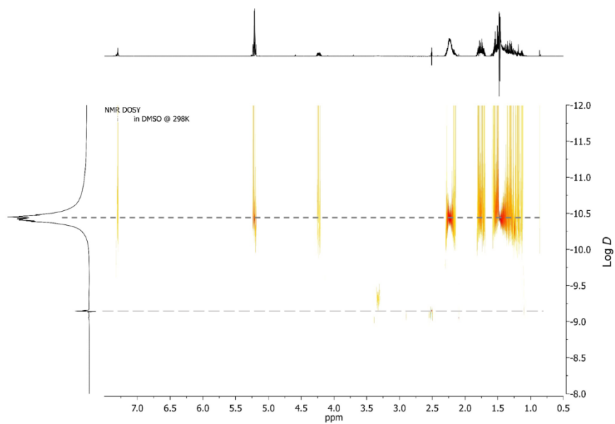
Figure S6. DOSY 1 H NMR spectrum (500 MHz, d 6 -DMSO) of benzyl mercaptan functionalized PLLA- b -PMAC- b -PAA triblock unimers.
