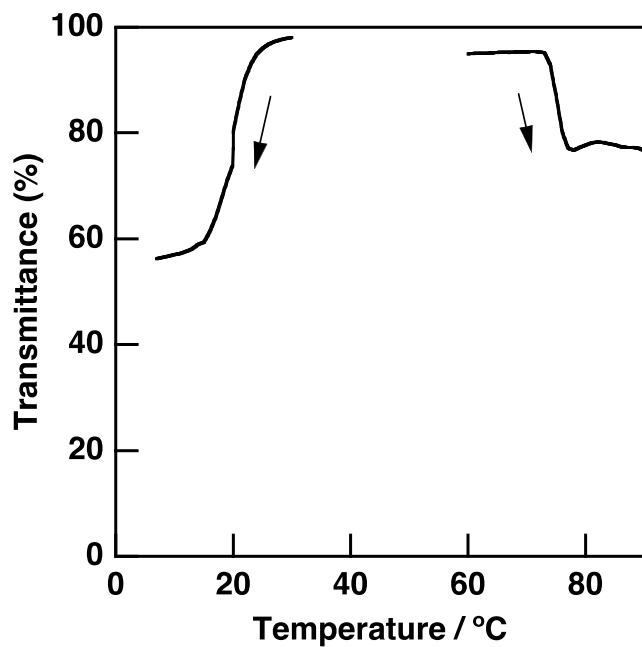
Fig. S1 Turbidity curves of an aqueous solution of 2.0 g/L \text{MOVE}_{200}\text{-}b\text{-}([\text{EtIm}][\text{BF}_4])_{200} containing 60 mM \text{NaBF}_4 , scan rate: 1 °C/min.
