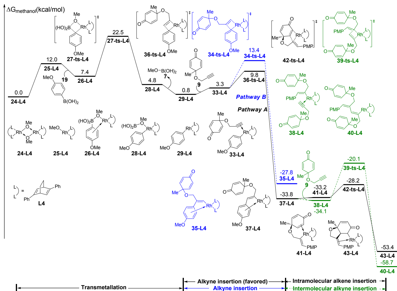
Figure S5. Free energy profile for rhodium-catalyzed synthesis of hydrobenzofurans with L4 ligand.
