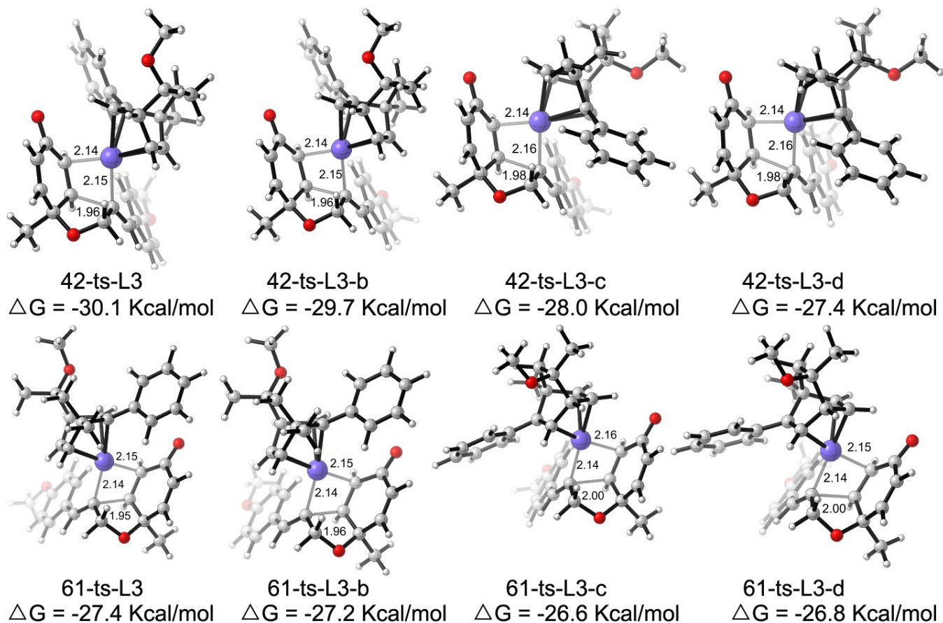
Figure S4. Geometries of 42-ts and 61-ts with L3 ligand. The values of bond lengths are given in angstrom. The values given in kcal/mol are the MN12-L calculated relative free energies in methanol solvent.
