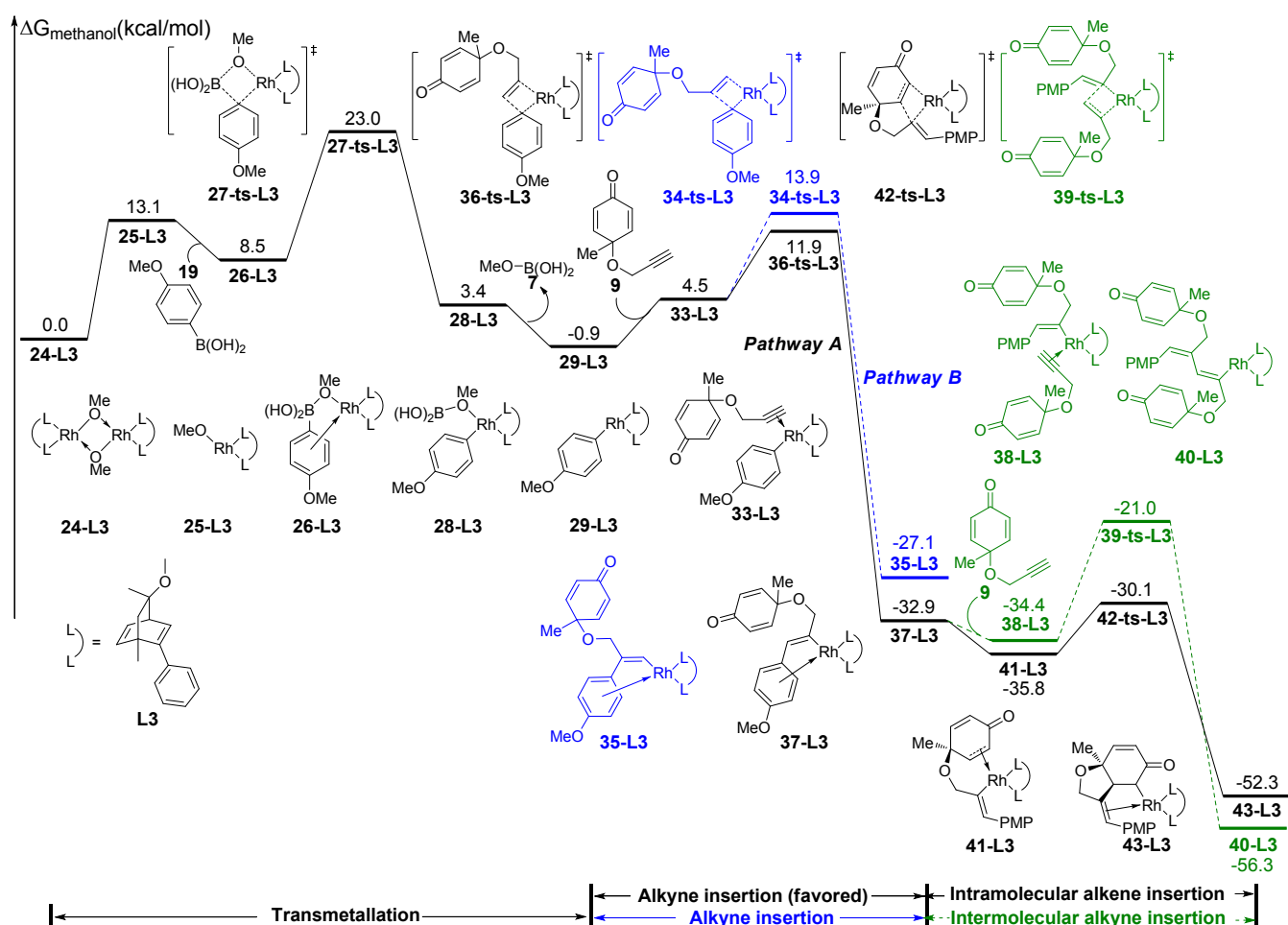
Figure S3. Free energy profile for rhodium-catalyzed synthesis of hydrobenzofurans with L3 ligand.
