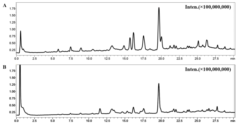
Fig. S1 The total ion chromatograms of methanolic extracts of DD (A) and DA (B)
