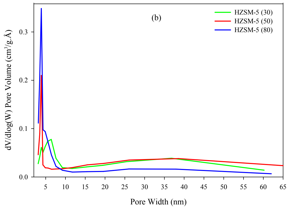
Fig. S1 Pore size distribution (from BJH desorption data): Halsey plot with Faas correction.
