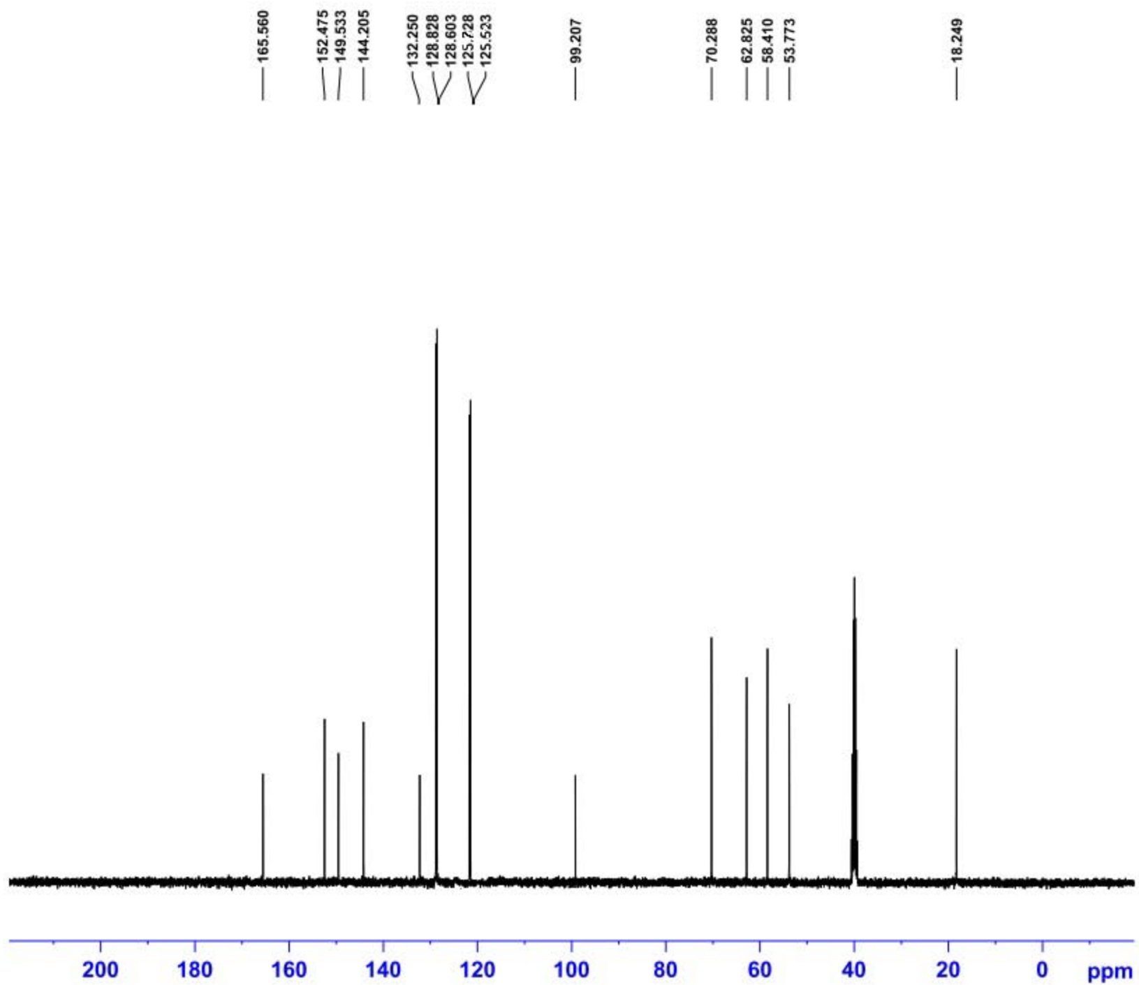
13C NMR 4-(4-chlorophenyl)-5-(2-methoxyethoxycarbonyl)-6-methyl-3,4-dihydropyrimidin-2(1H)-one (14u)
