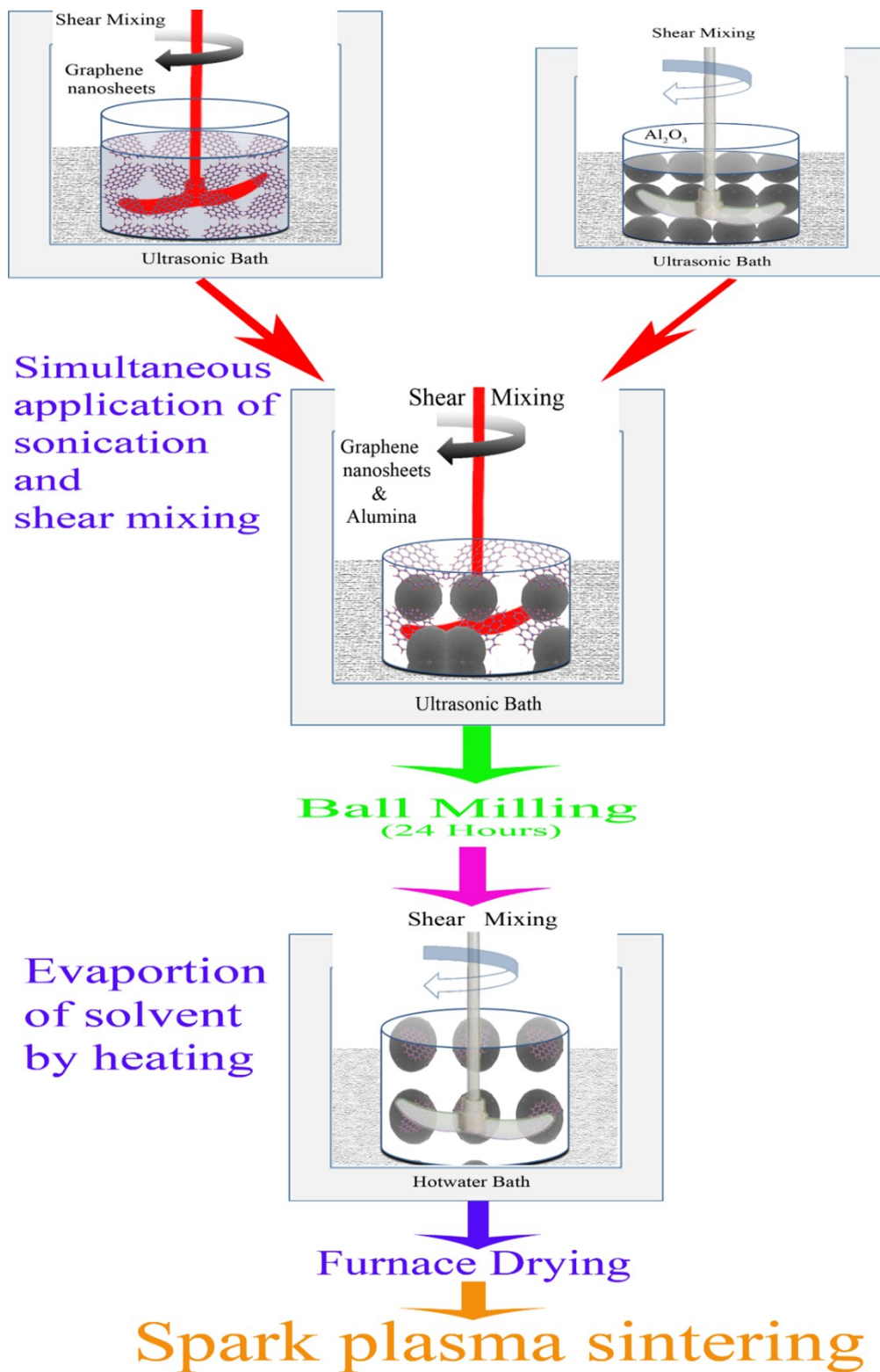
Figure S1. Schematic illustration of multistep processing for uniform mixing of graphene nanosheets in alumina powder
