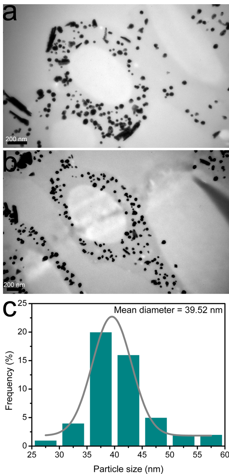
Figure S1. Cross-sectional TEM images of AuNPs-immobilized nanofibers with different magnification (reduced in 5mM \text{HAuCl}_4 solution) (a, b); the particle size distribution histogram (c)
