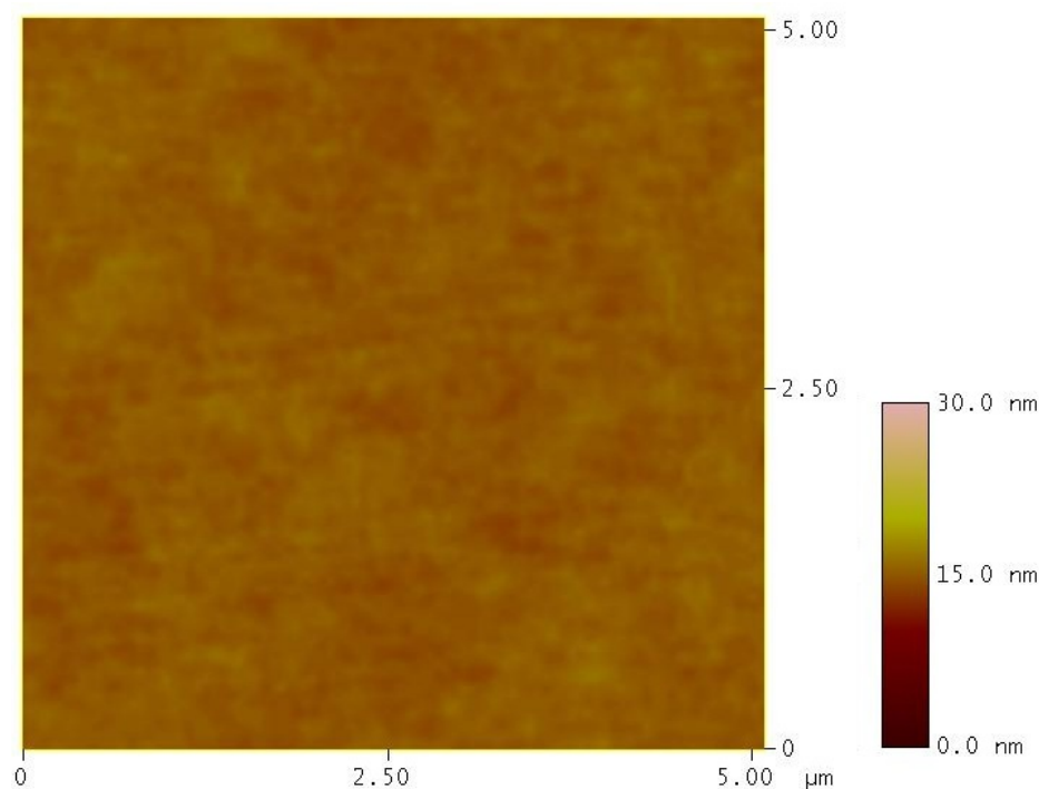
Fig. S1. AFM image of the cured PE-PMP film on a silicon wafer.
