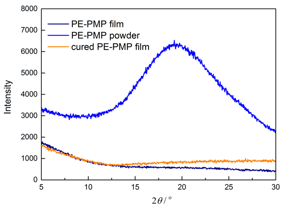
Fig. S2. X-ray diffraction (XRD) patterns of PE-PMP before and after postpolymerization.
