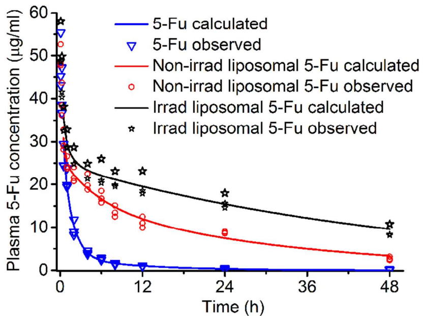
Supplementary Figure 1: Time-concentration curve of free and liposomal 5-Fu in IRC mice by PK software. 87x61mm (300 x 300 DPI)
