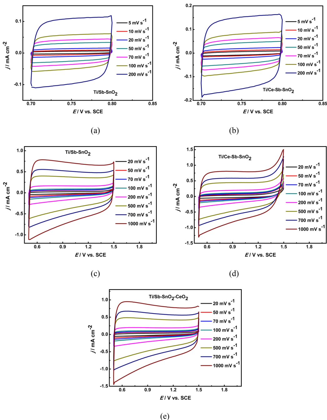
Fig. S1 Cyclic voltammograms at different sweep rates in 0.25 M Na 2 SO 4 solution: (a) and (b) between 0.7 and 0.8 V; (c), (d) and (e) between 0.5 and 1.5 V.
