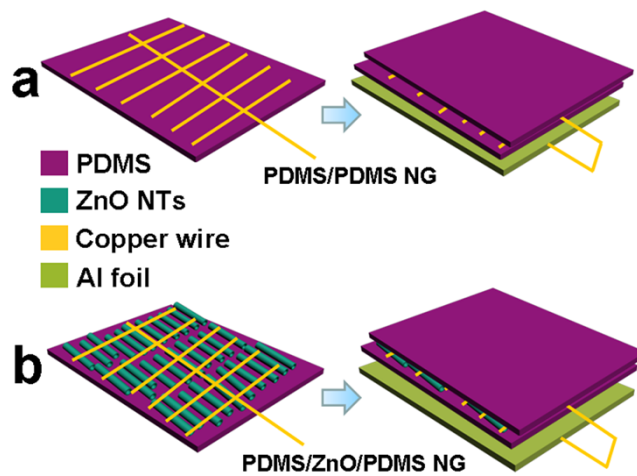
Fig. S1 The diagram of the fabrication of PDMS/PDMS NG (a) and PDMS/ZnO/PDMS NG (b)
