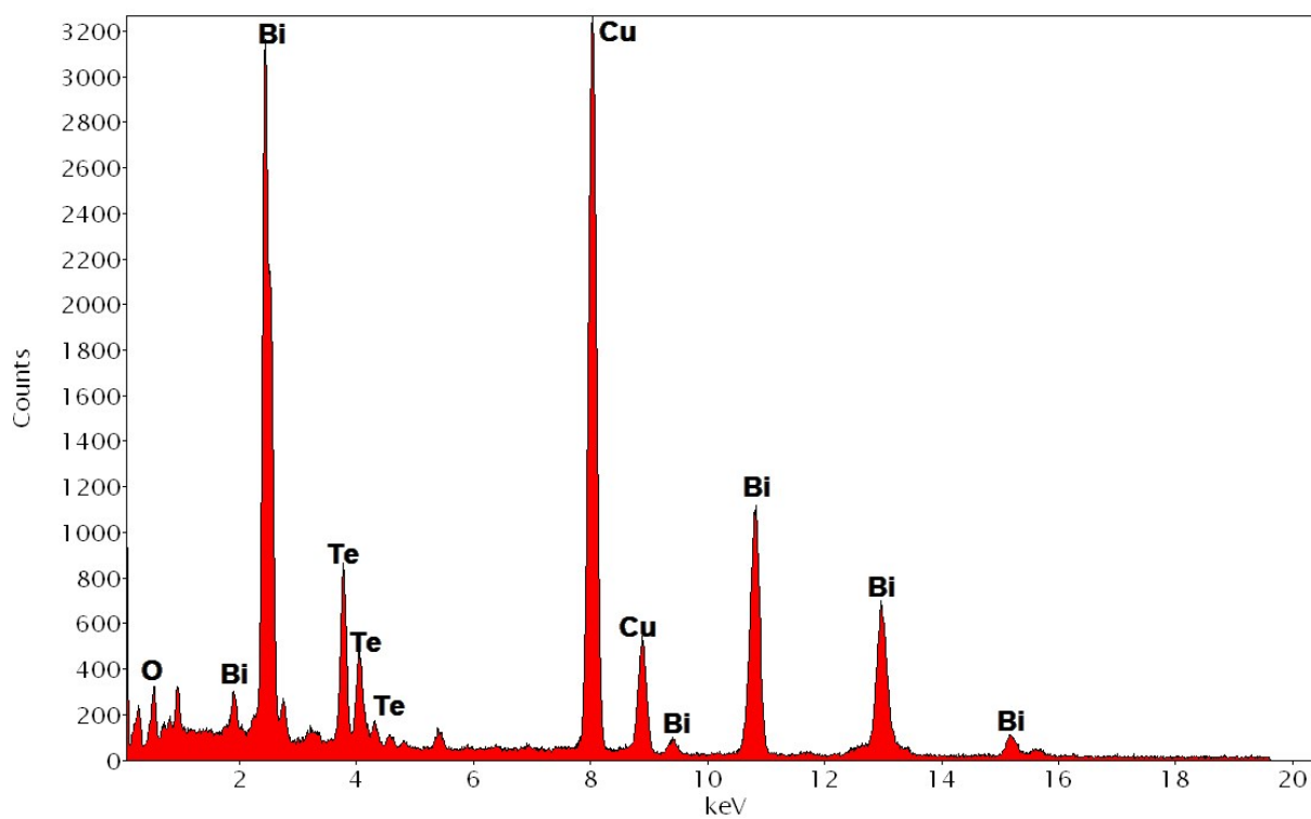
Figure S2. EDS image of PM-4
