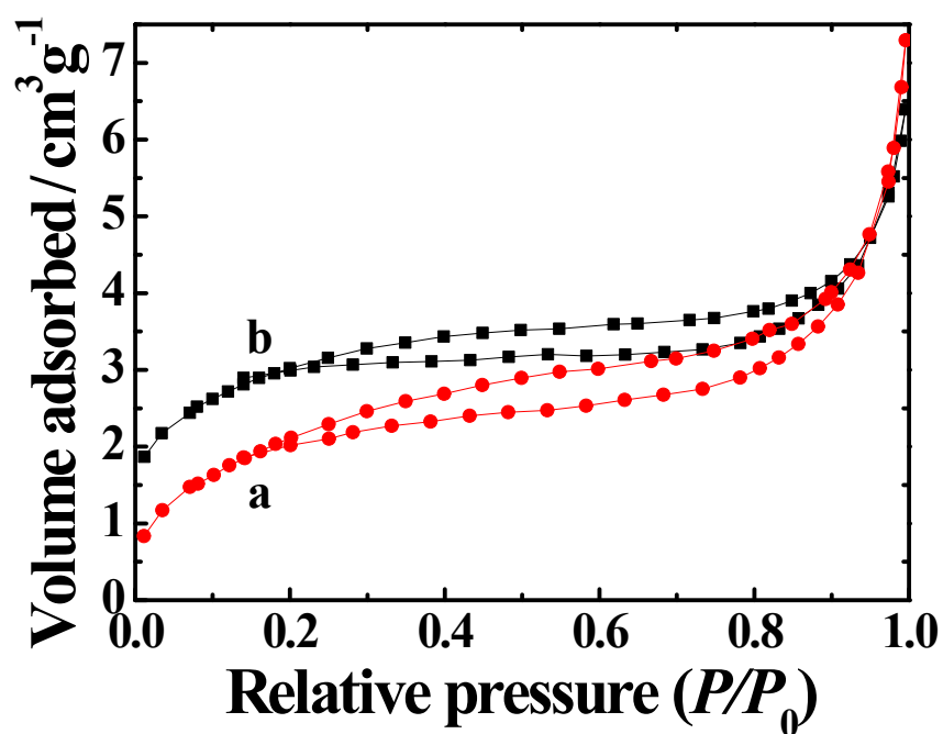
Fig. S1 N 2 adsorption-desorption isotherms of the samples synthesized in water/ethanol mixtures with ethanol volume ratios of 0 (a) and 25% (b).
