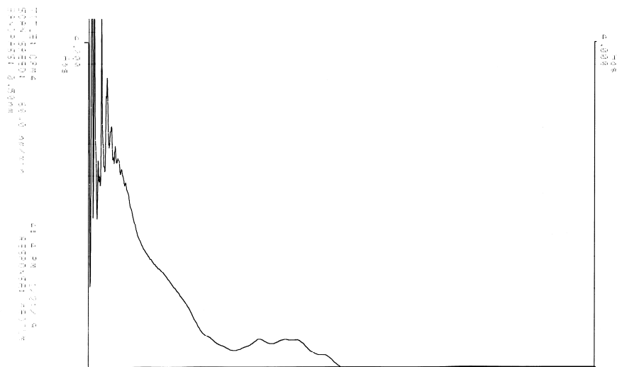
UV spectrum of fraction CPM-4
