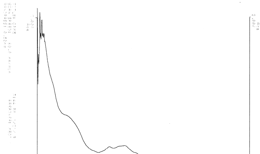
UV spectrum of fraction CPM-5
