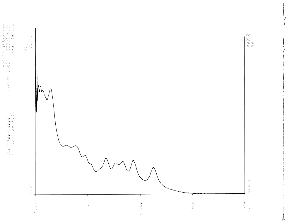
UV spectrum of fraction CPM-2
