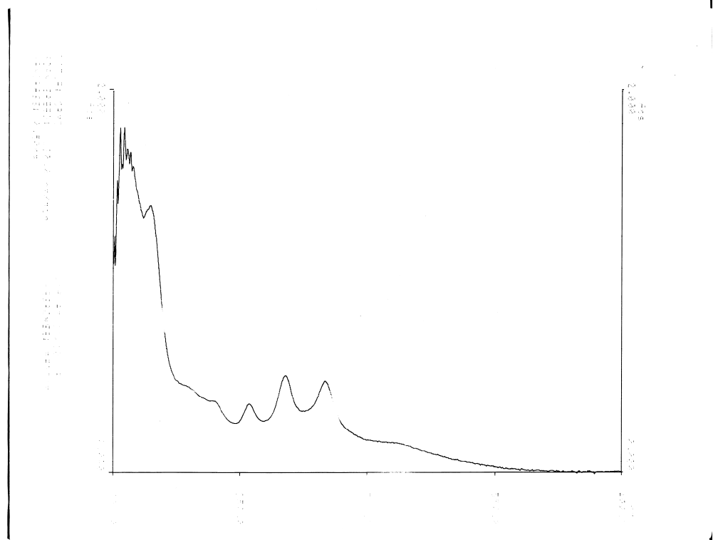
UV spectrum of fraction CPM-3
