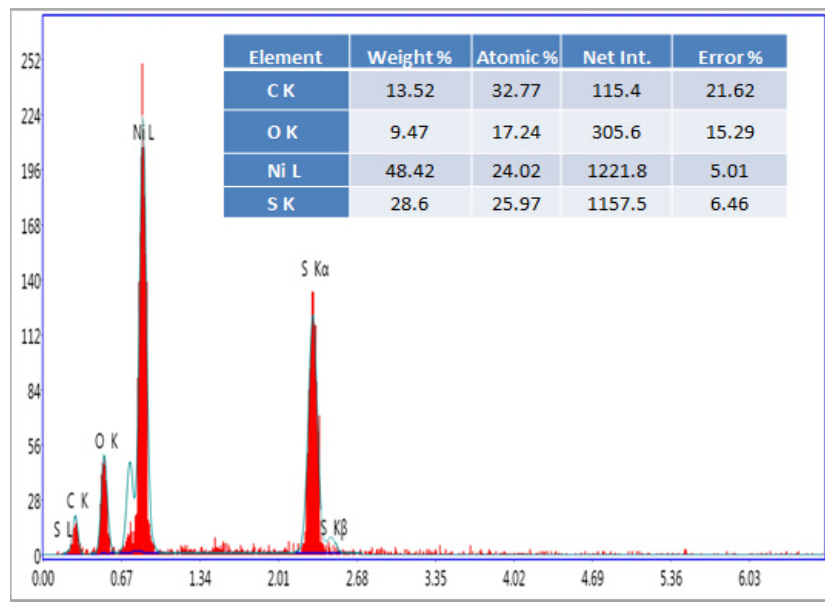
Fig. S2 Element ratio of Ni, S and C in NiS/SWNTs composite
