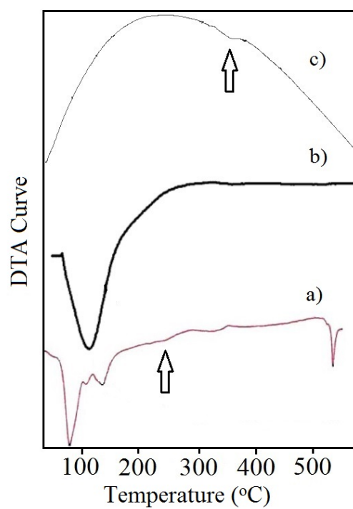
SM 1. DTA curves for a) \text{PMo}_{11} , b) \text{H}\beta and c) 30% \text{PMo}_{11}/\text{H}\beta .
