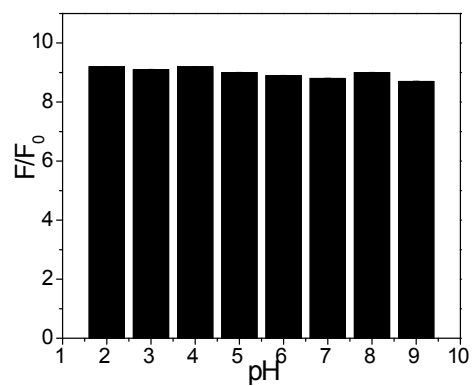
Fig. S1. Effects of Ph on the F/F_0 value of sensor system. Conditions: Hg^{2+} , 0.8 nM.
