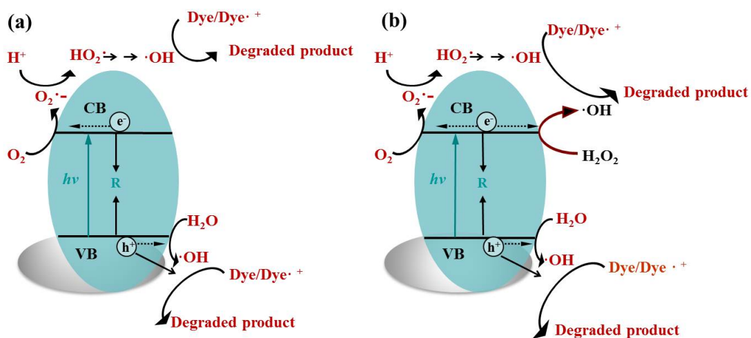
Fig. S2 Proposed mechanisms of t-Se NRs in the visible-SeNRs-HCl (a) and visible-SeNRs-H 2 O 2 (b) degradation of MO.
