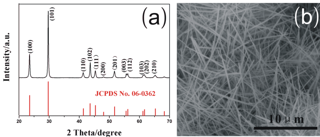
Fig. S1 XRD patterns (a) and SEM (b) image of the spent t-Se NRs after photocatalytic in the visible-Se NRs-H 2 O 2 systems
