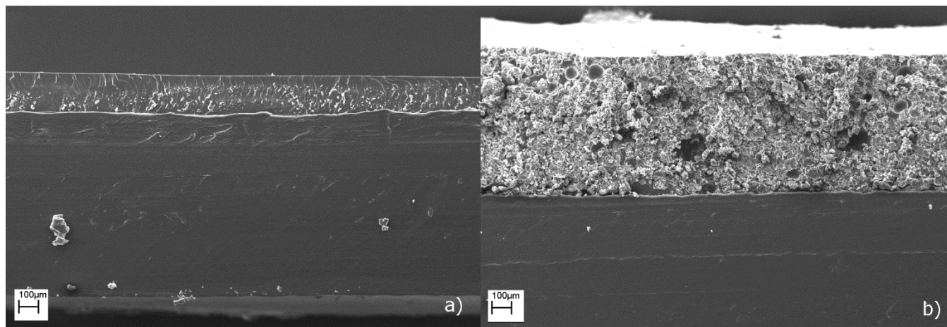
Figure. SEM micrographs of PA 10,10 coated with UV-curable resin (a) and UV-curable resin + ammonium polyphosphate (b)
