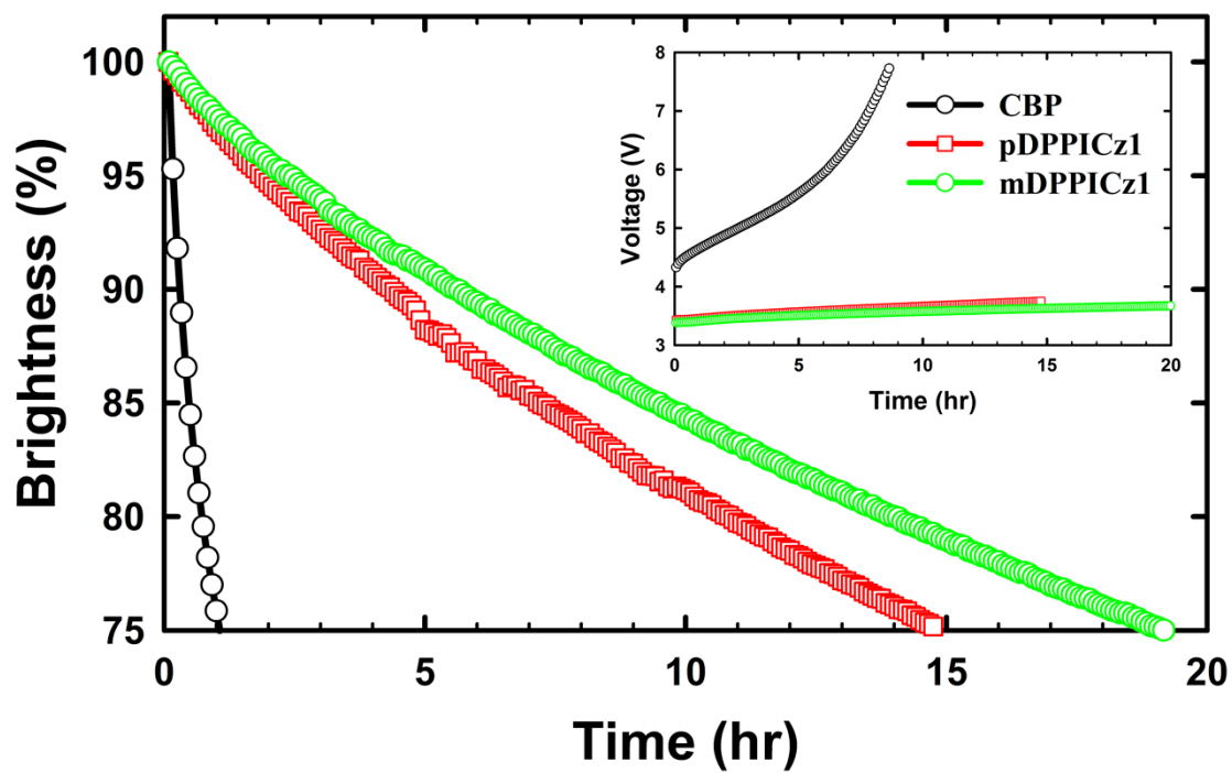
Fig. S1. Operational lifetime curves of pDPPICz1, mDPPICz1 and CBP based OLEDs.
