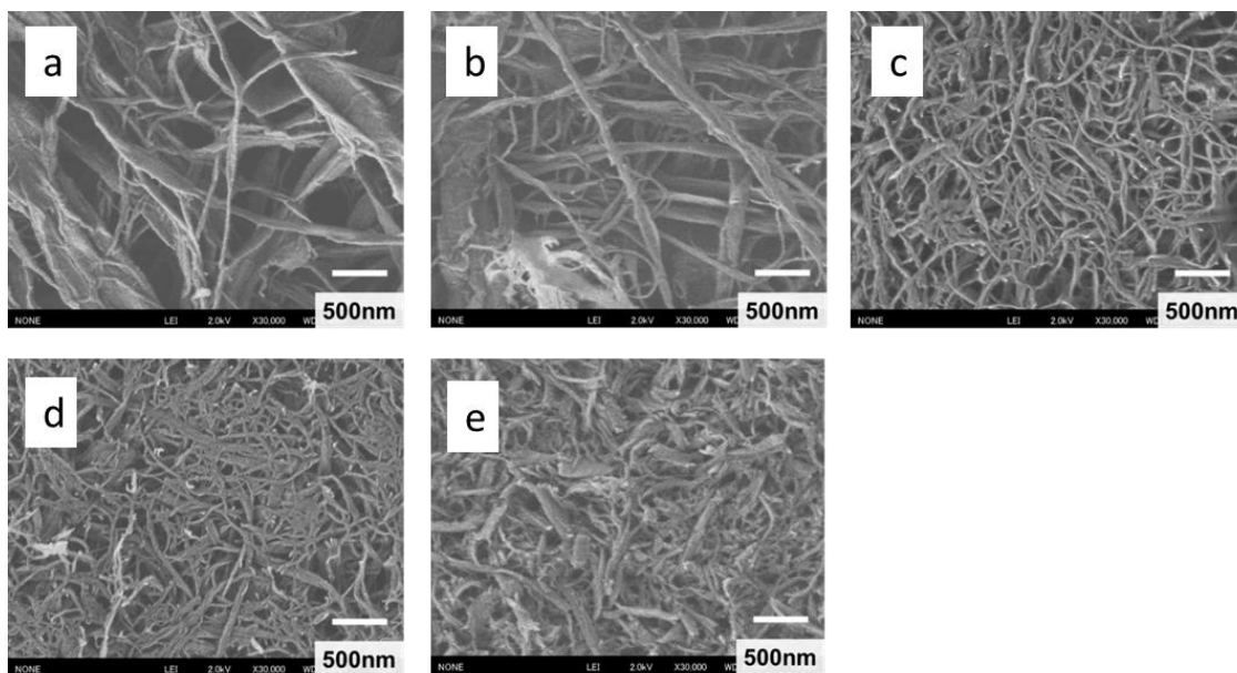
Figure S2. FE-SEM images poly( p -phenylene benzobisoxazole) nanofibers with different alkaline hydrolysis times of (a) 3 h, (b) 12 h, (c) 1 week, (d) 2 weeks, and (e) 3 weeks.
