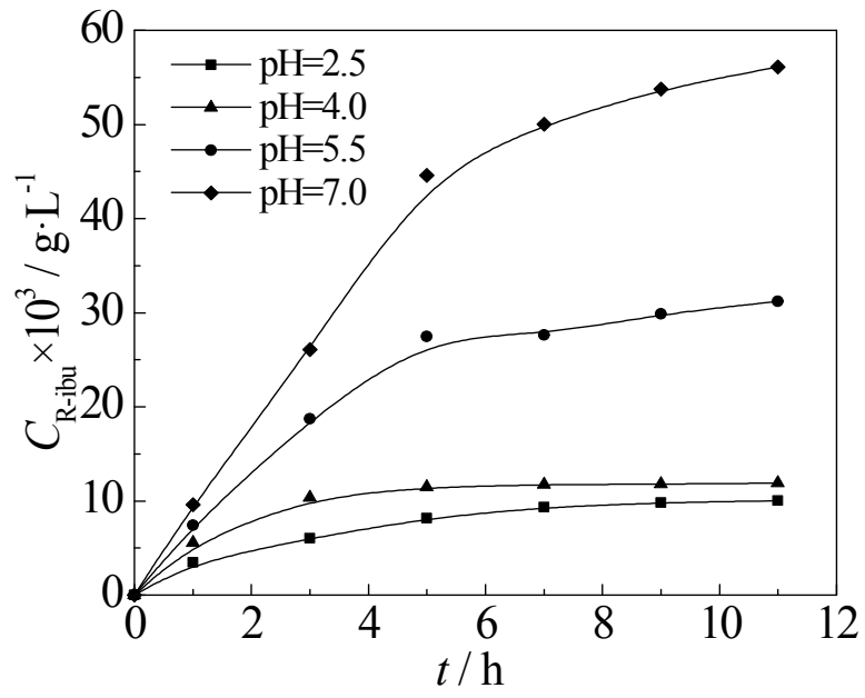
Fig.S1 Influence of pH in stripping phase on the concentration of R -ibuprofen.
