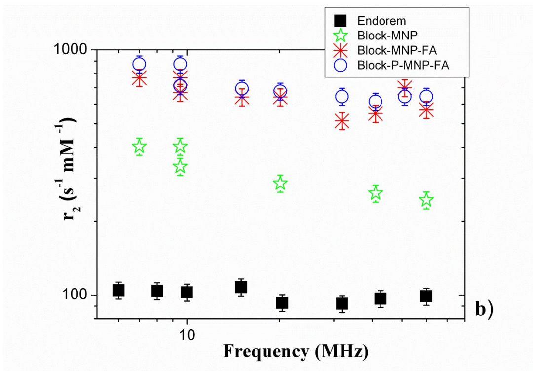
Figure SI2. Longitudinal ( r_1 ) and Transverse ( r_2 ) relaxivities ( L \cdot \text{mmol}^{-1} \cdot \text{sec}^{-1} ) of Block-MNP, Block-MNP-FA and Block-P-MNP-FA samples compared to Endorem ®
