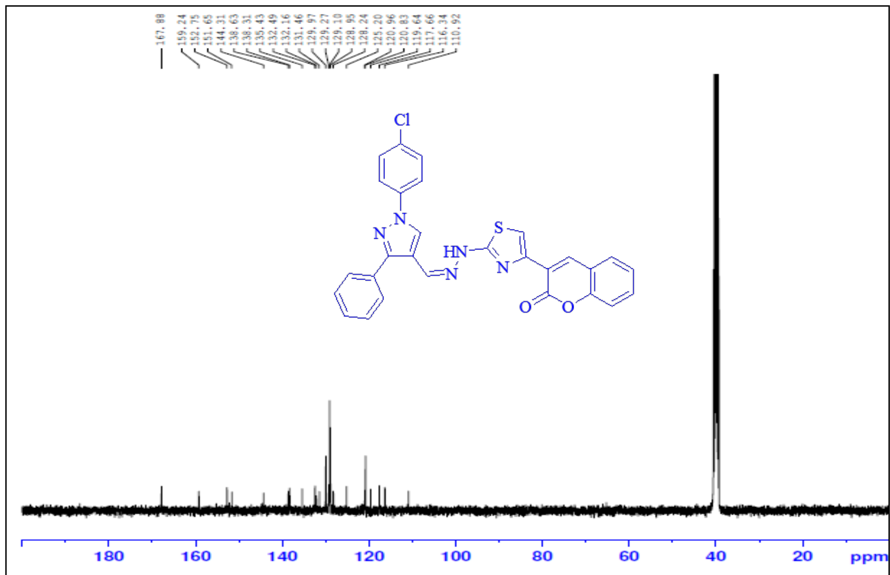
13 C NMR spectrum of 10b- DMSO-d 6 -100 MHz
