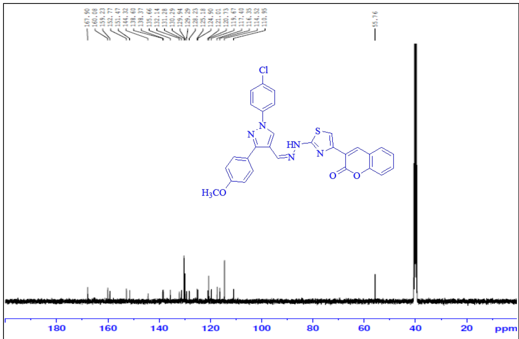
13 C NMR spectrum of 10f- DMSO-d 6 -100 MHz
