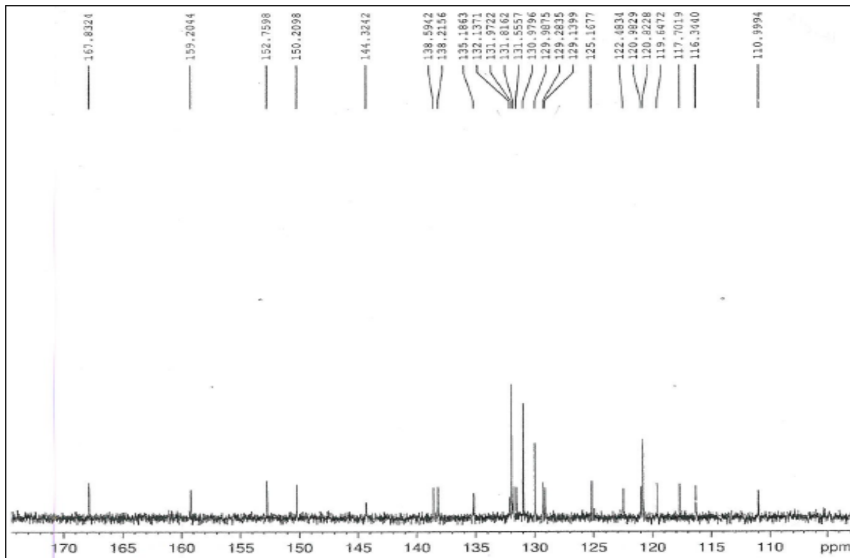
Expanded spectrum of 10j ( ^{13}\text{C} NMR)
