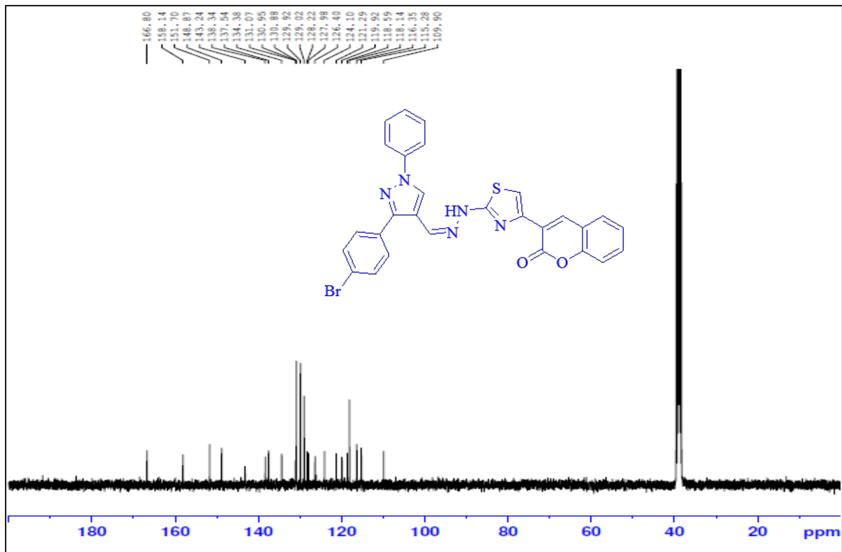
13 C NMR spectrum of 10i- DMSO-d 6 -100 MHz
