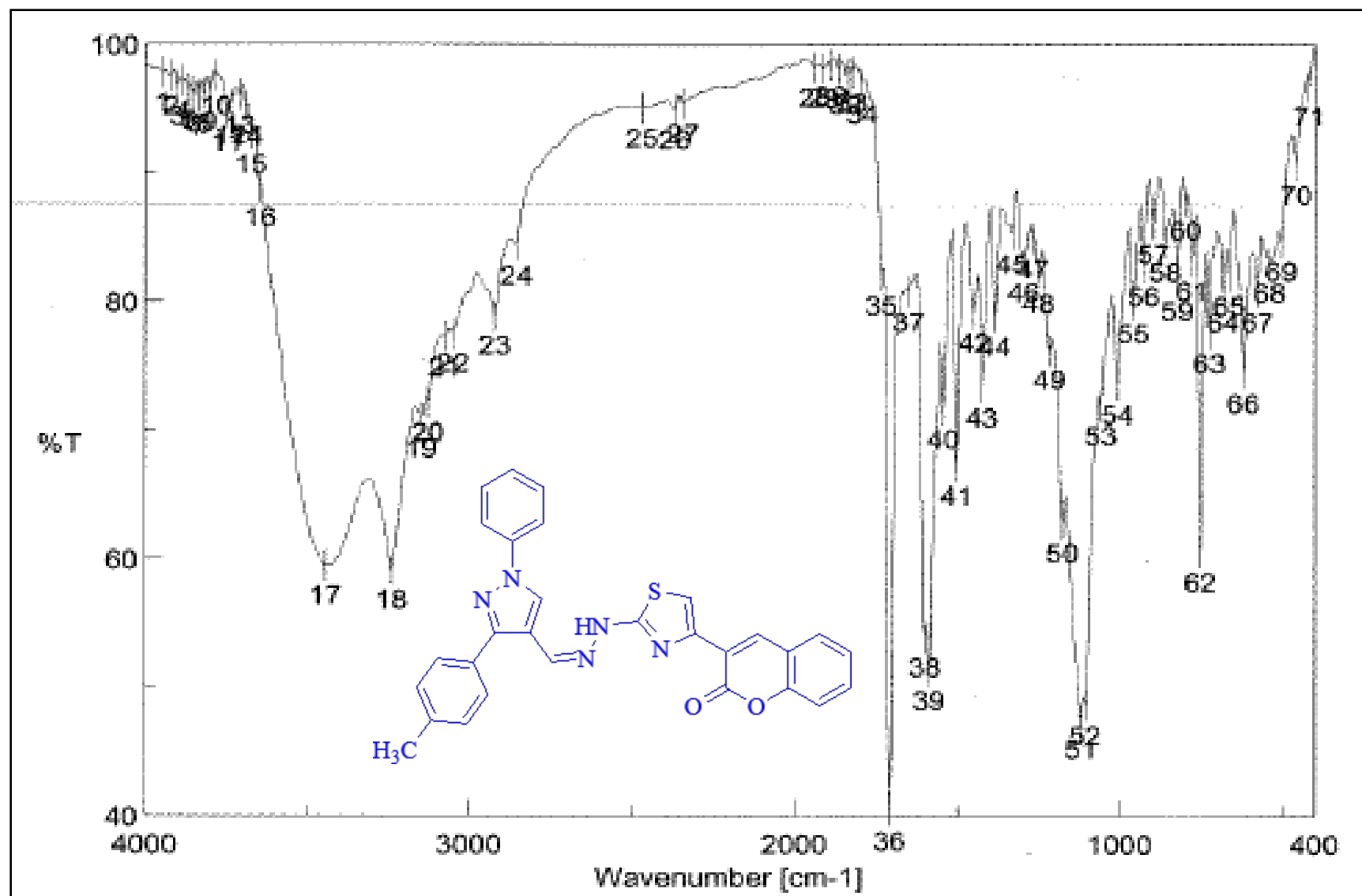
IR spectrum of 10c
