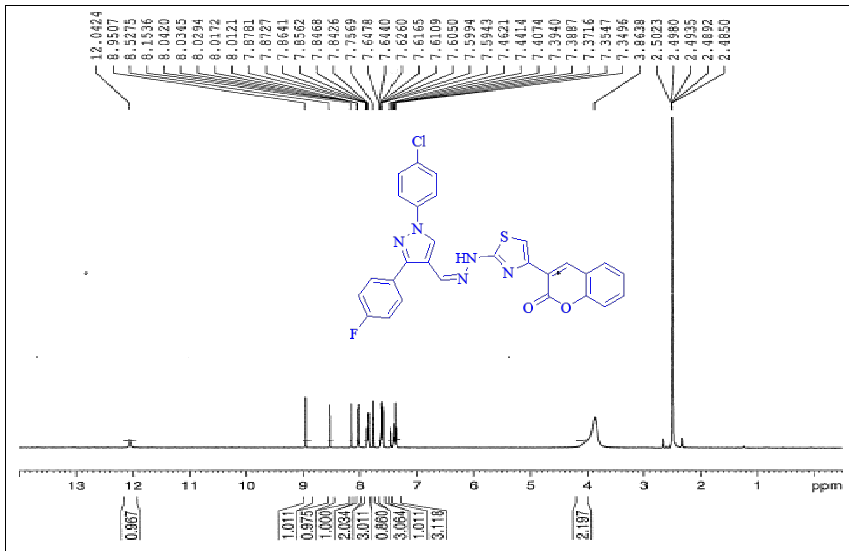
1 H NMR spectrum of 10l-DMSO-d 6 -400 MHz
