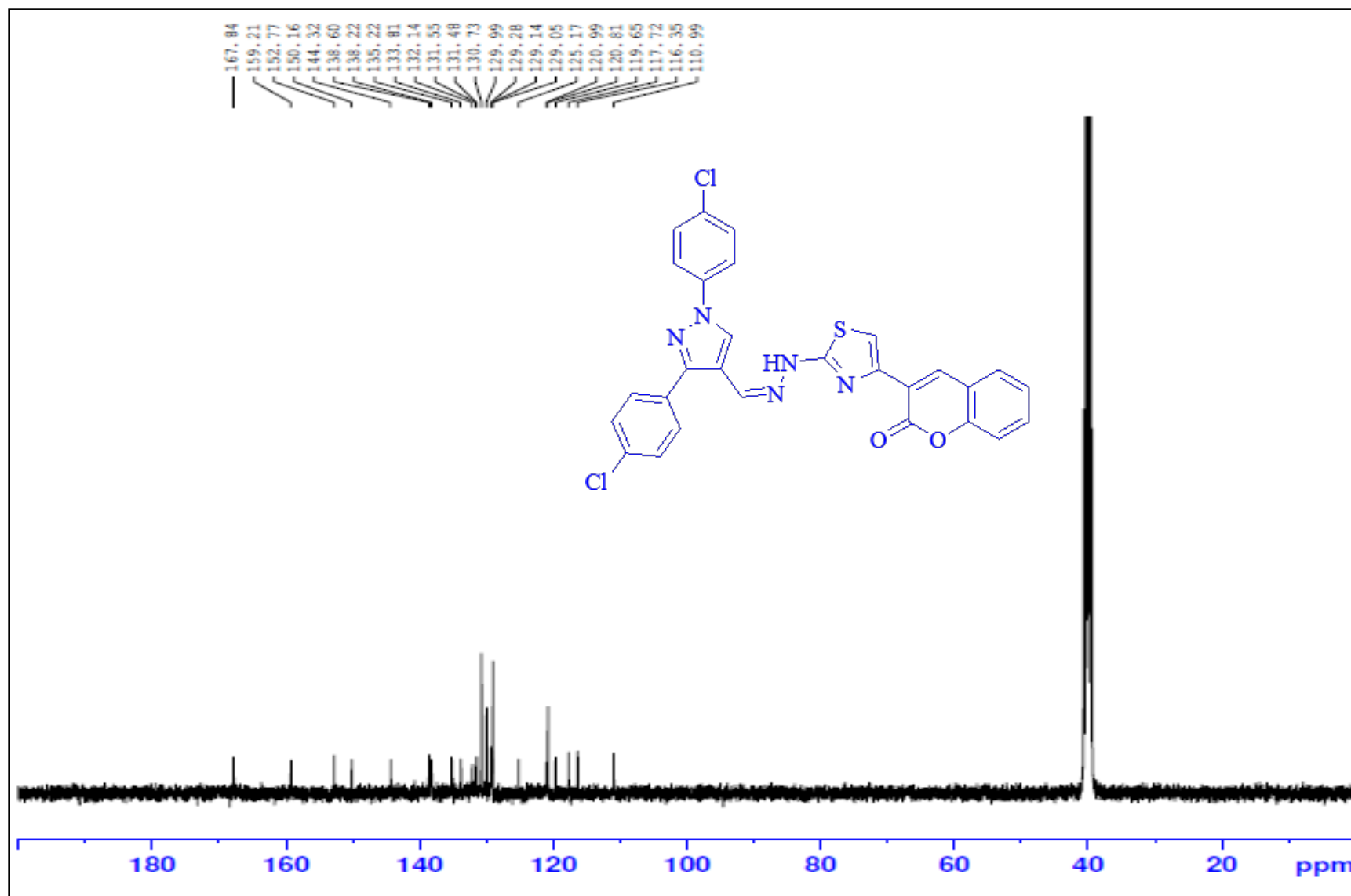
13 C NMR spectrum of 10h- DMSO-d 6 -100 MHz
