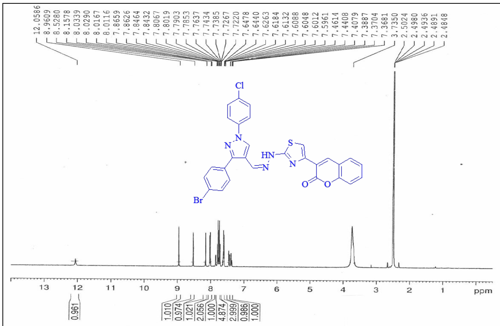
1 H NMR spectrum of 10j-DMSO-d 6 -400 MHz
