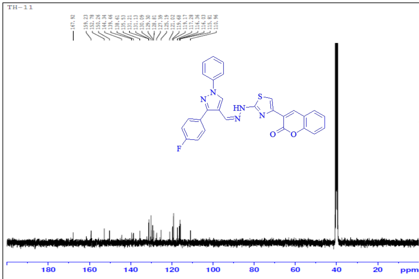
13 C NMR spectrum of 10k- DMSO-d 6 -100 MHz
