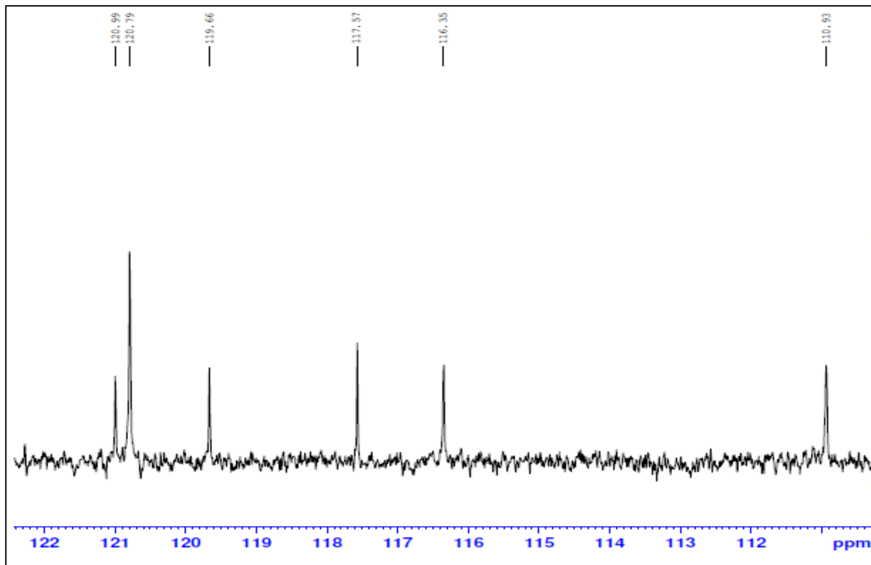
Expanded spectrum of 10d ( ^{13}\text{C} NMR)
