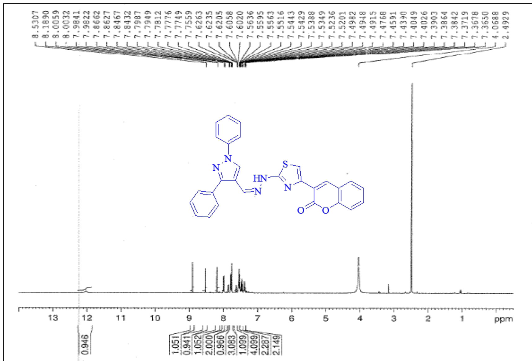
1 H NMR spectrum of 10a-DMSO-d 6 -400 MHz
