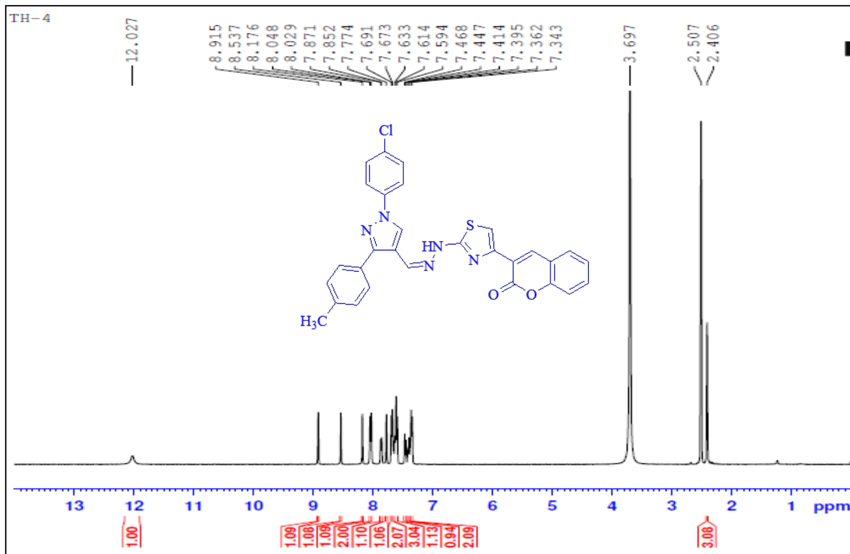
1 H NMR spectrum of 10d-DMSO-d 6 -400 MHz
