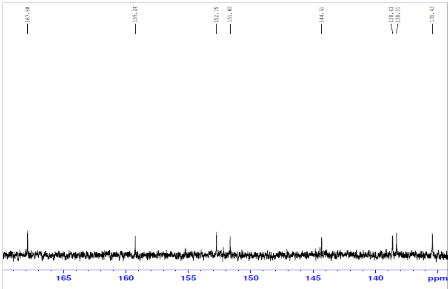
Expanded spectrum of 10b ( ^{13}\text{C} NMR)
