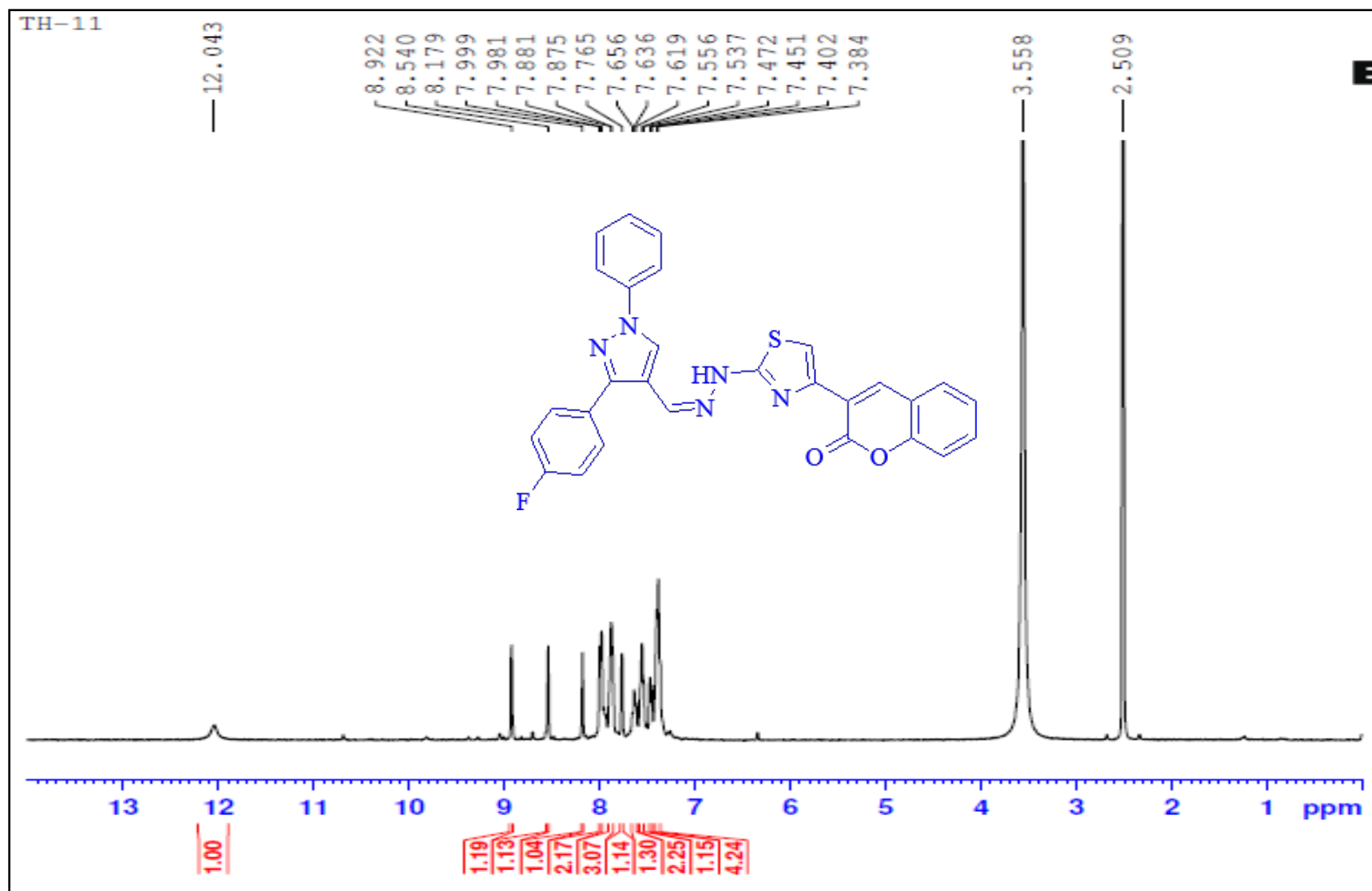
1 H NMR spectrum of 10k-DMSO-d 6 -400 MHz
