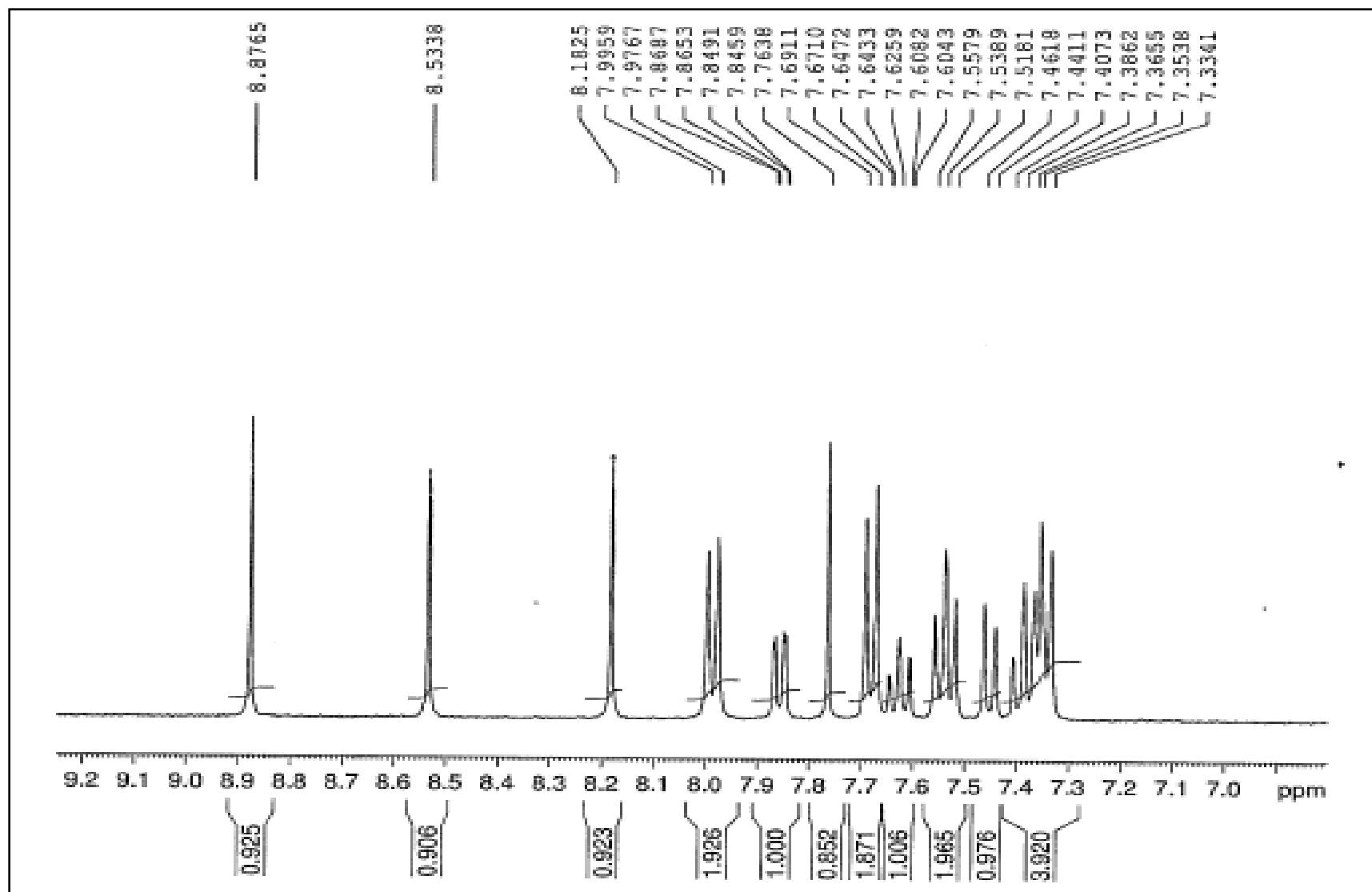
Expanded spectrum of 10c ( ^1\text{H} NMR)
