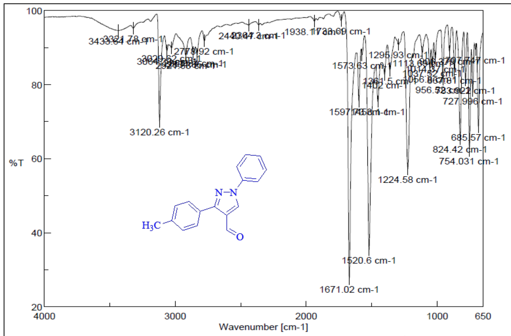
IR spectrum of 4c
