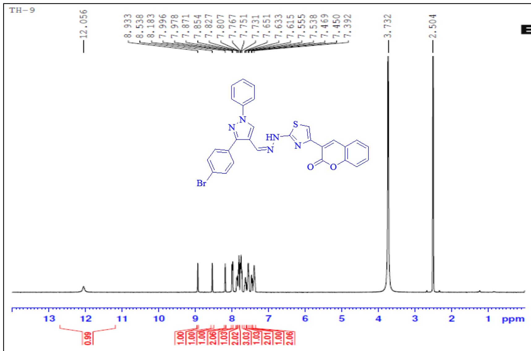
1 H NMR spectrum of 10i-DMSO-d 6 -400 MHz
