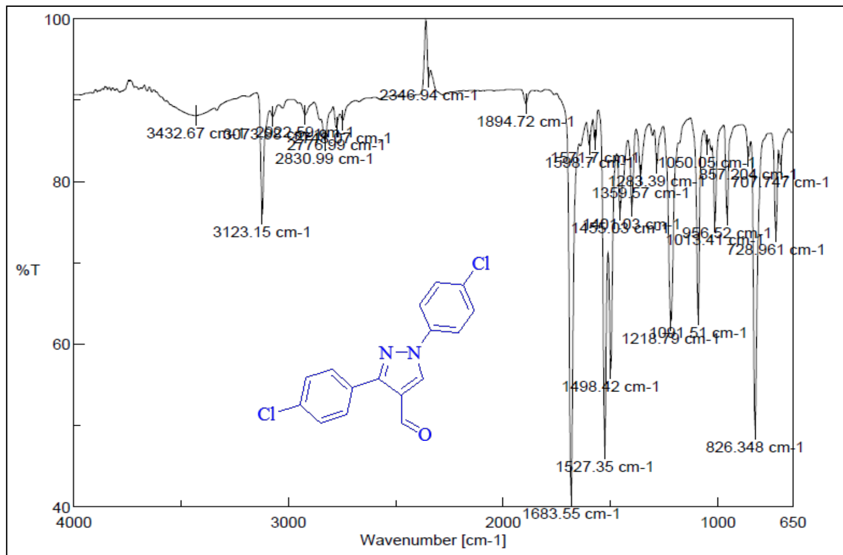
IR spectrum of 4h
