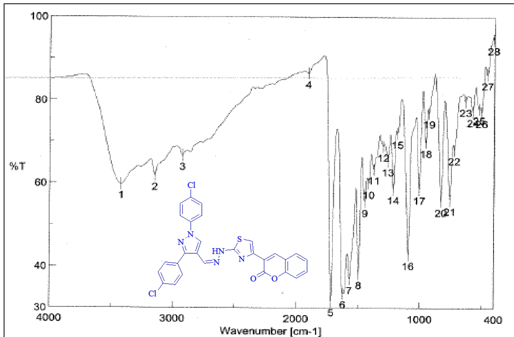
IR spectrum of 10h
