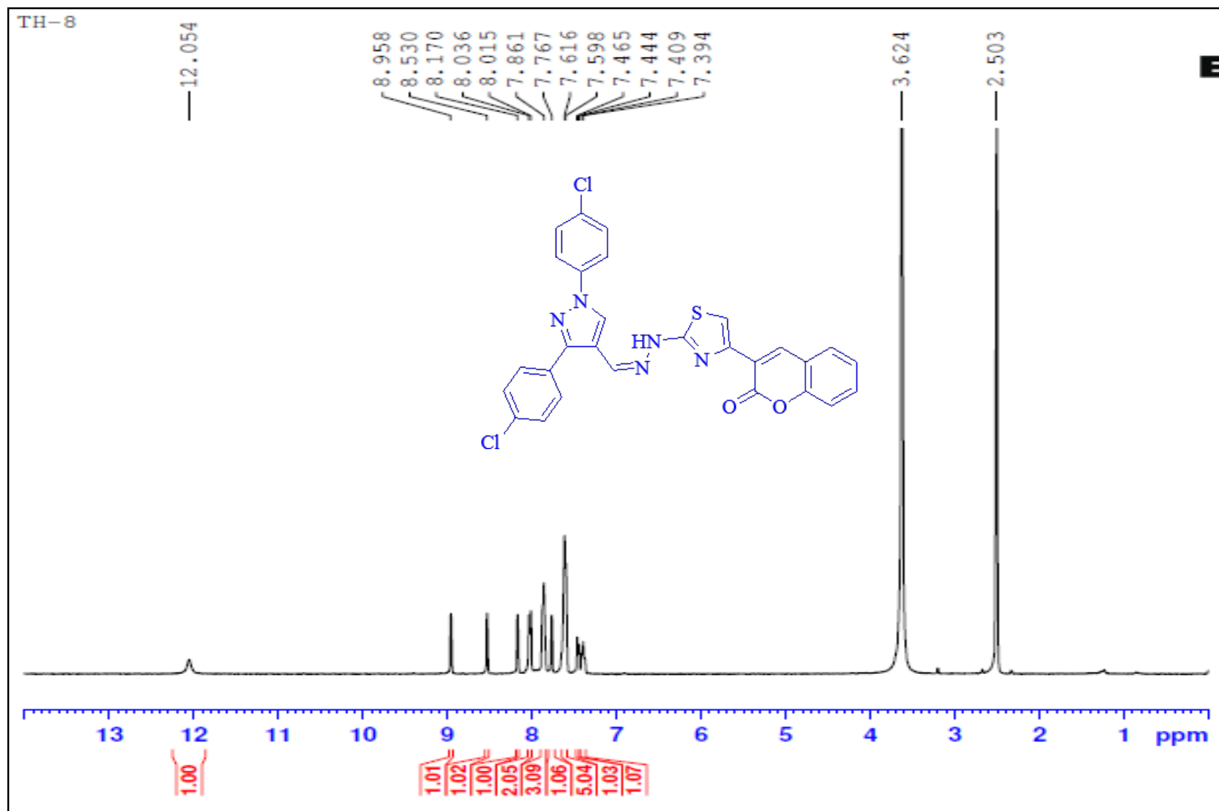
1 H NMR spectrum of 10h-DMSO-d 6 -400 MHz
