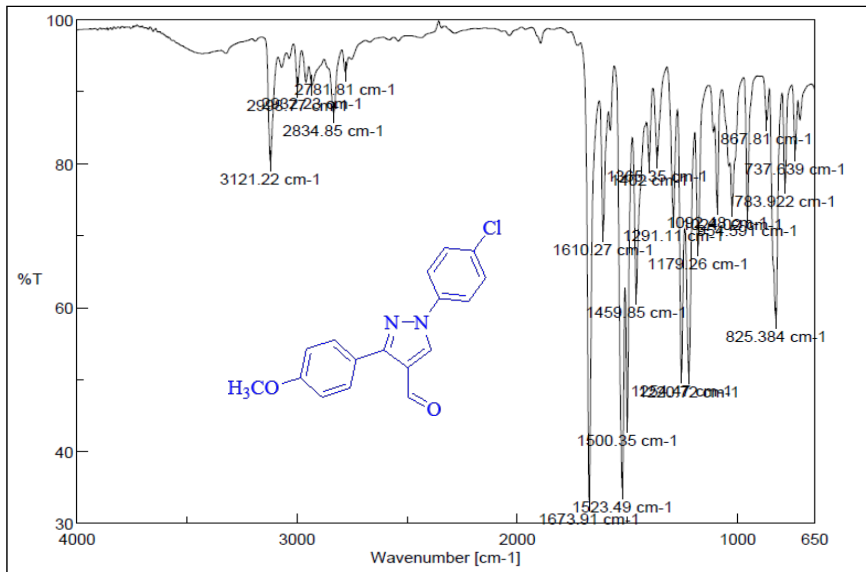
IR spectrum of 4f
