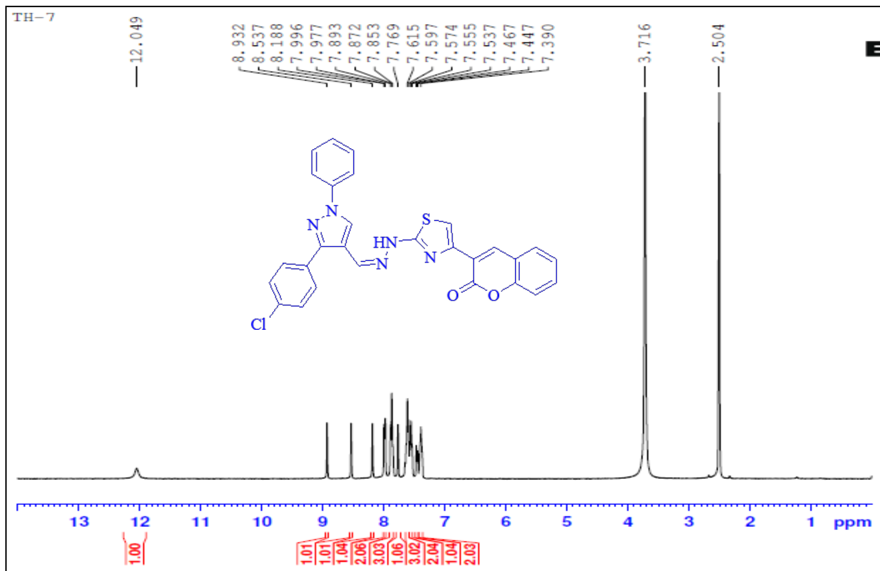
1 H NMR spectrum of 10g-DMSO-d 6 -400 MHz
