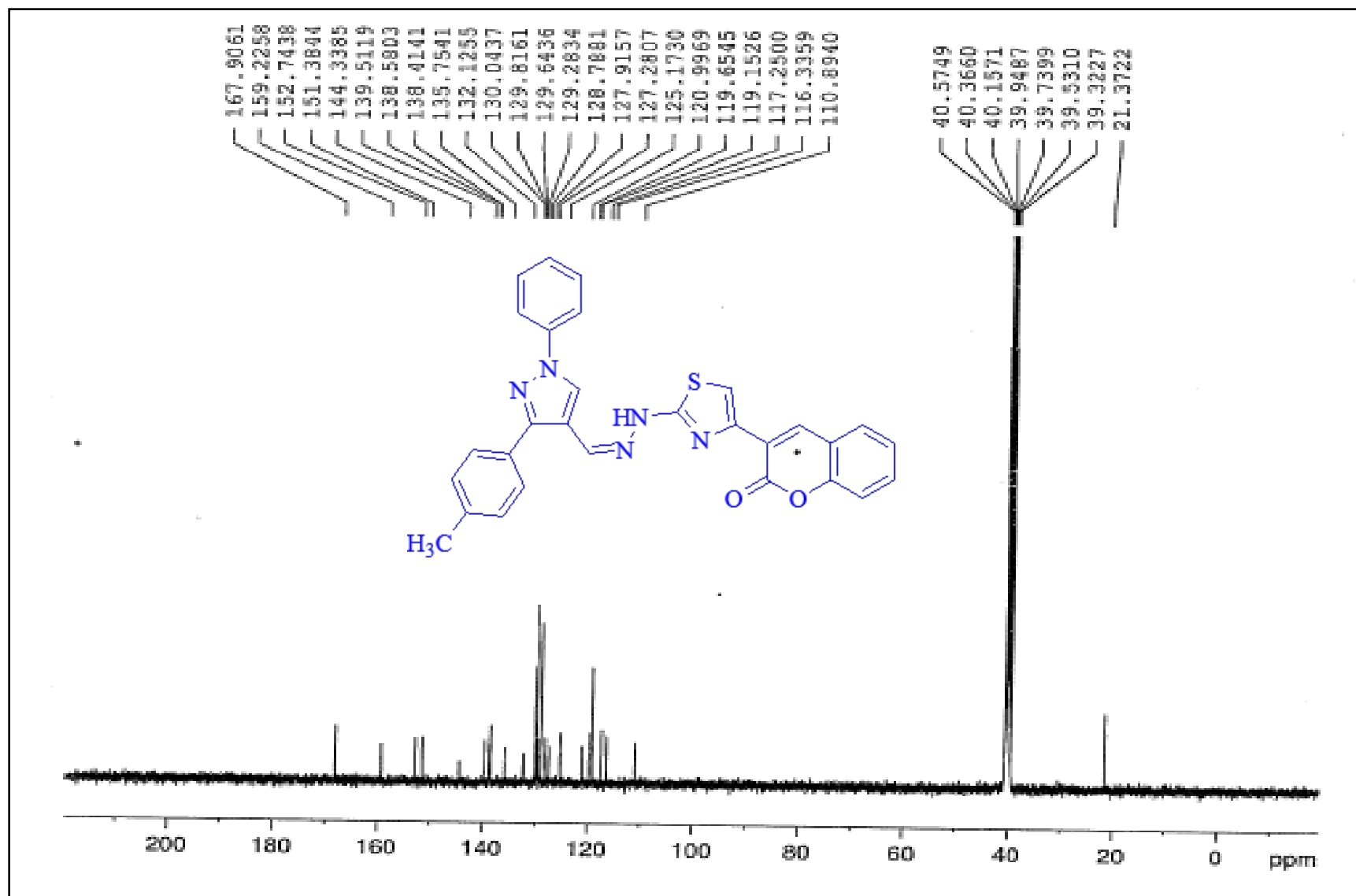
13 C NMR spectrum of 10c- DMSO-d 6 -100 MHz
