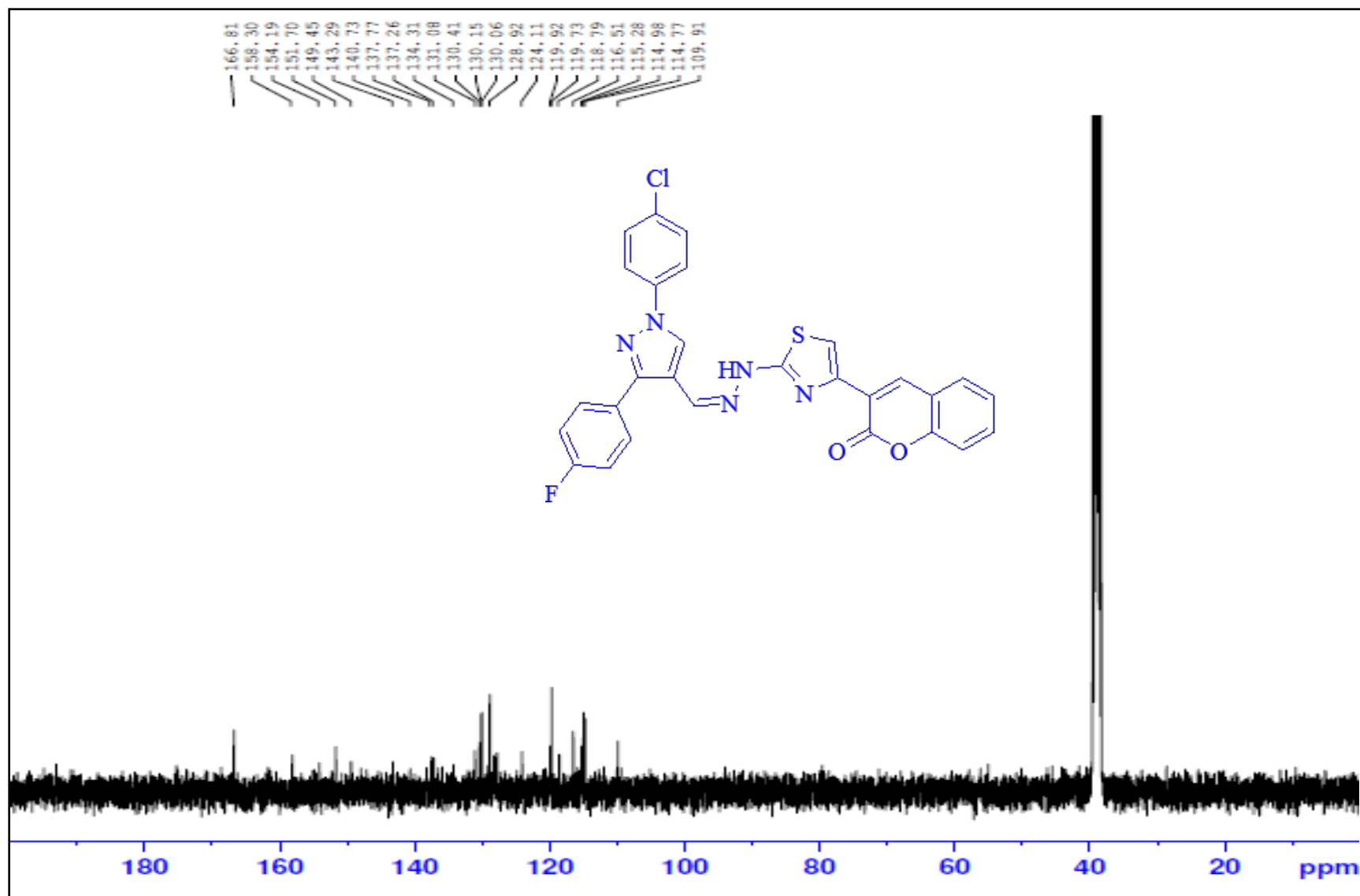
13 C NMR spectrum of 10l- DMSO-d 6 -100 MHz
