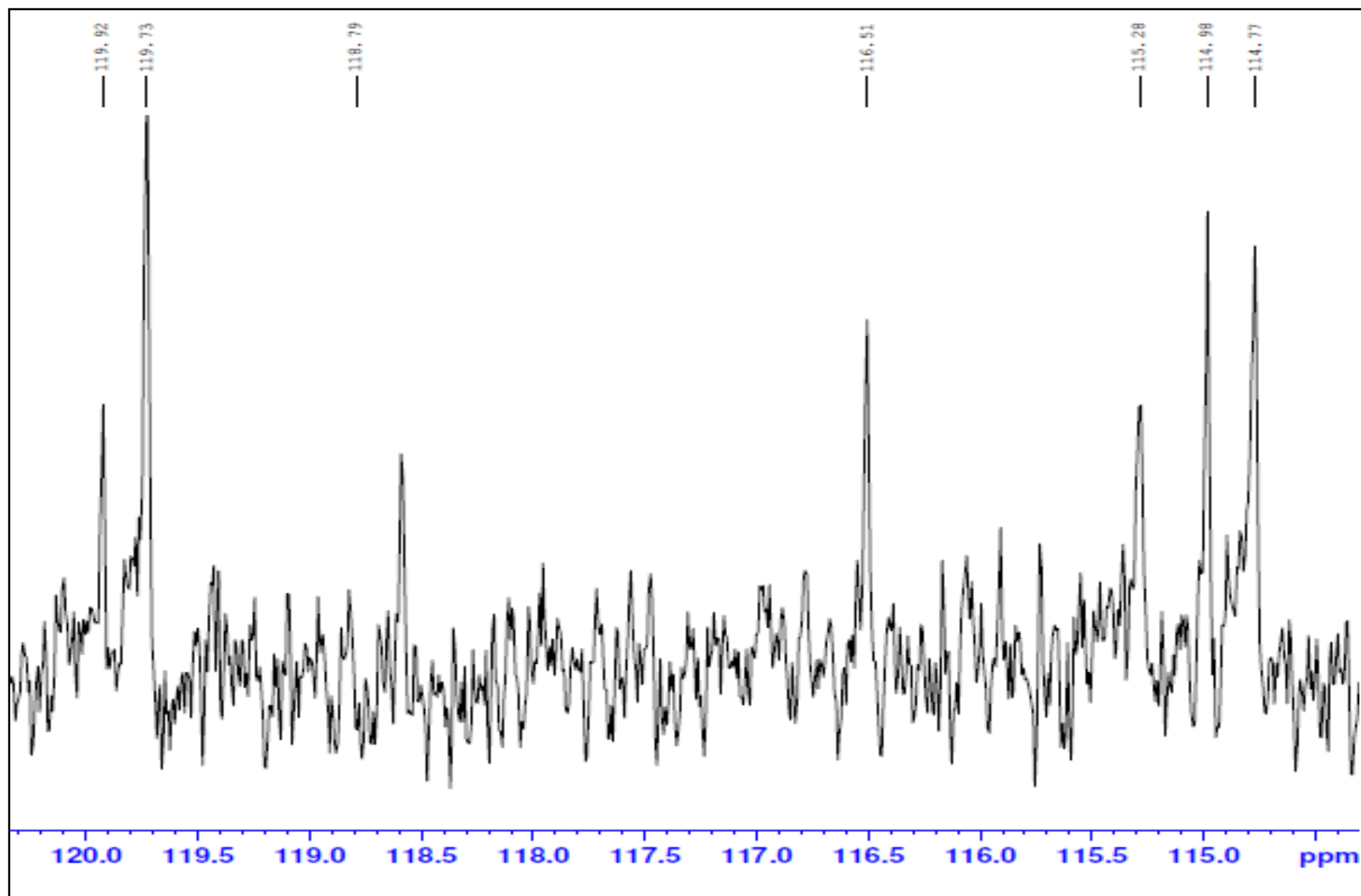
Expanded spectrum of 10l ( ^{13}\text{C} NMR)
