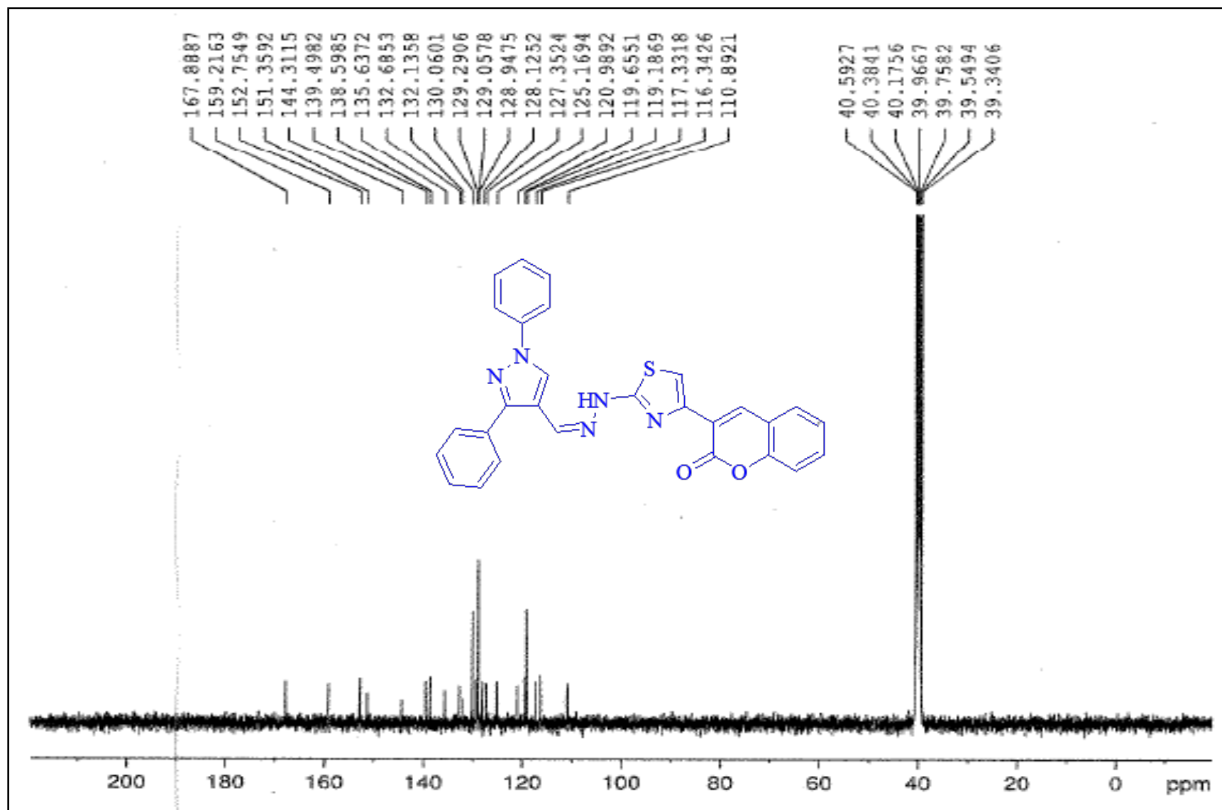
13 C NMR spectrum of 10a- DMSO-d 6 -100 MHz
