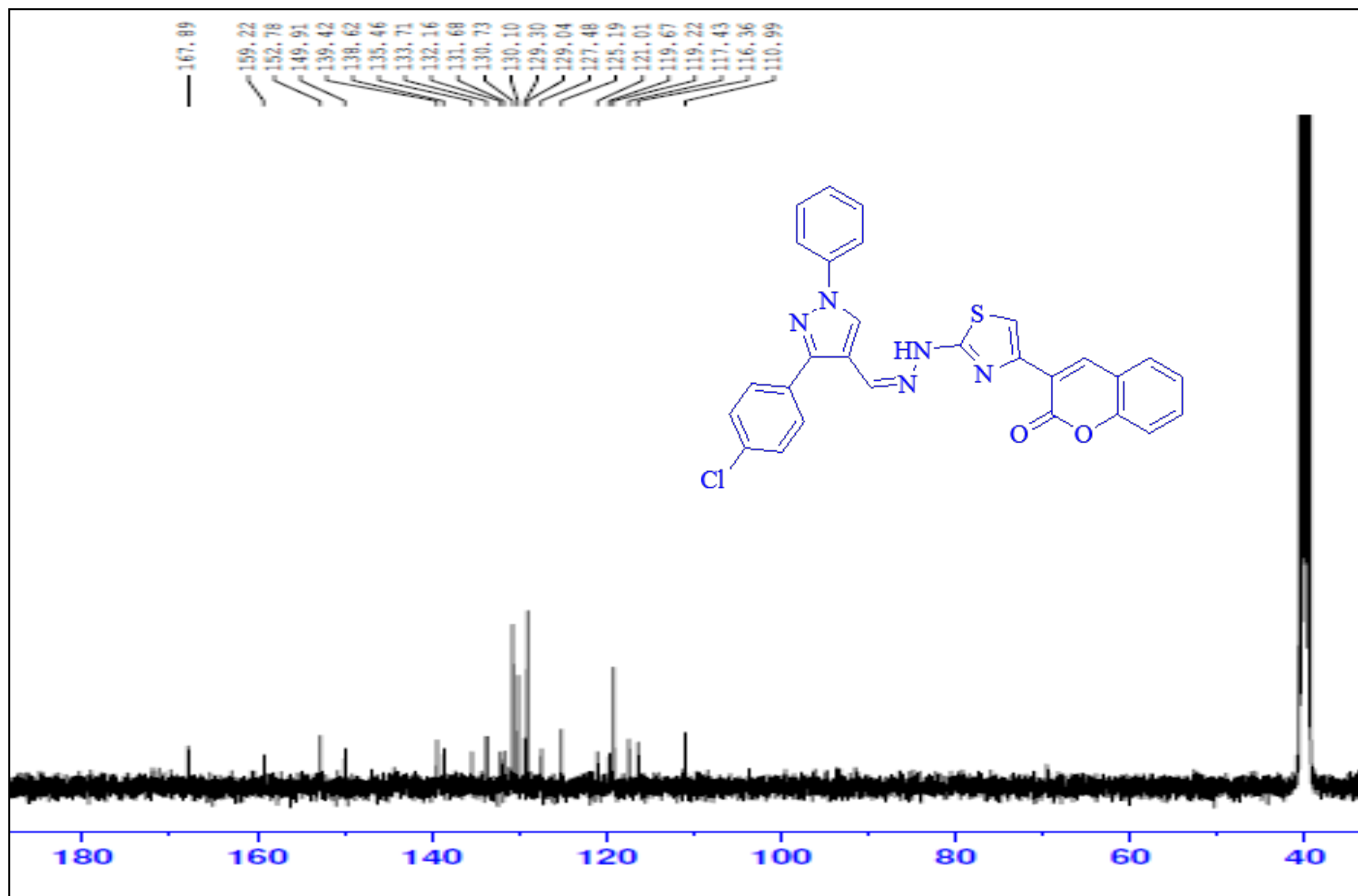
13 C NMR spectrum of 10g- DMSO-d 6 -100 MHz
