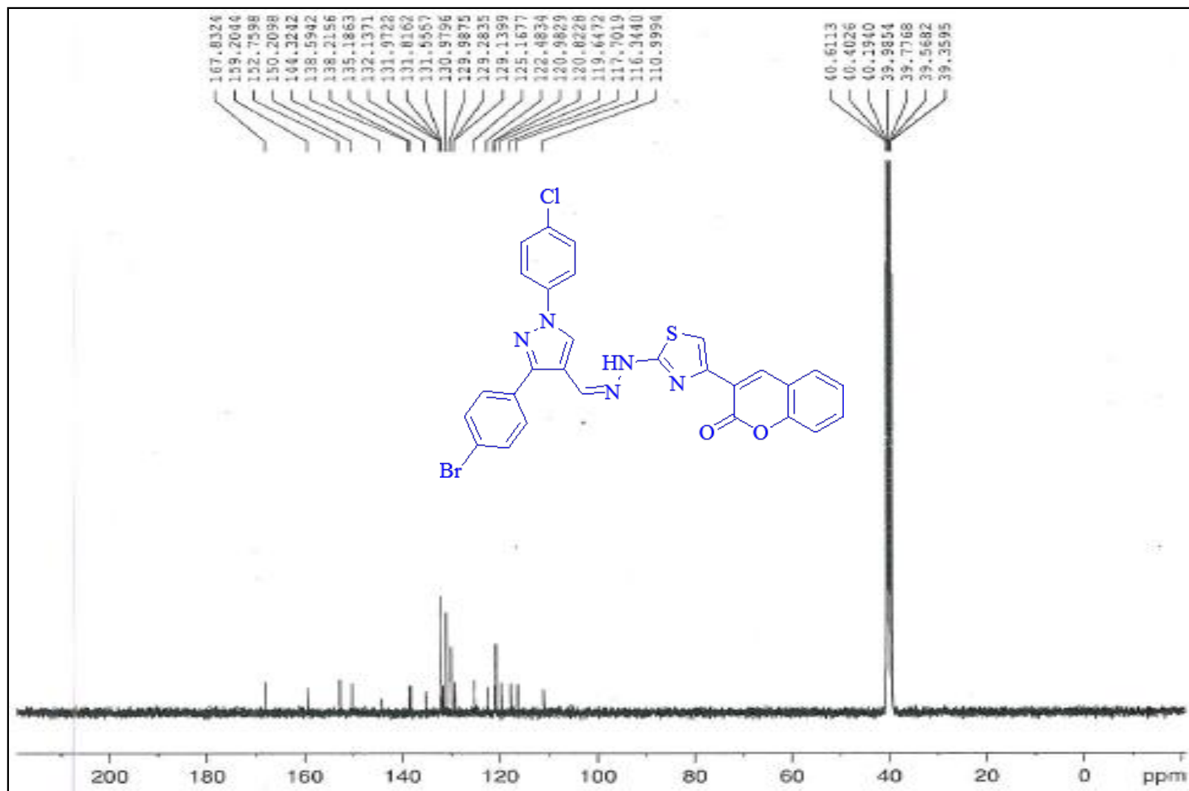
13 C NMR spectrum of 10j- DMSO-d 6 -100 MHz
