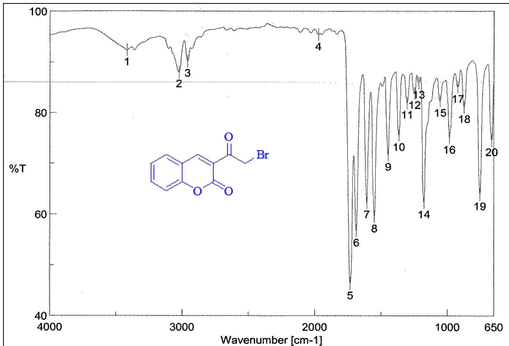
IR spectrum of 8
