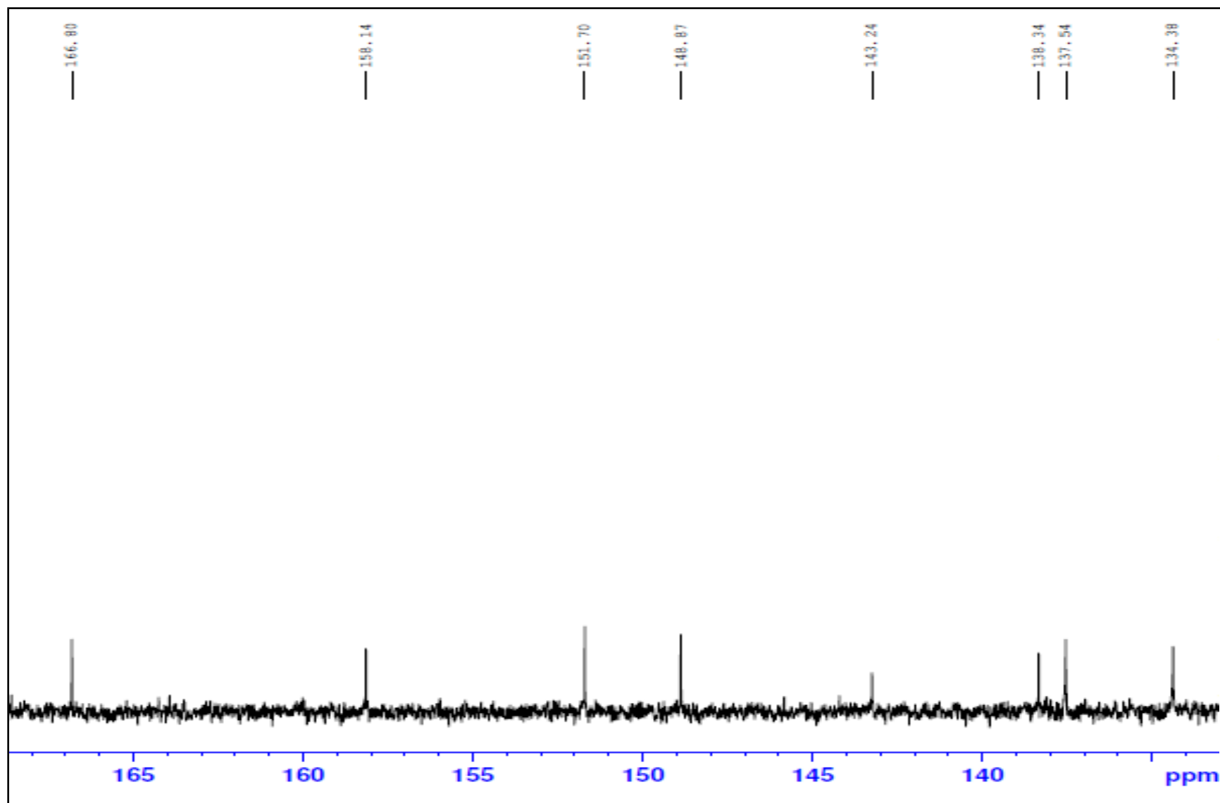
Expanded spectrum of 10i ( ^{13}\text{C} NMR)
