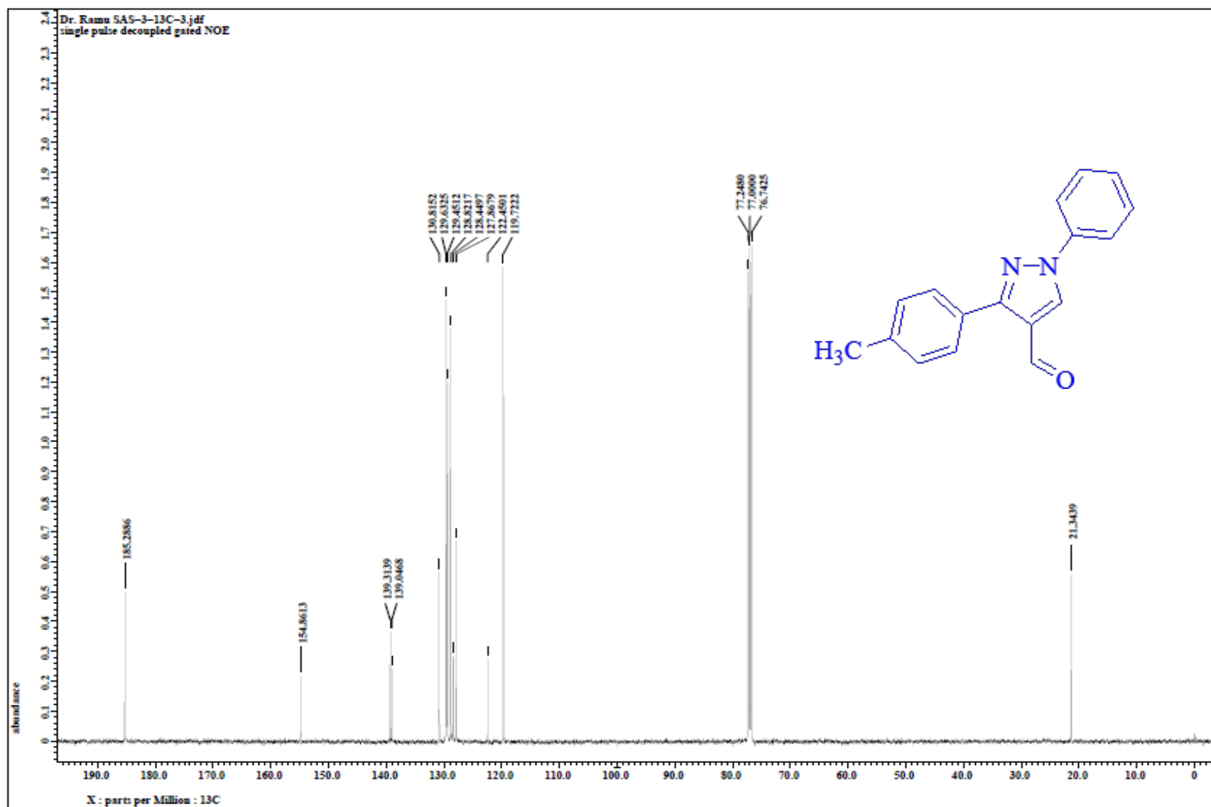
^{13}\text{C} NMR spectrum of 4c- \text{CDCl}_3 -100 MHz
