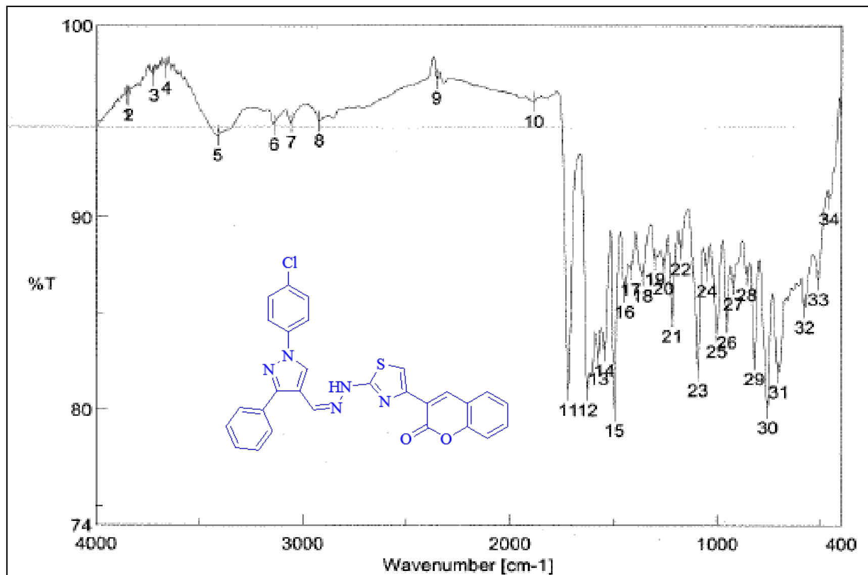
IR spectrum of 10b
