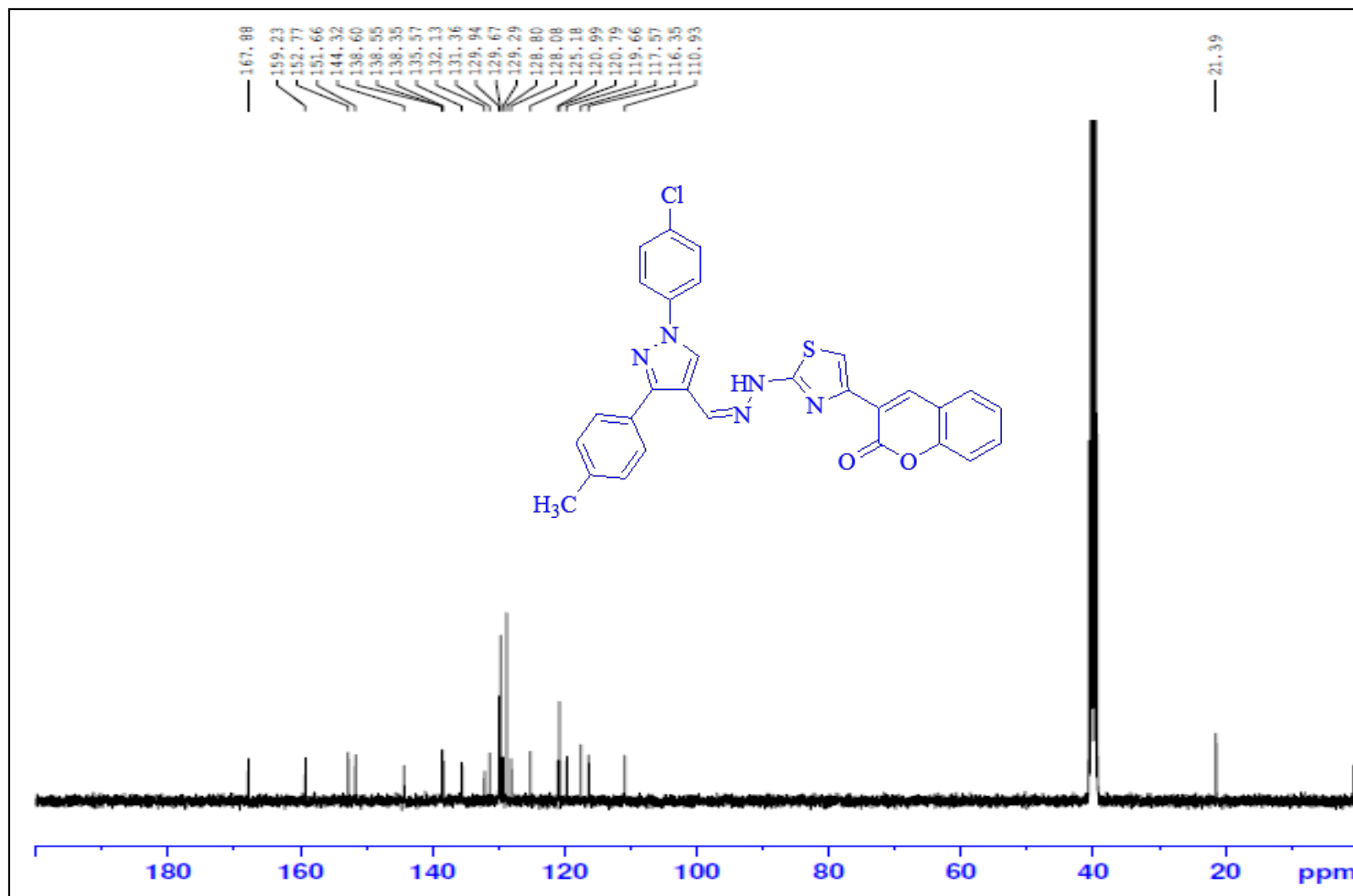
13 C NMR spectrum of 10d- DMSO-d 6 -100 MHz
