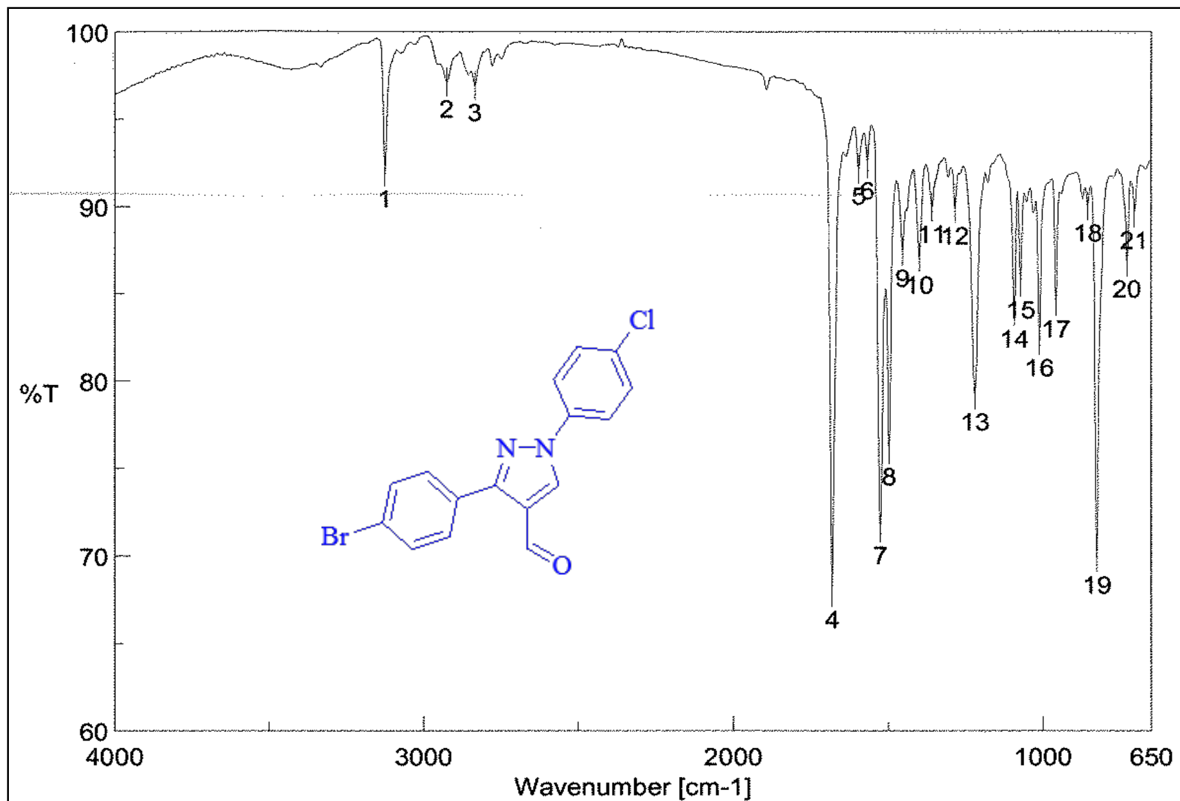
IR spectrum of 4j
