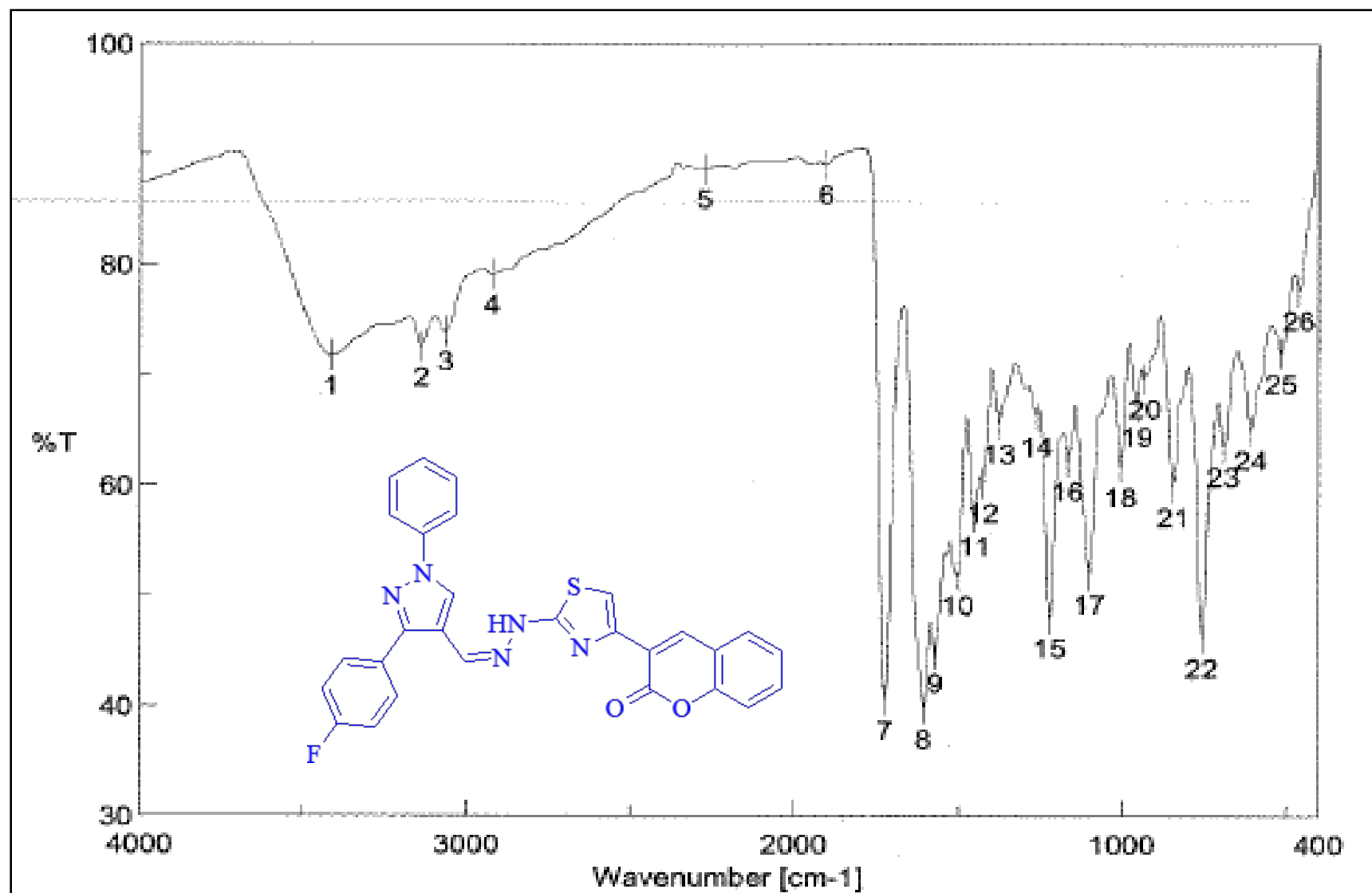
IR spectrum of 10k
