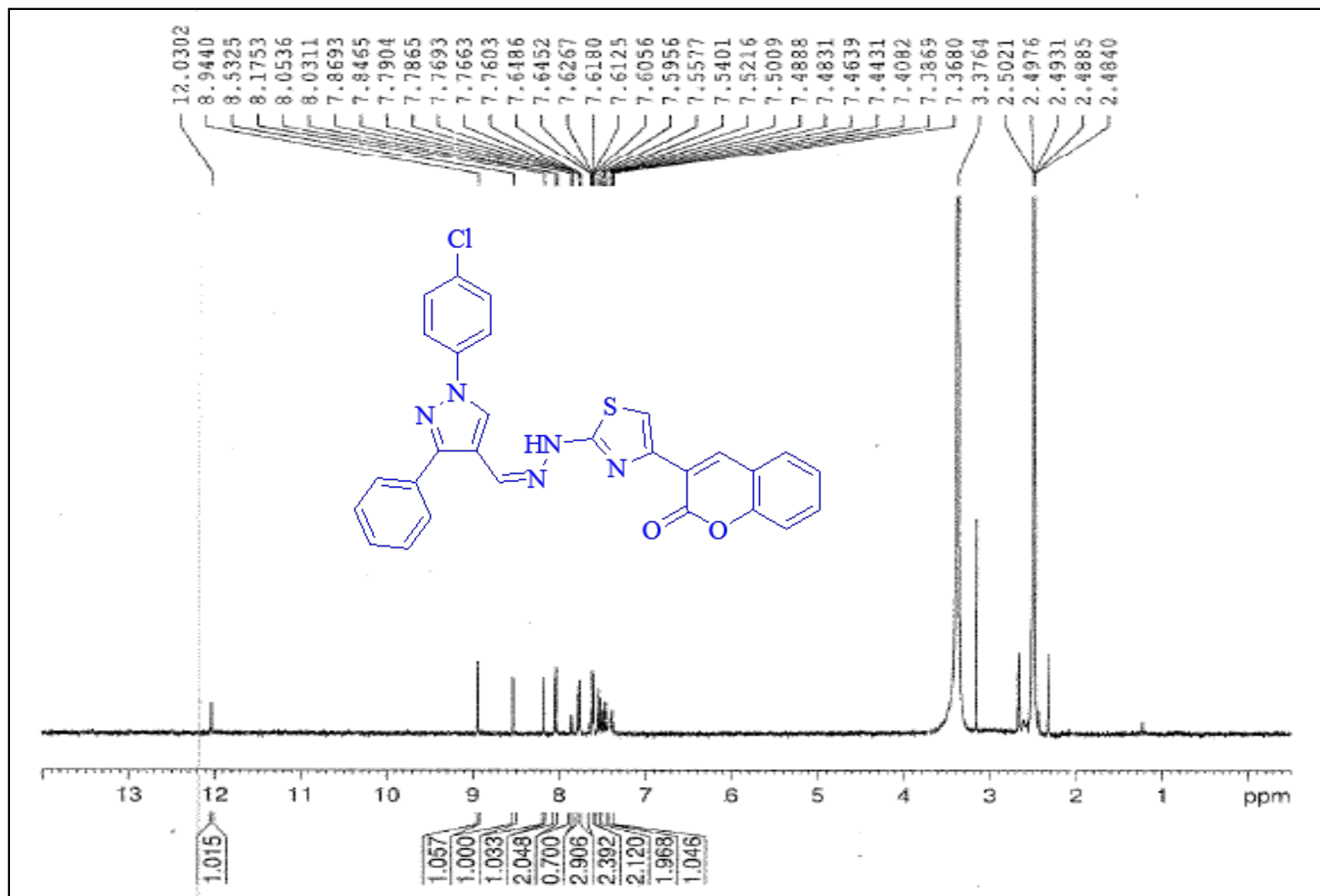
1 H NMR spectrum of 10b-DMSO-d 6 -400 MHz
