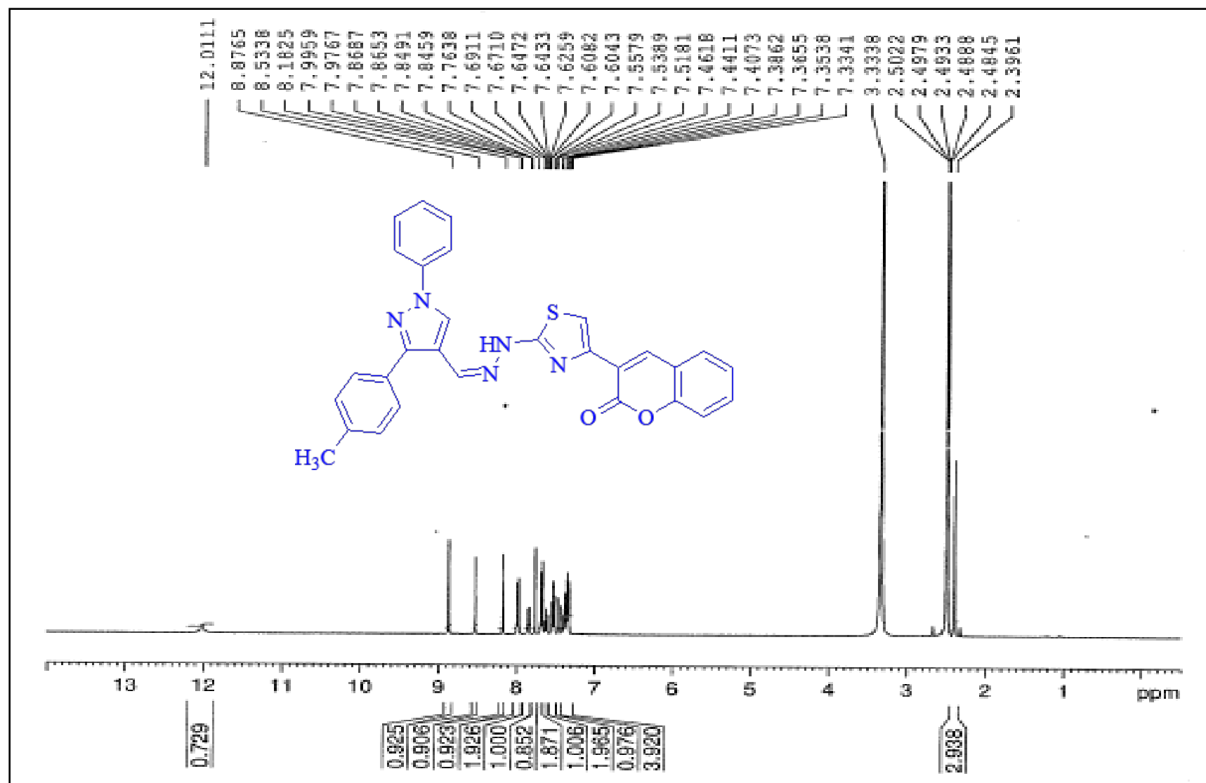
1 H NMR spectrum of 10c-DMSO-d 6 -400 MHz
