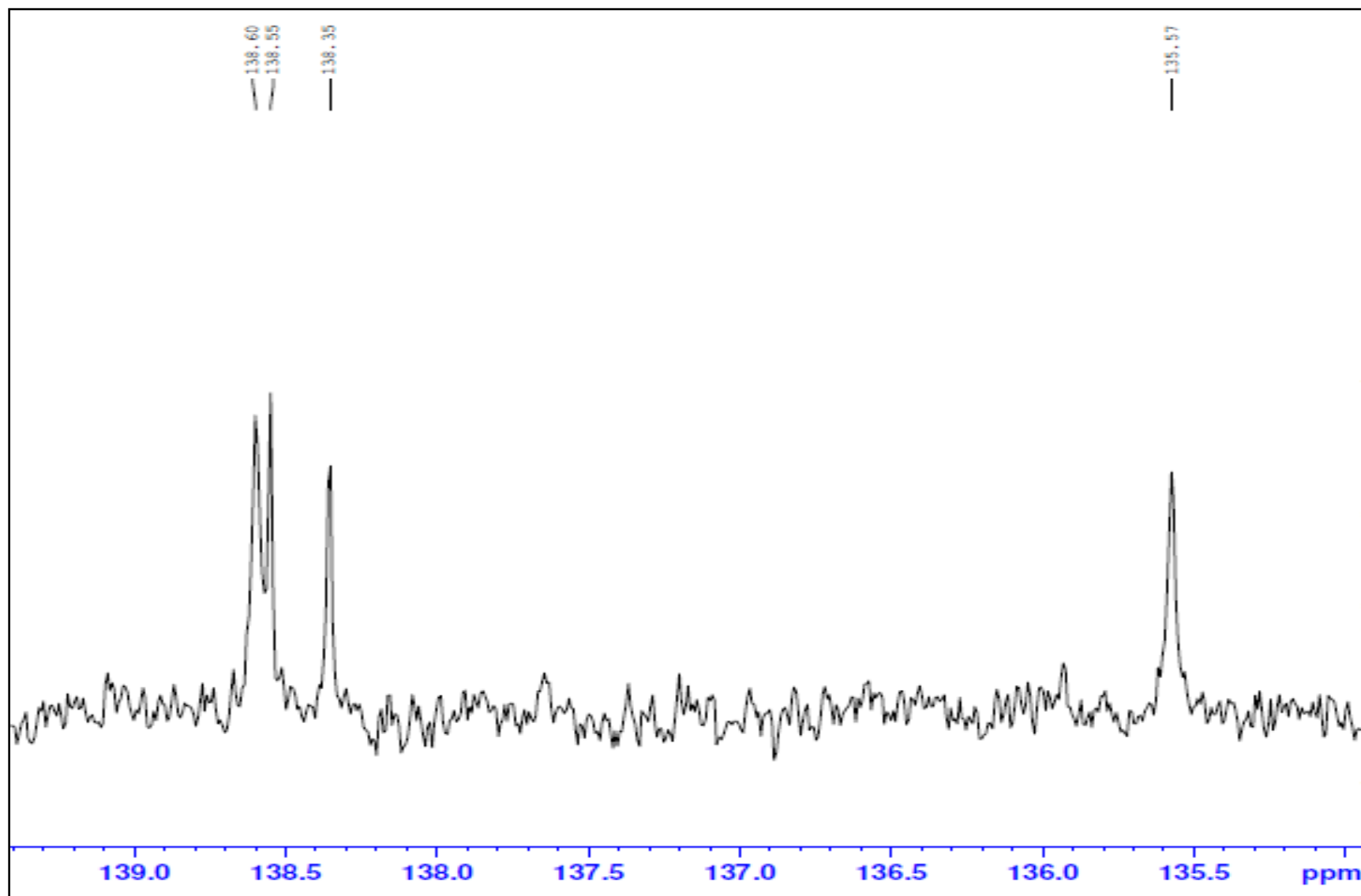
Expanded spectrum of 10d ( ^{13}\text{C} NMR)
