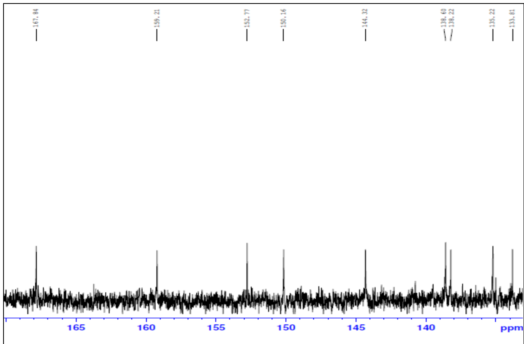
Expanded spectrum of 10h ( ^{13}\text{C} NMR)
