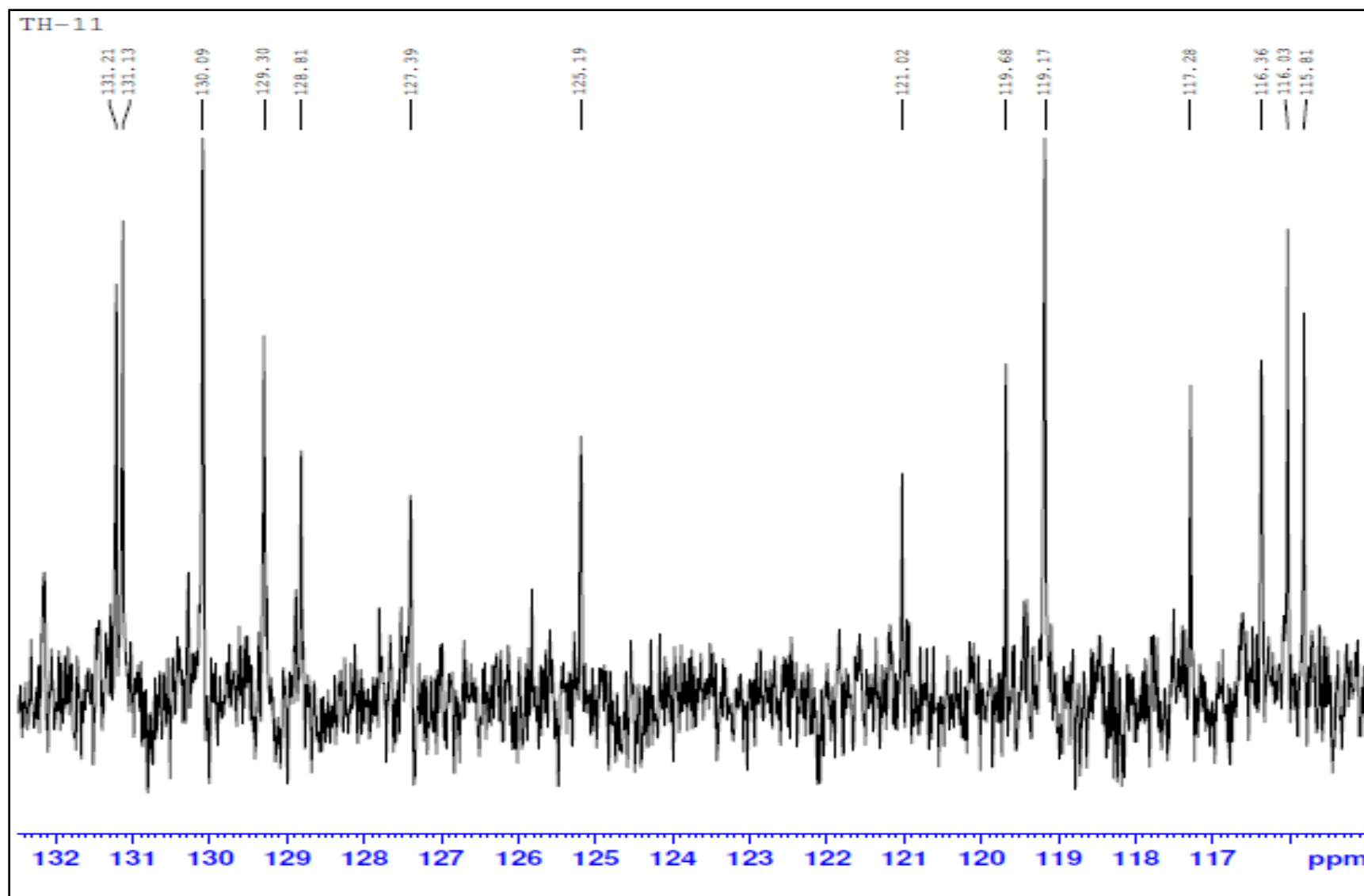
Expanded spectrum of 10k ( ^{13}\text{C} NMR)
