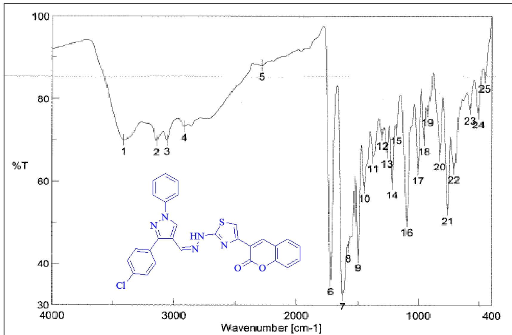
IR spectrum of 10g
