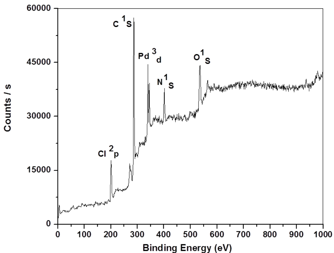
Fig. S1 Overall XPS spectrum of the Pd-PANI nanocomposite
