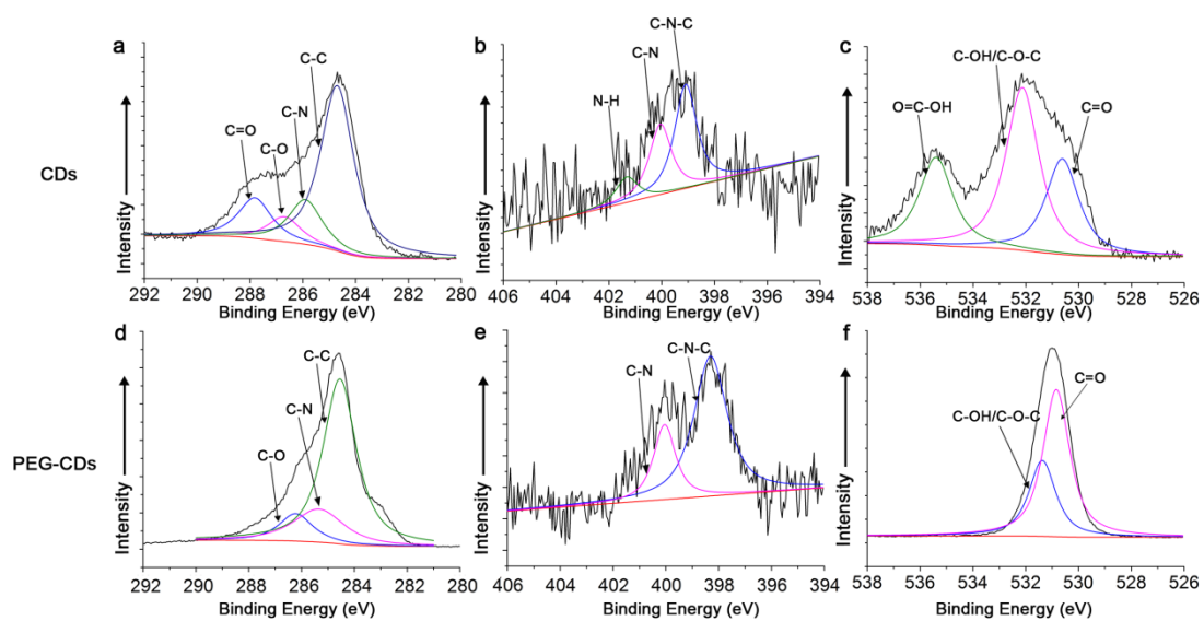
Fig. S1 High resolution XPS spectra for CDs and PEG-CDs: C_{1s} spectrum (a, d); N_{1s} spectrum (b, e); O_{1s} spectrum (c, f).
