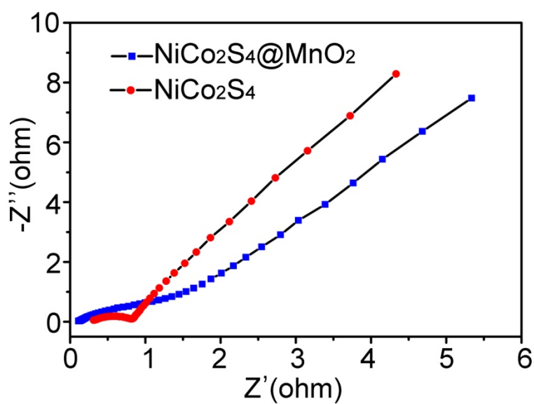
Figure S4. EIS spectra of the NiCo 2 S 4 and NiCo 2 S 4 @MnO 2 electrode.
