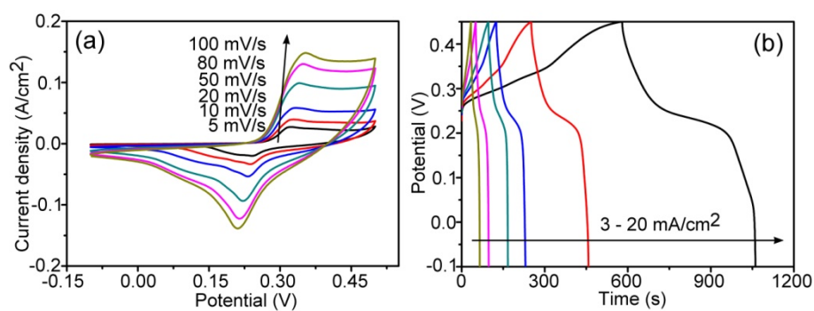
Figure S3. (a) CV curves and (b) CD curves of the NiCo 2 S 4 @MnO 2 electrode materials.
