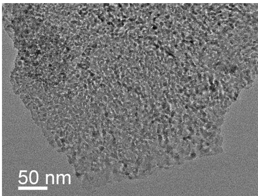
Figure S1. TEM image of NiCo 2 O 4 nanosheet.
