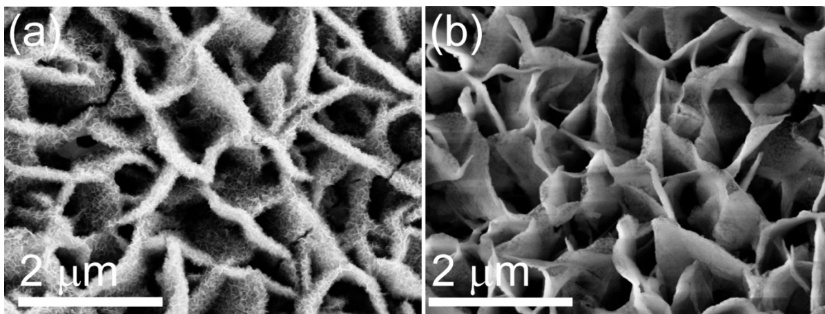
Figure S5. SEM image of the (a) \text{NiCo}_2\text{S}_4@\text{MnO}_2 and (b) \text{NiCo}_2\text{S}_4 electrode after cycling.
