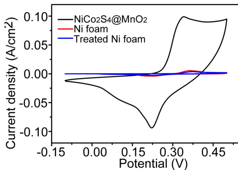
Figure S2. CV curve of NiCo 2 S 4 @MnO 2 electrode, pure and treated Ni foams electrode.
