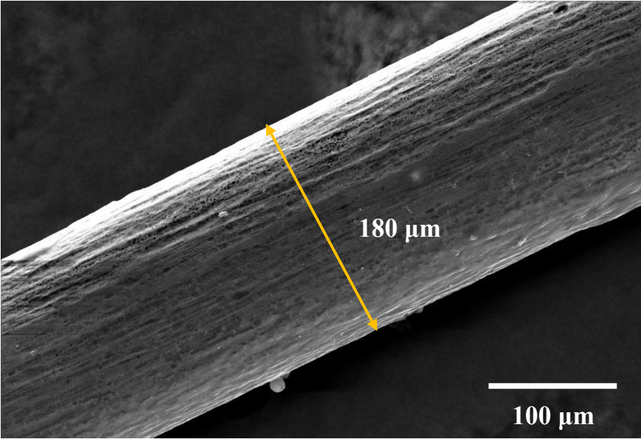
Fig. S1. The scanning electron micrograph of stainless steel wire after corrosion process.
