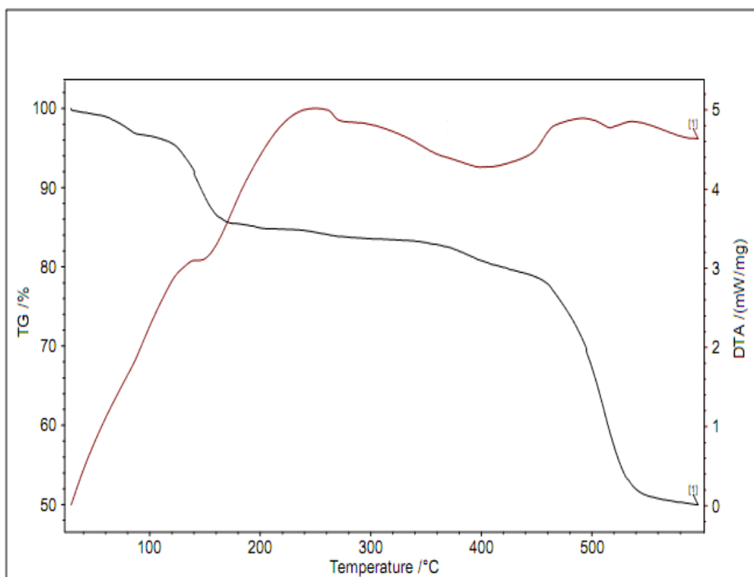
Fig S2. Thermogram of PLHP
