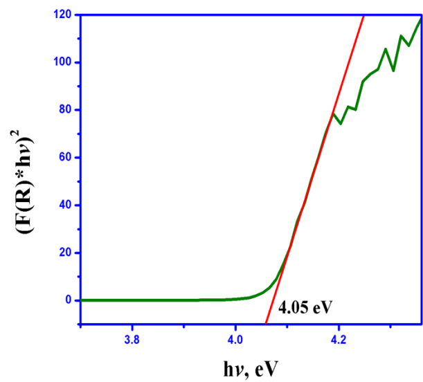
Fig S4. Tauc plot (Direct Band gap energy curve)
