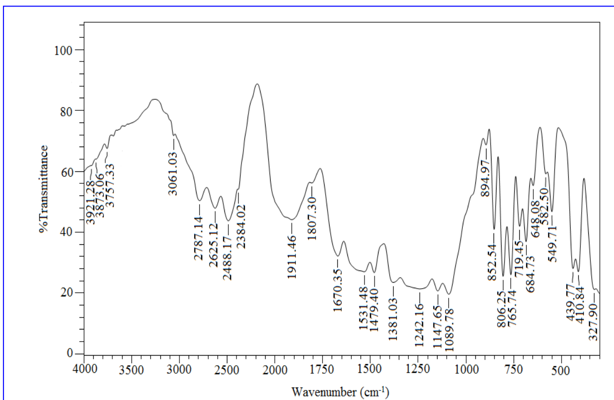
Fig S1. FT-IR spectrum of mixed crystal PLHP
