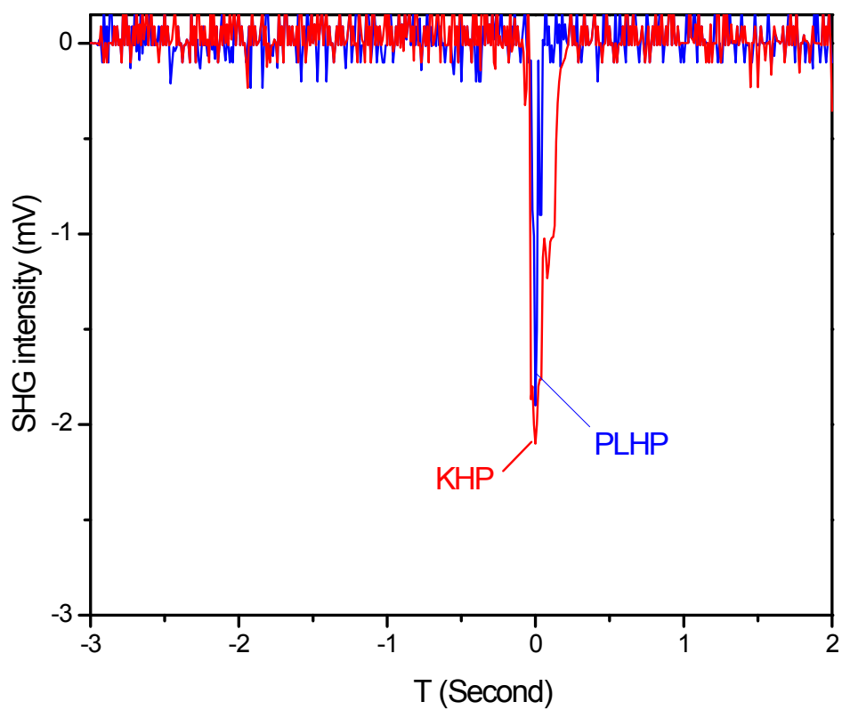
Fig S4. The comparative SHG oscilloscope traces of the powder samples KHP (red) and PLHP (blue)
