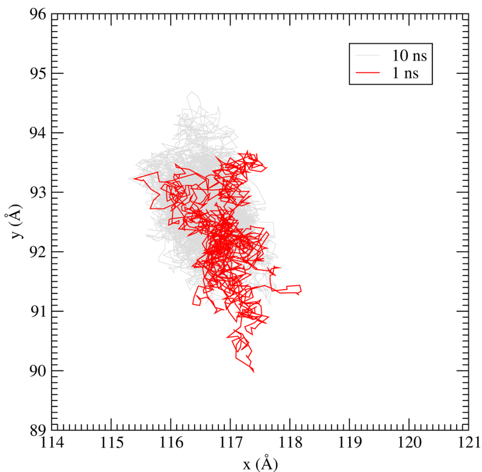
Fig.15 Trajectories across xy of the centre-of-mass coordinates of COL in TU obtained from the molecular dynamics run (1ns, in red and superimposed up to 10 ns, in gray).
