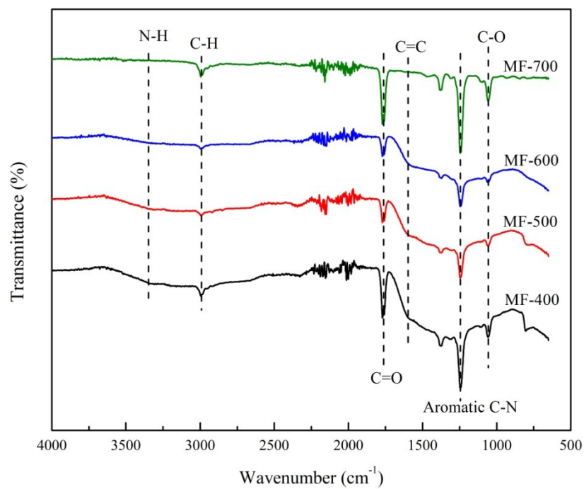
Fig. S5 FTIR spectra of prepared carbon materials.
