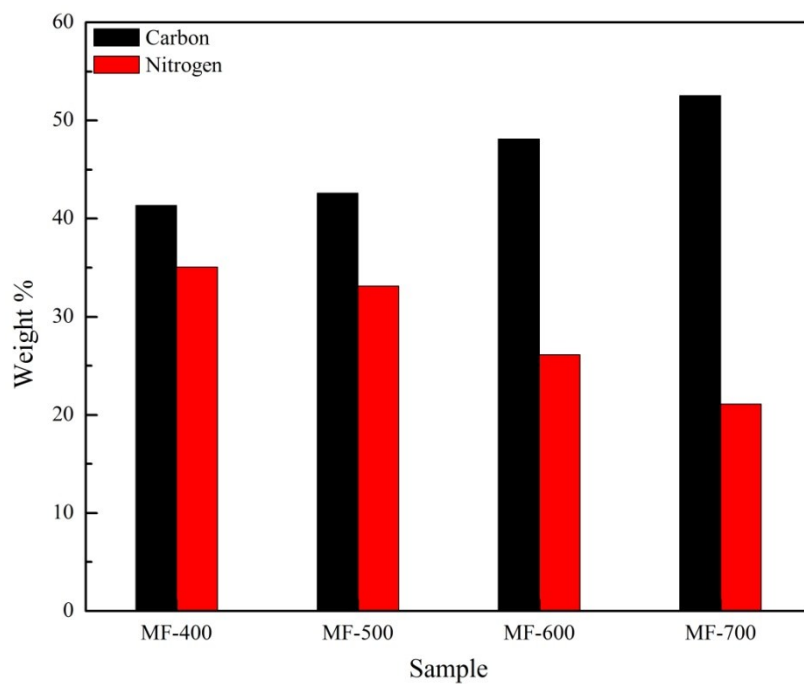
Fig. S4 Elemental composition of the mesoporous carbons.
