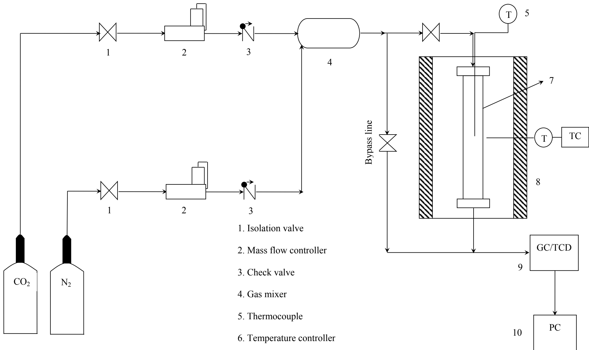
Fig. S1 Schematic diagram of the adsorption-desorption setup.
