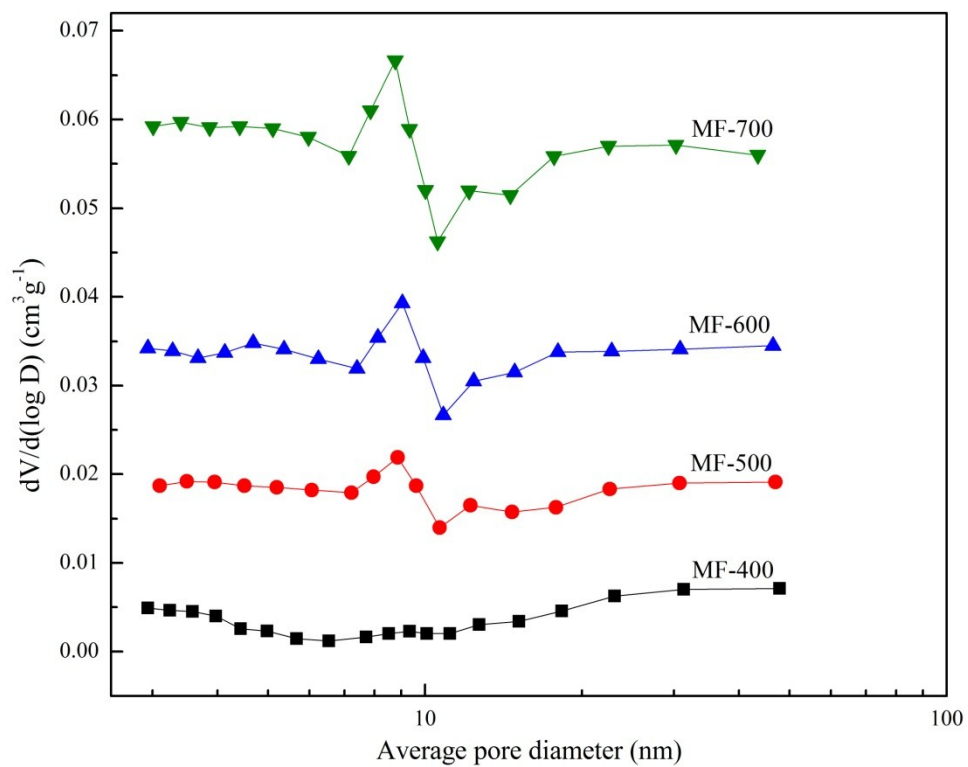
Fig. S3 Pore size distribution of prepared carbons.
