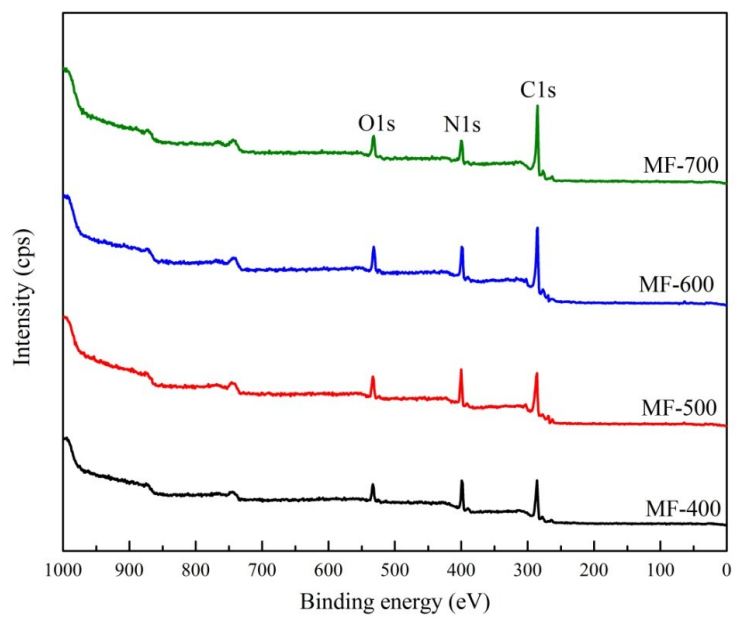
Fig. S6 XPS survey scan spectra of prepared mesoporous carbons.
