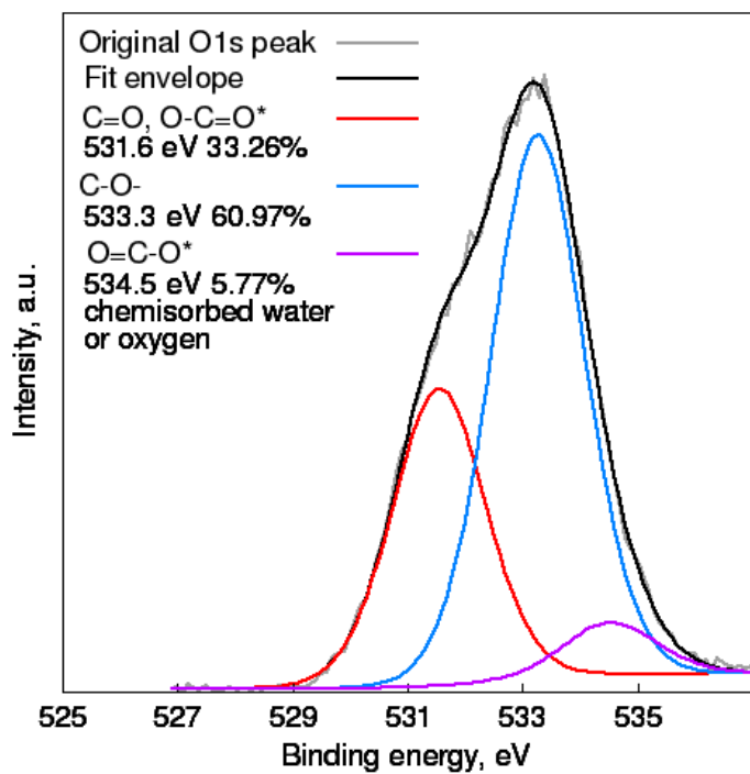
Fig. S2. O1s XPS spectra of CH
