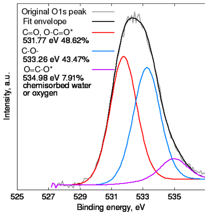
Fig. S3. O1s XPS spectra of CH-mel
