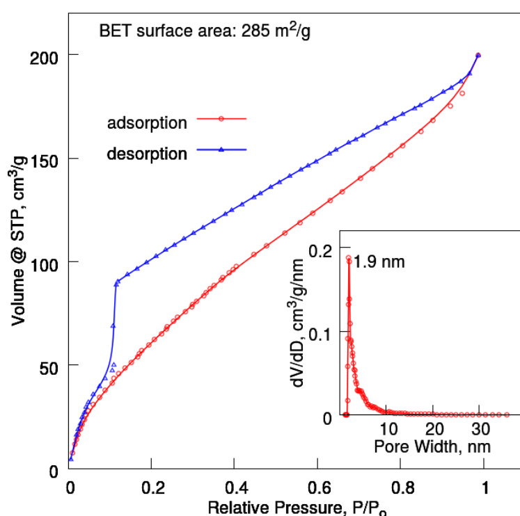
Fig. S1. Nitrogen sorption isotherms and pore size distribution (inset) of CH-mel.
