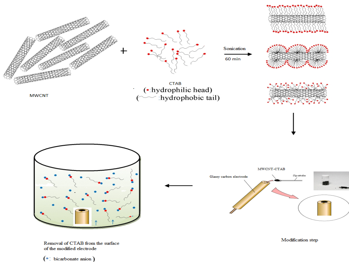
Supplementary Fig. S1. Schematic diagram of the proposed modification steps.
