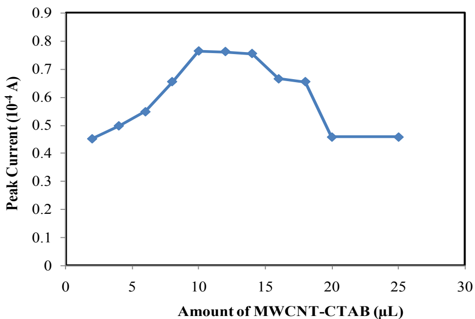
Supplementary Fig. S2. Effect of amount of MWCNT-CTAB suspension on response current of the sensor for 1.0 mM PCM.
