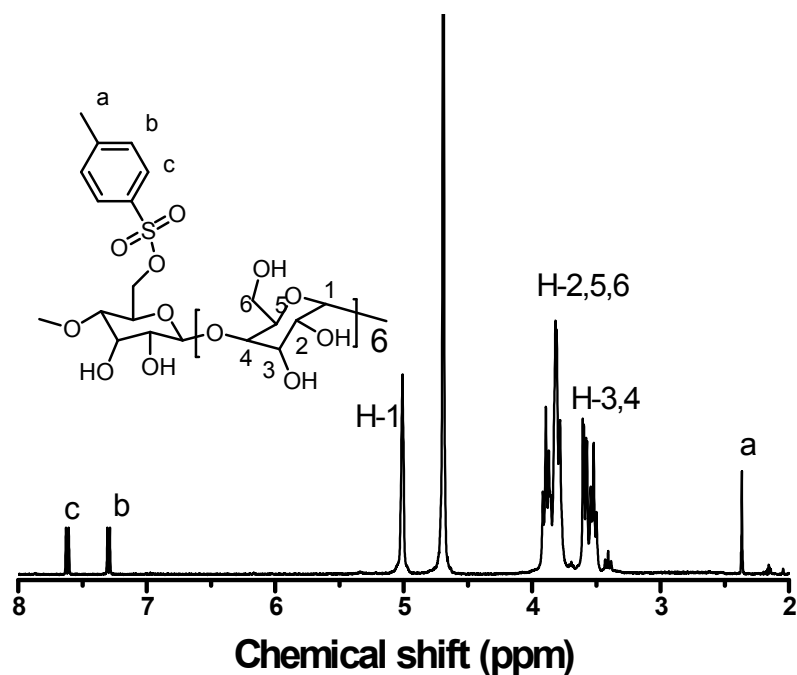
Fig. S1. ^1\text{H} NMR spectrum of 6-mono-TsCD.
