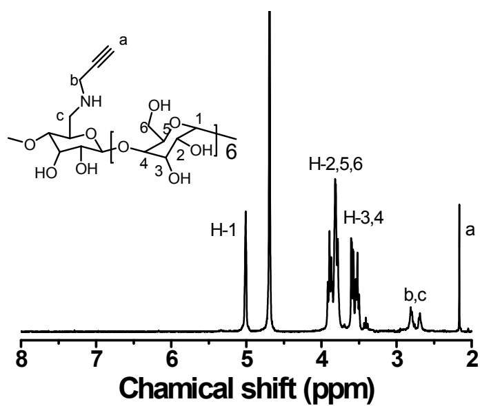
Fig. S3. ^1\text{H} NMR spectrum of 6-mono-alkyne-CD.
