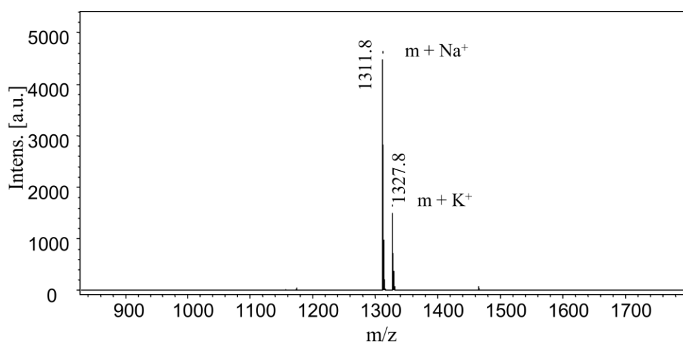
Fig. S2. MALDI-TOF MS of 6-mono-TsCD.
