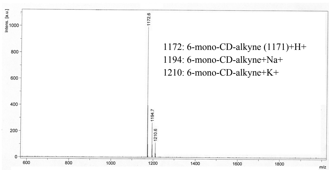
Fig. S4. MALDI-TOF MS of 6-mono-alkyne-CD.
