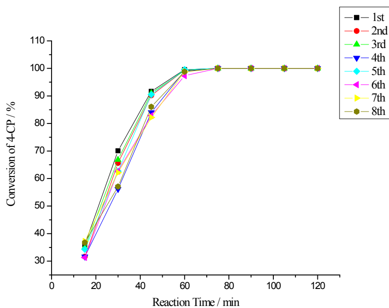
Fig. 9 The influence of reuse times of catalysts on the conversion of 4-CP
