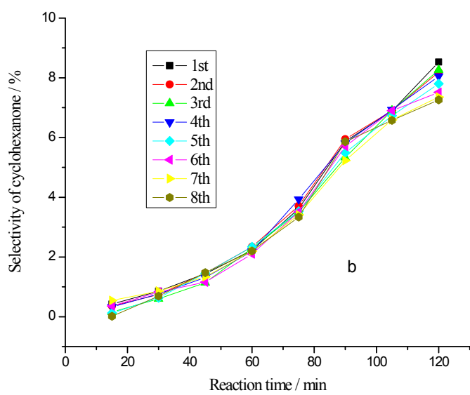
Fig. 10 The influence of reuse times of catalysts on the hydrogenation products
